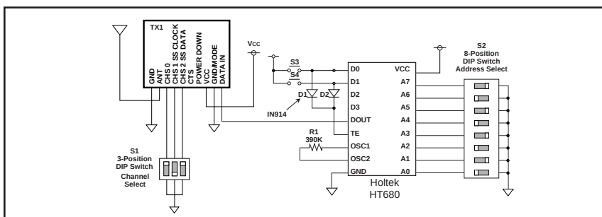
Figure 23: Typical Application: Remote-Control Transmitter
