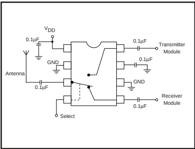
Figure 28: Typical Antenna Switch
