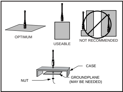
Figure 25: Antenna Orientations
