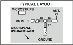
Figure 17: T-pad Layout
