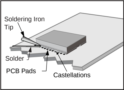
Figure 12: Soldering Technique
