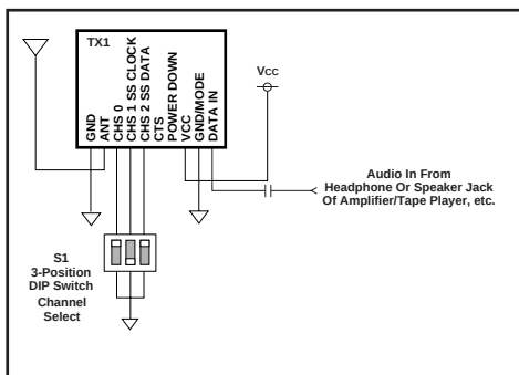
Figure 22: Typical Voice Transmitter
