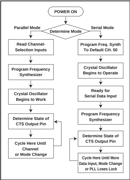
Figure 19: Start-up Sequence
