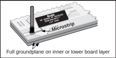
Figure 15: Groundplane Treatment
