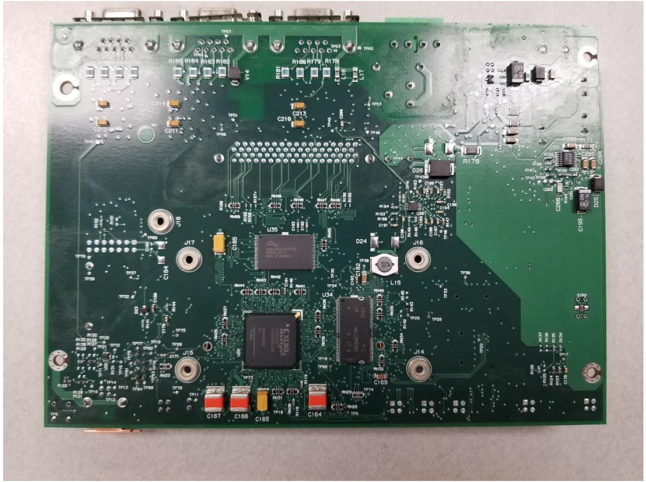
Figure 5: MAIN BOARD BOTTOM
