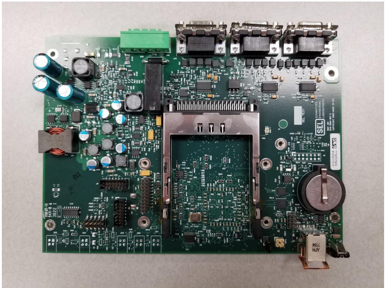
Figure 6: MAIN BOARD TOP
