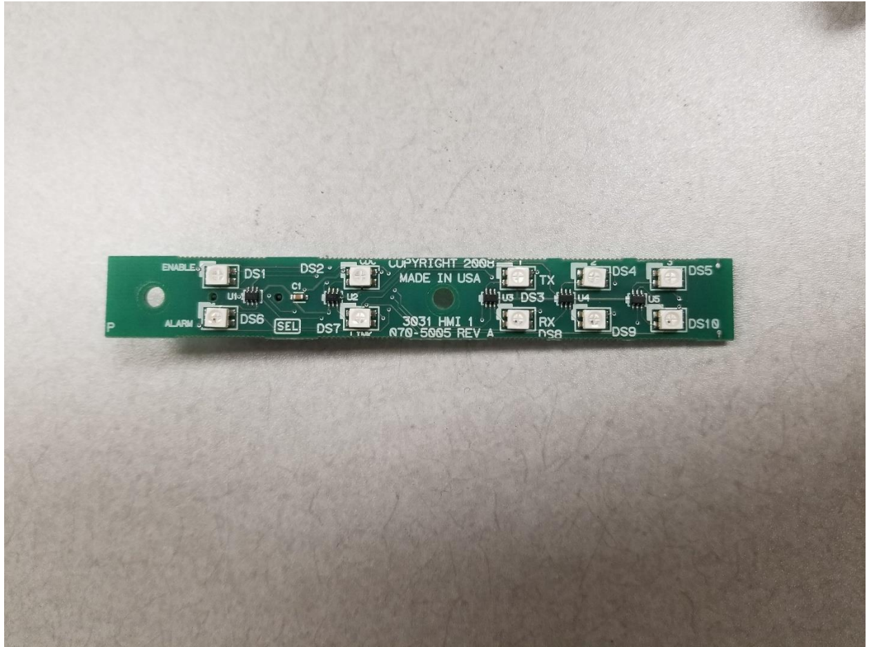
Figure 4: HMI BOARD TOP
