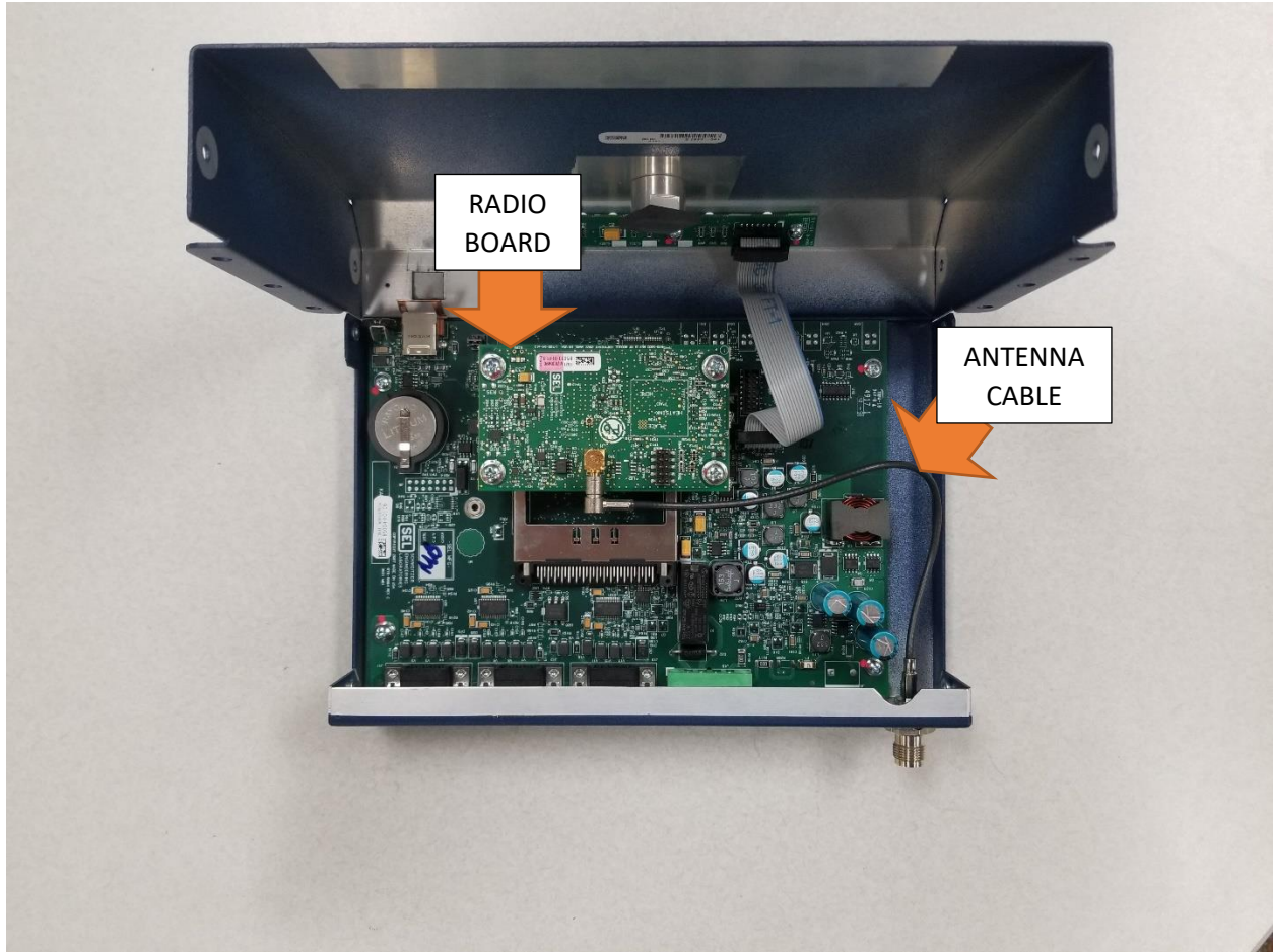
Figure 1: INTERNAL BOARD SETUP
