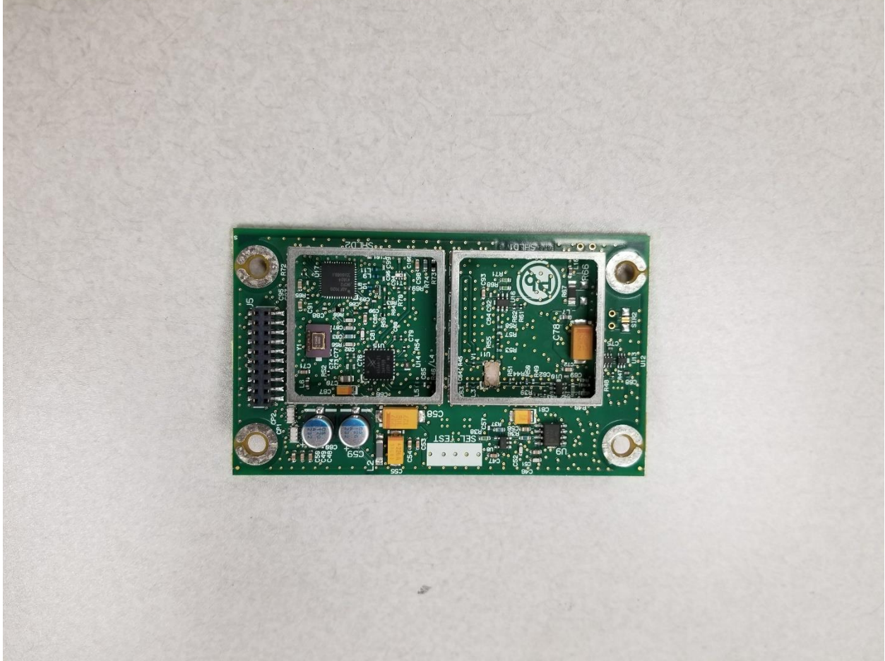
Figure 7: RADIO BOARD BOTTOM - UNSHIELDED
