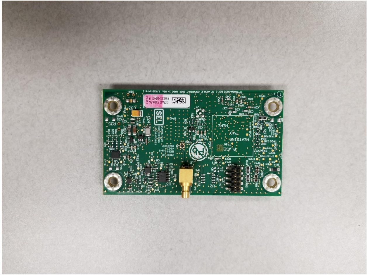
Figure 9: RADIO BOARD TOP
