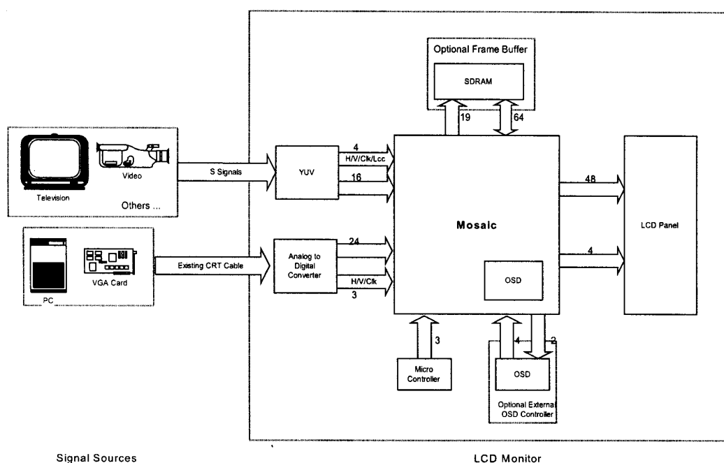
Reference Design with Vitesse II and Mascot II LCD Monitor Controller
