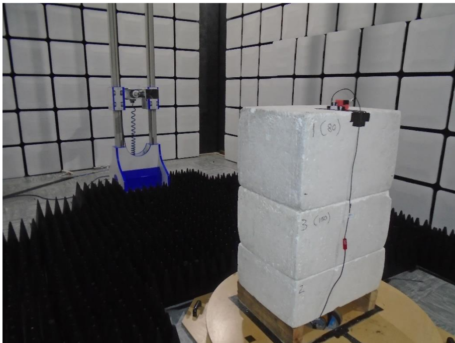
Figure 2 – Radiated Disturbance - 1 GHz to 18 GHz
