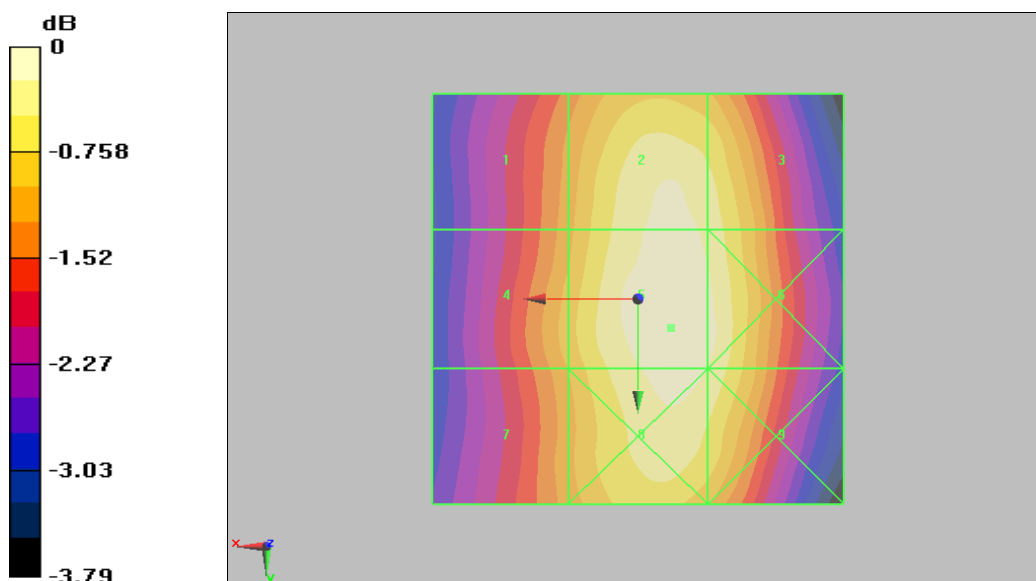
Figure 14 HAC RF E-Field CDMA Cellular Channel 1013
