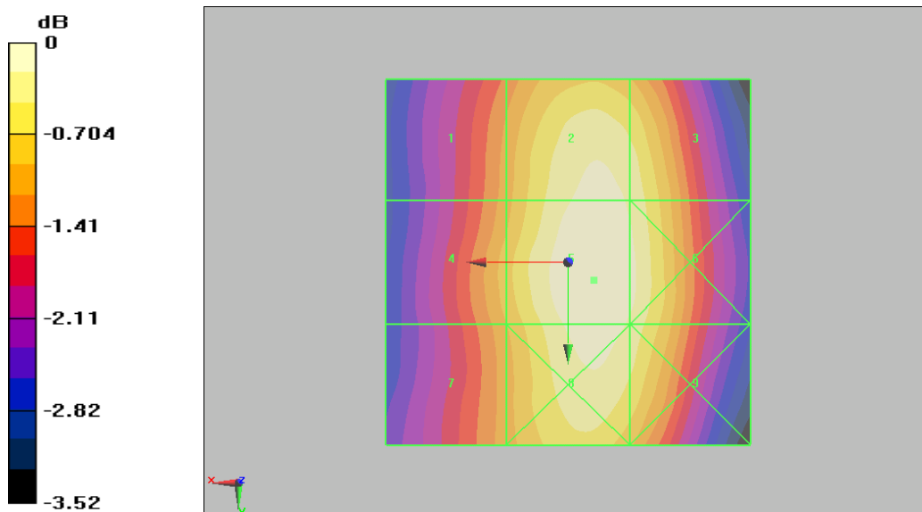
Figure 13 HAC RF E-Field CDMA Cellular Channel 384
