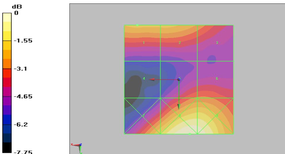
Figure 24 HAC RF E-Field CDMA AWS Channel 850
