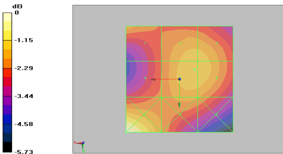
Figure 27 HAC RF H-Field CDMA AWS Channel 850
