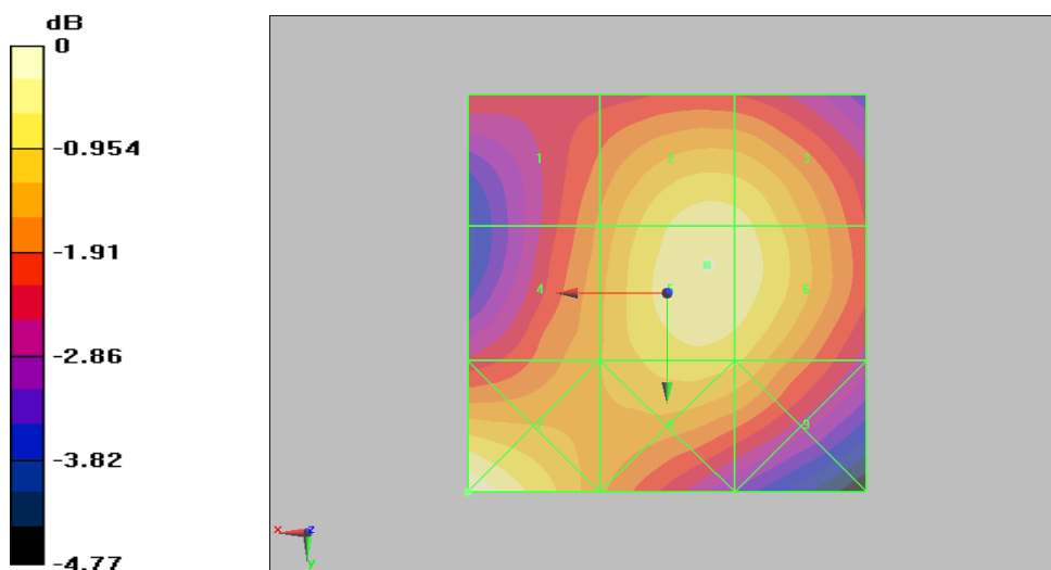
Figure 29 HAC RF H-Field CDMA AWS Channel 25
