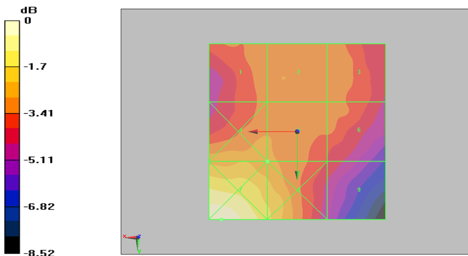
Figure 21 HAC RF H-Field CDMA PCS Channel 1175
