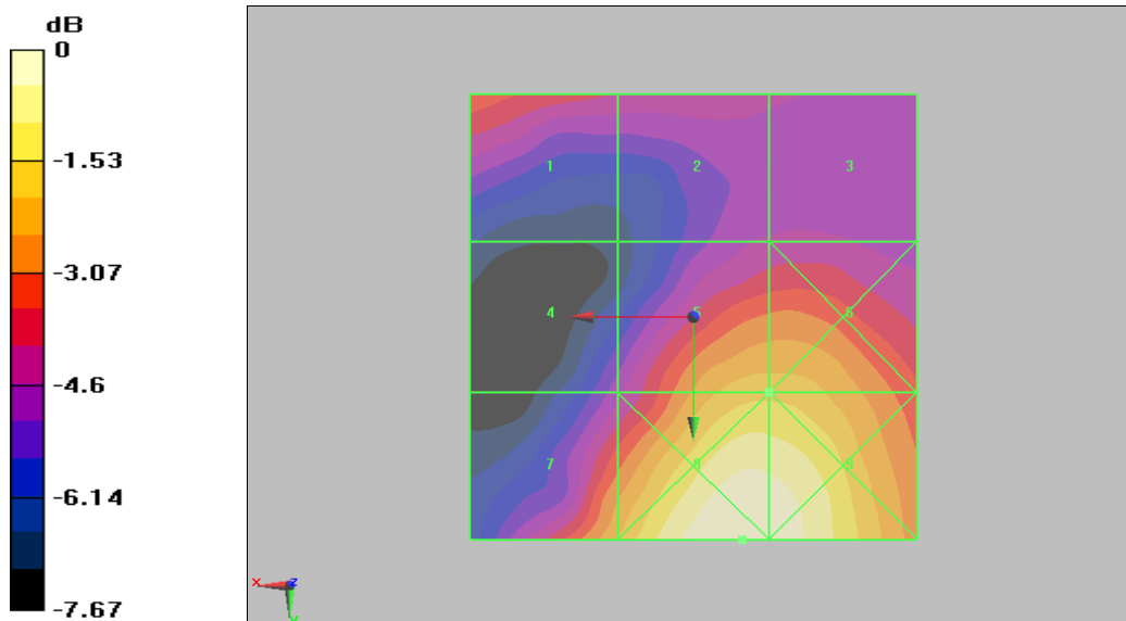
Figure 19 HAC RF E-Field CDMA PCS Channel 600
