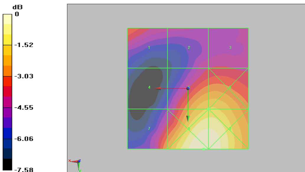
Figure 18 HAC RF E-Field CDMA PCS Channel 1175
