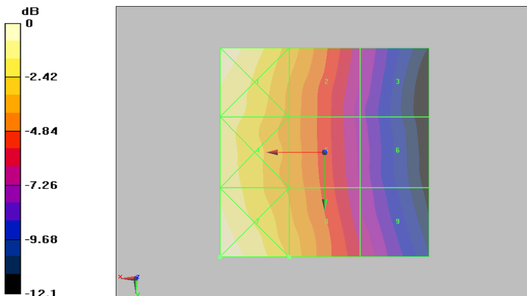
Figure 17 HAC RF H-Field CDMA Cellular Channel 1013
