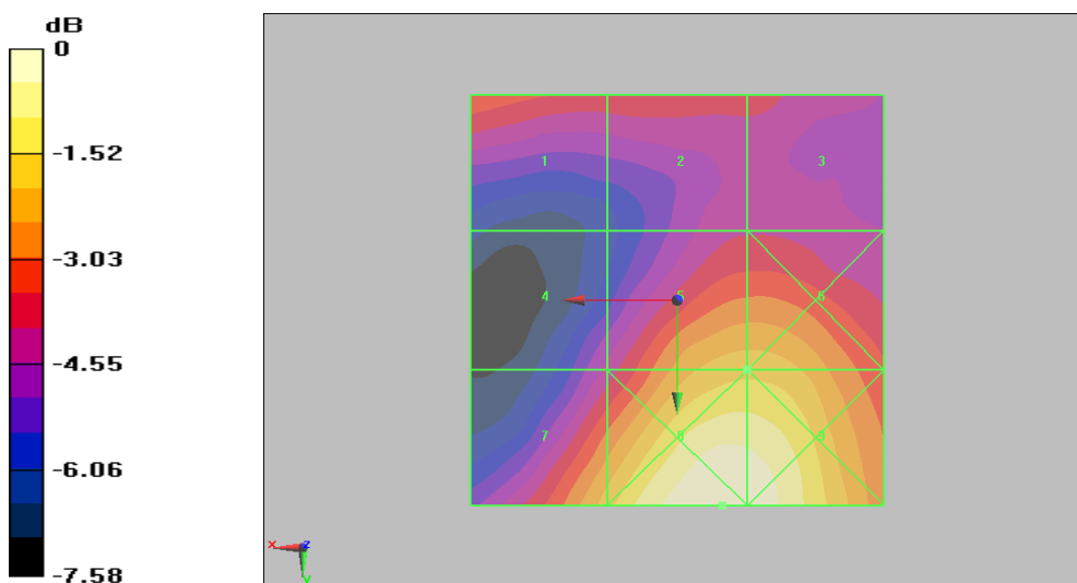
Figure 20 HAC RF E-Field CDMA PCS Channel 25
