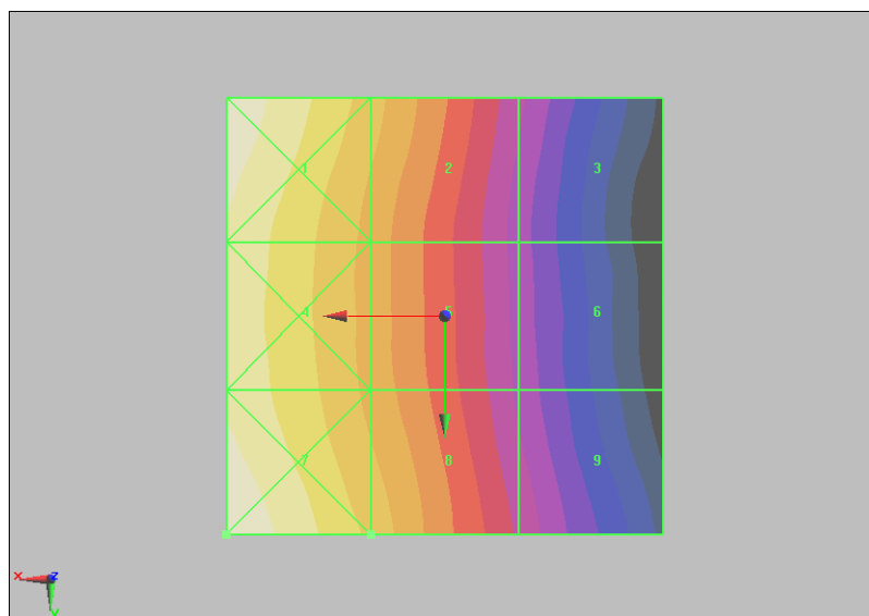
Figure 15 HAC RF H-Field CDMA Cellular Channel 777
