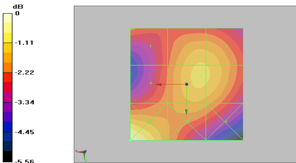
Figure 28 HAC RF H-Field CDMA AWS Channel 450
