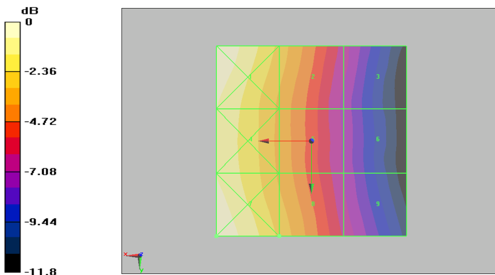
Figure 16 HAC RF H-Field CDMA Cellular Channel 384
