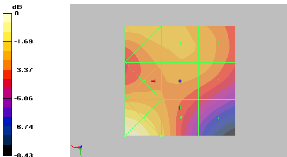
Figure 23 HAC RF H-Field CDMA PCS Channel 25
