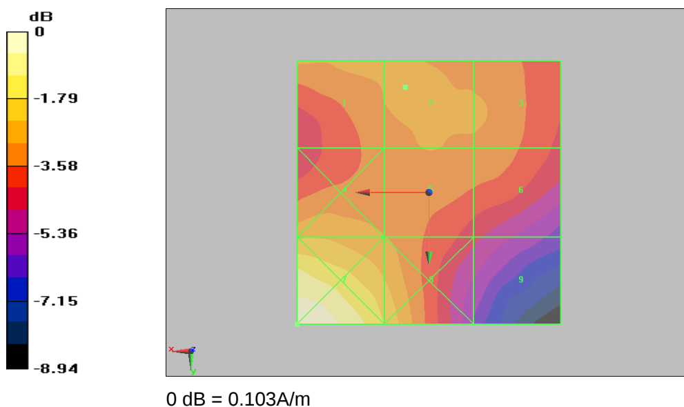
Figure 22 HAC RF H-Field CDMA PCS Channel 600
