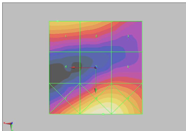
Figure 26 HAC RF E-Field CDMA AWS Channel 25
