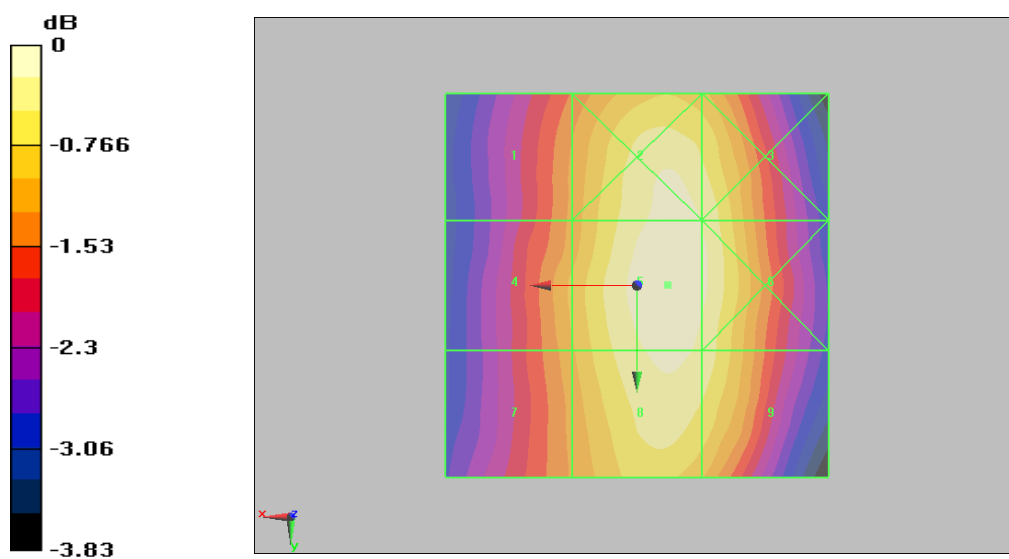
Figure 12 HAC RF E-Field CDMA Cellular Channel 777
