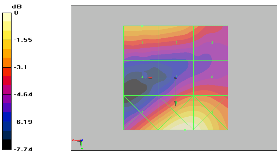
Figure 25 HAC RF E-Field CDMA AWS Channel 450
