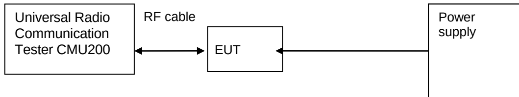
Figure 3. Test Set-up
