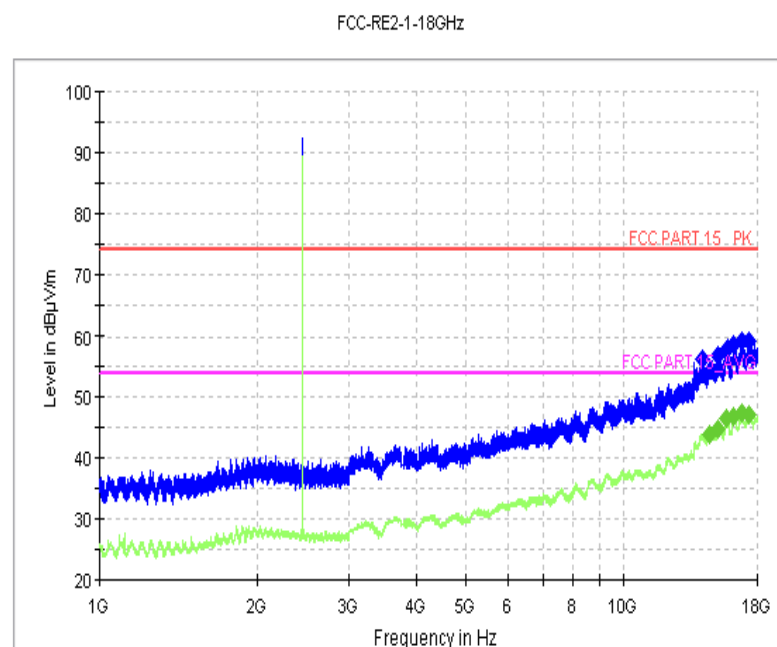
Fig.4 Radiated Spurious Emission (GFSK, Ch39, 1 GHz-18GHz)
