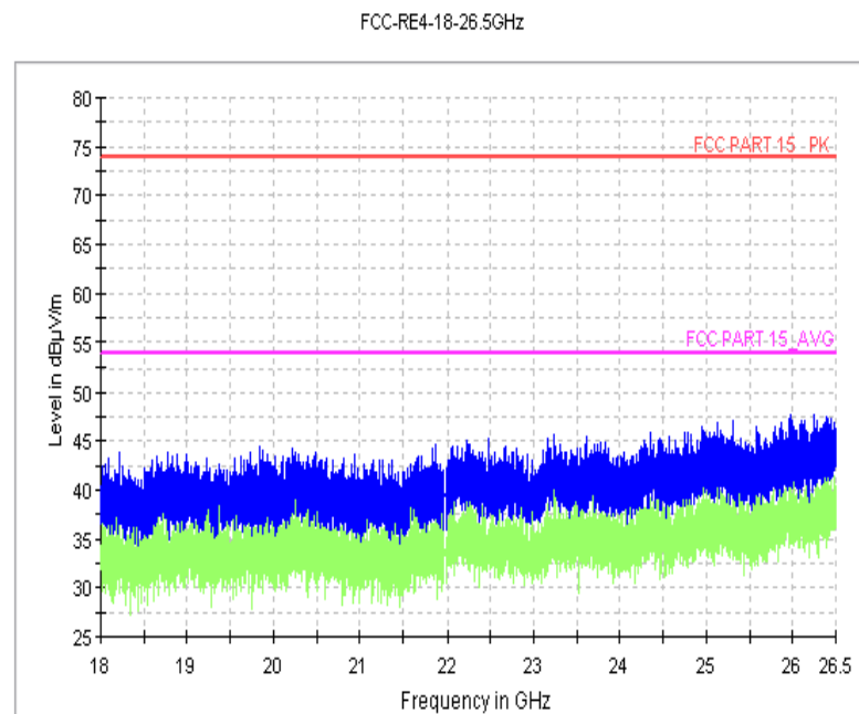
Fig.5 Radiated Spurious Emission (GFSK, Ch39, 18 GHz-26.5GHz)
