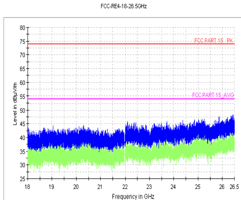
Fig.12 Radiated Spurious Emission ( \pi/4 DQPSK, Ch39, 18 GHz-26.5GHz)
