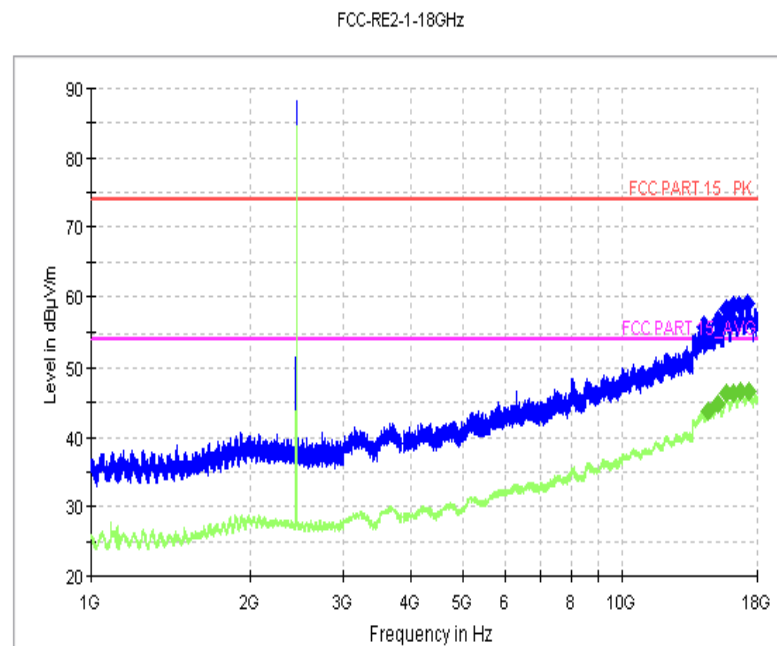
Fig.19 Radiated Spurious Emission (8DPSK, Ch39, 1 GHz-18GHz)
