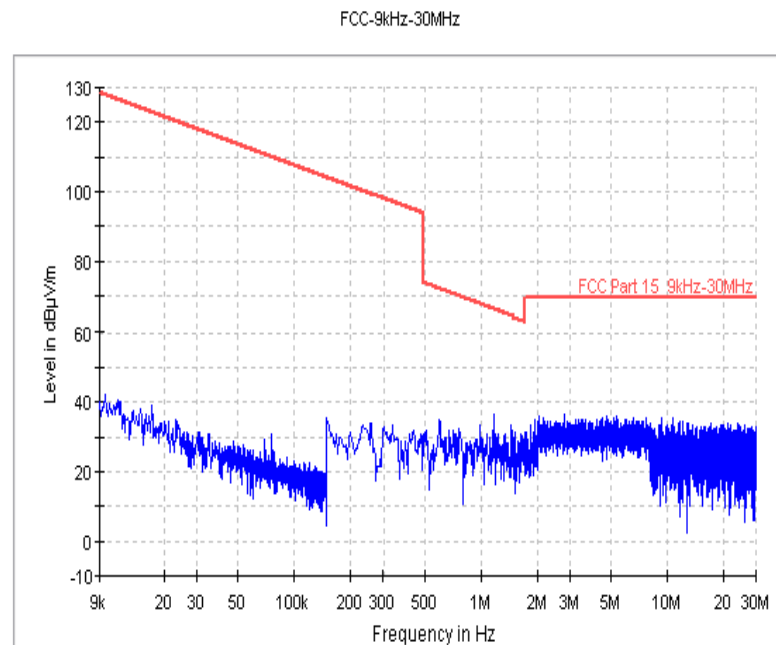
Fig.2 Radiated Spurious Emission (GFSK, Ch39, 9 kHz-30MHz)
