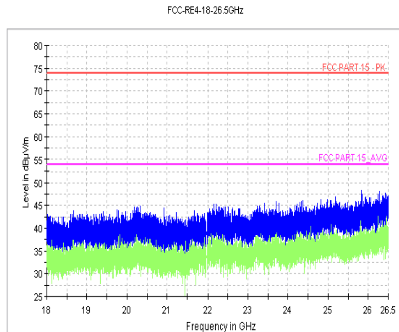
Fig.20 Radiated Spurious Emission (8DPSK, Ch39, 18 GHz-26.5GHz)
