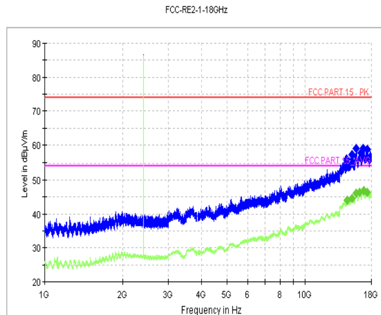
Fig.9 Radiated Spurious Emission ( \pi/4 DQPSK, Ch0, 1 GHz-18GHz)
