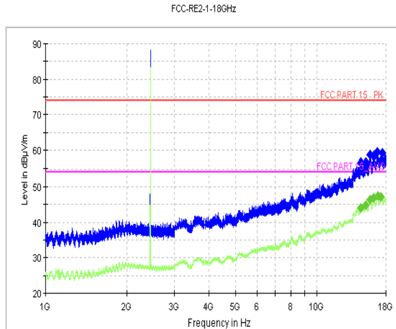
Fig.11 Radiated Spurious Emission ( \pi/4 DQPSK, Ch39, 1 GHz-18GHz)
