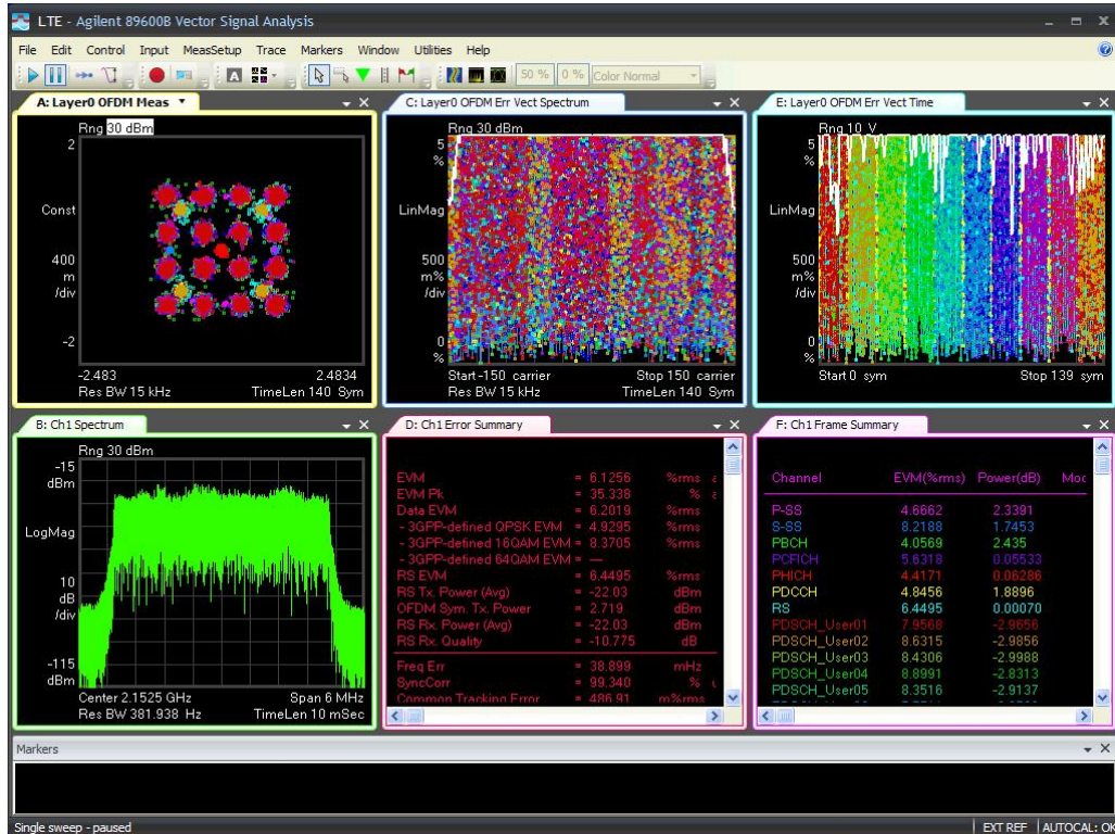
5M-Port 2 -2152.5MHz-TM3.3
