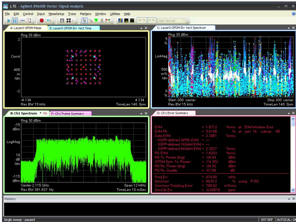
10M-Port 2 -2115MHz-TM3.1
