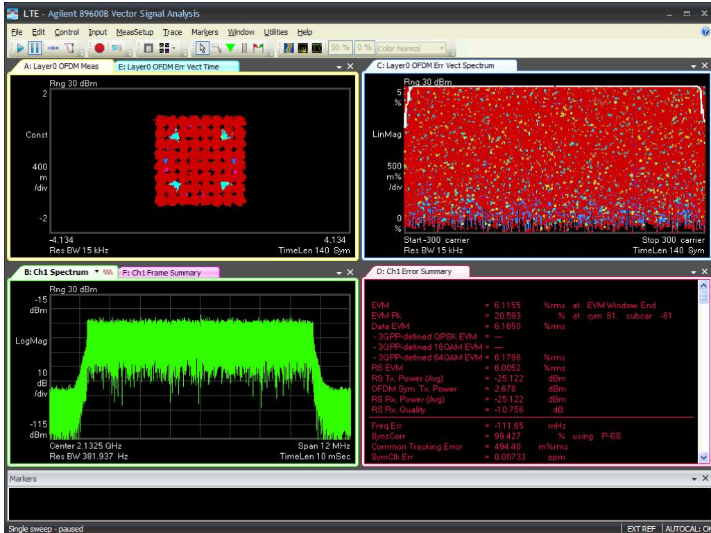
10M-Port 2 -2132.5MHz-TM3.2
