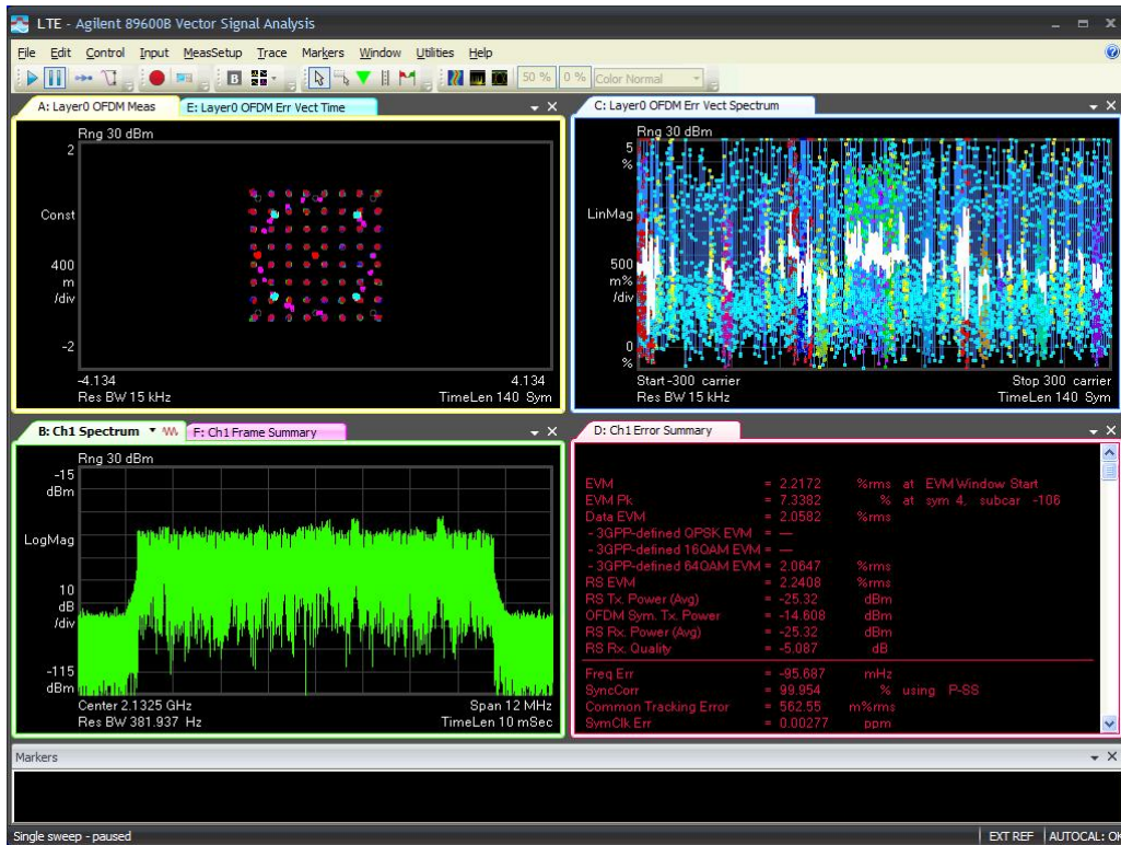
10M-Port 2 -2132.5MHz-TM3.1
