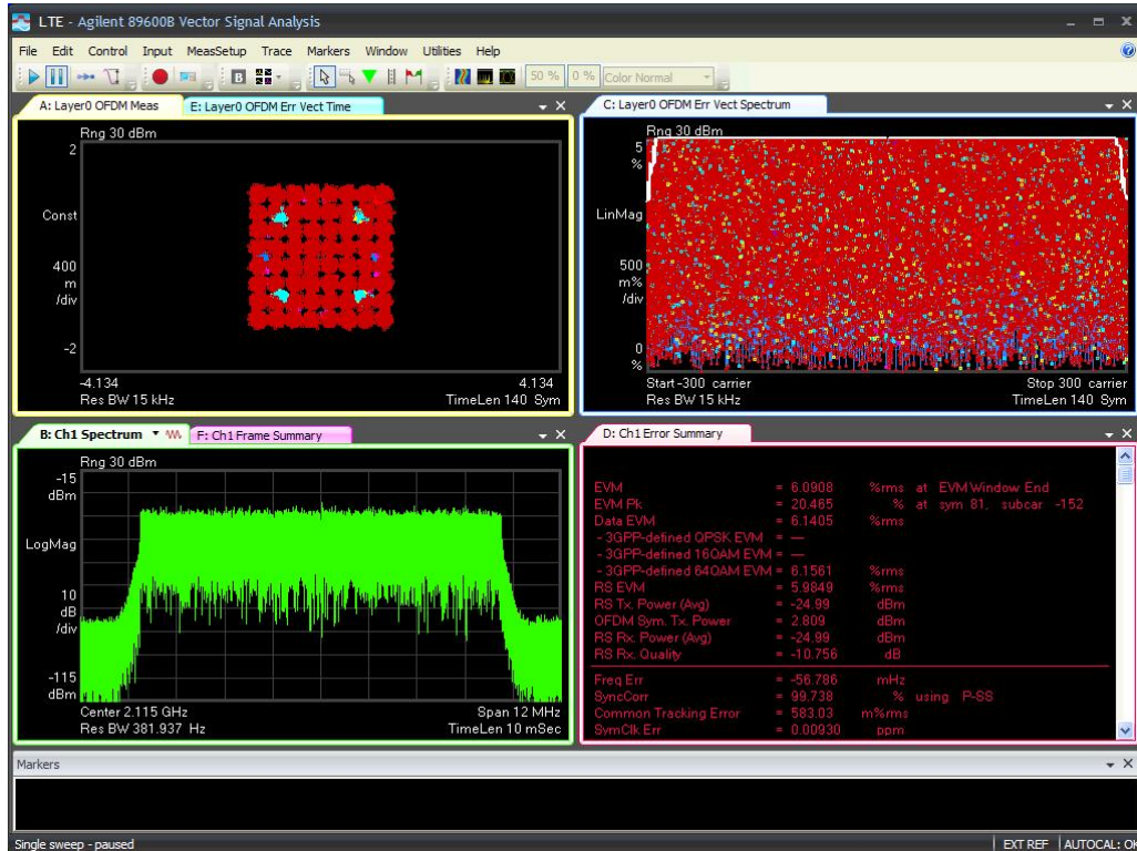
10M-Port 2 -2115MHz-TM3.2
