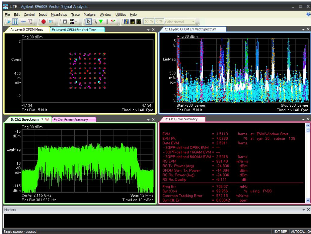
10M-Port 1 -2115MHz-TM3.1
