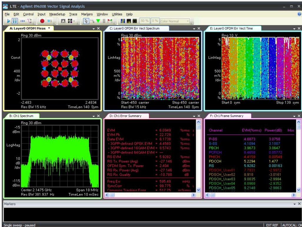
15M-Port 1 -2147.5MHz-TM3.3
