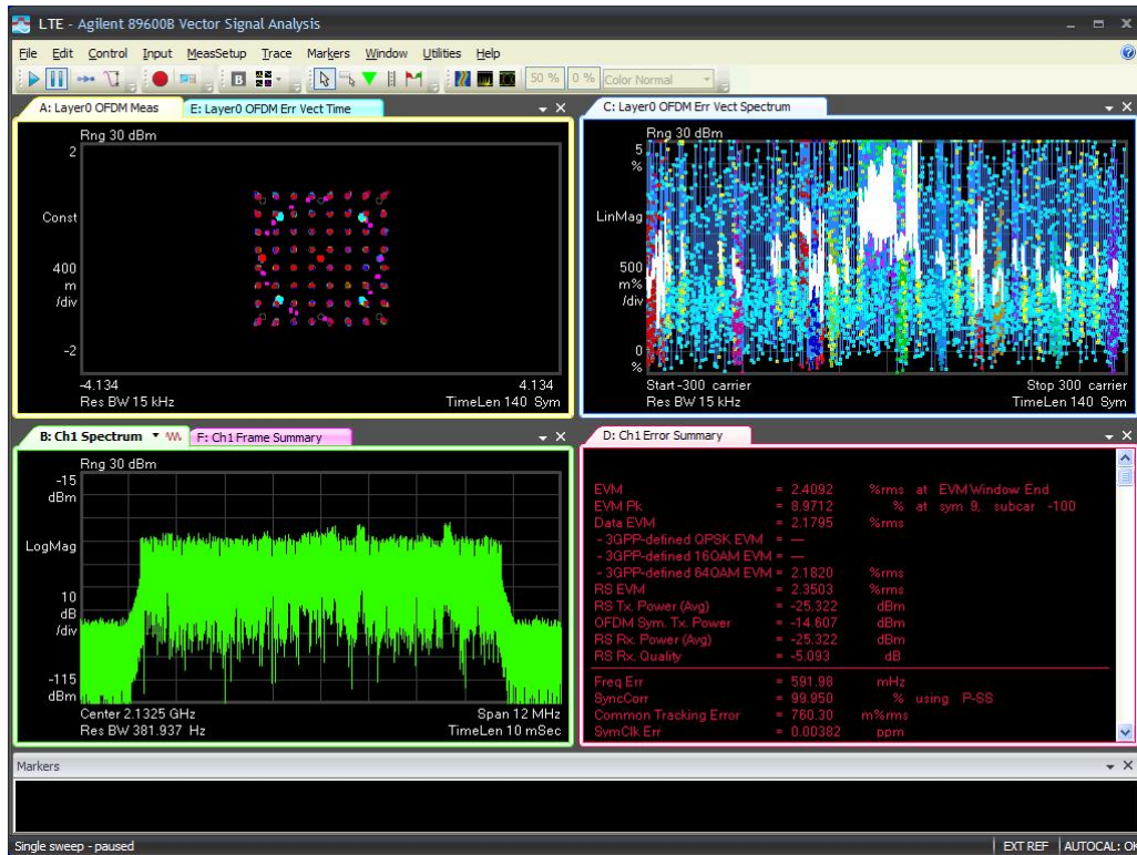
10M-Port 1 -2132.5MHz-TM3.1
