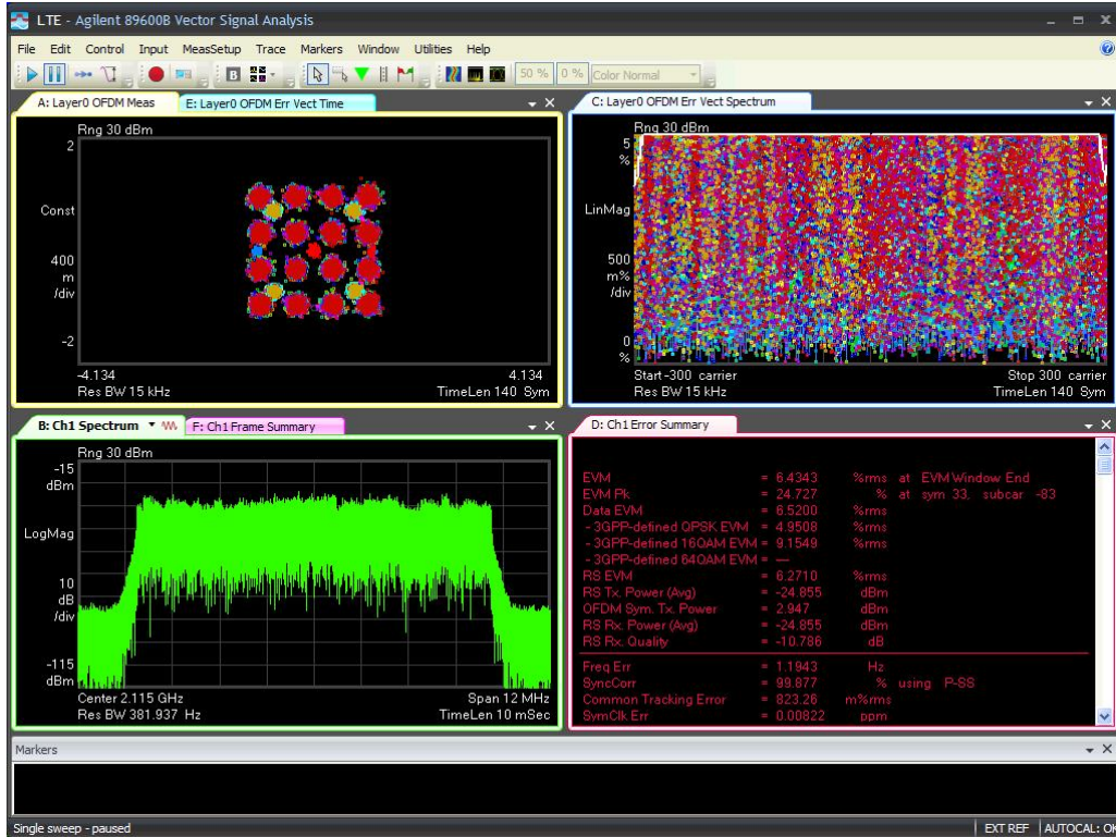
10M-Port 1 -2115MHz-TM3.3
