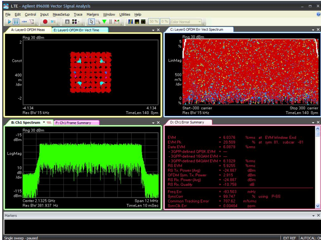
10M-Port 1 -2132.5MHz-TM3.2
