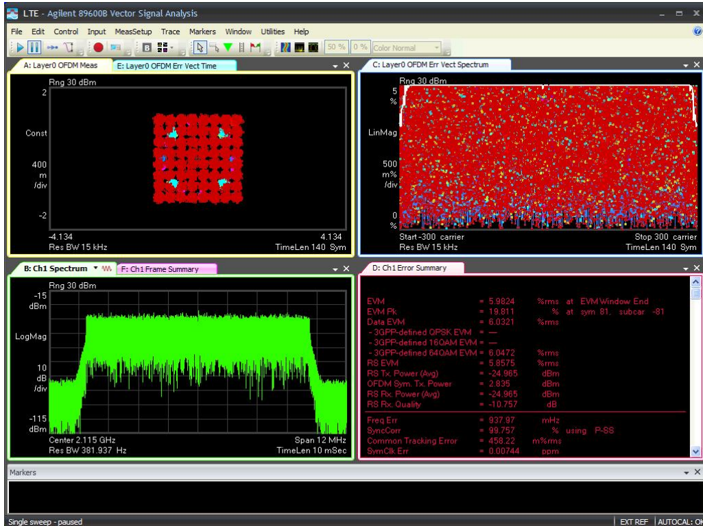
10M-Port 1 -2115MHz-TM3.2
