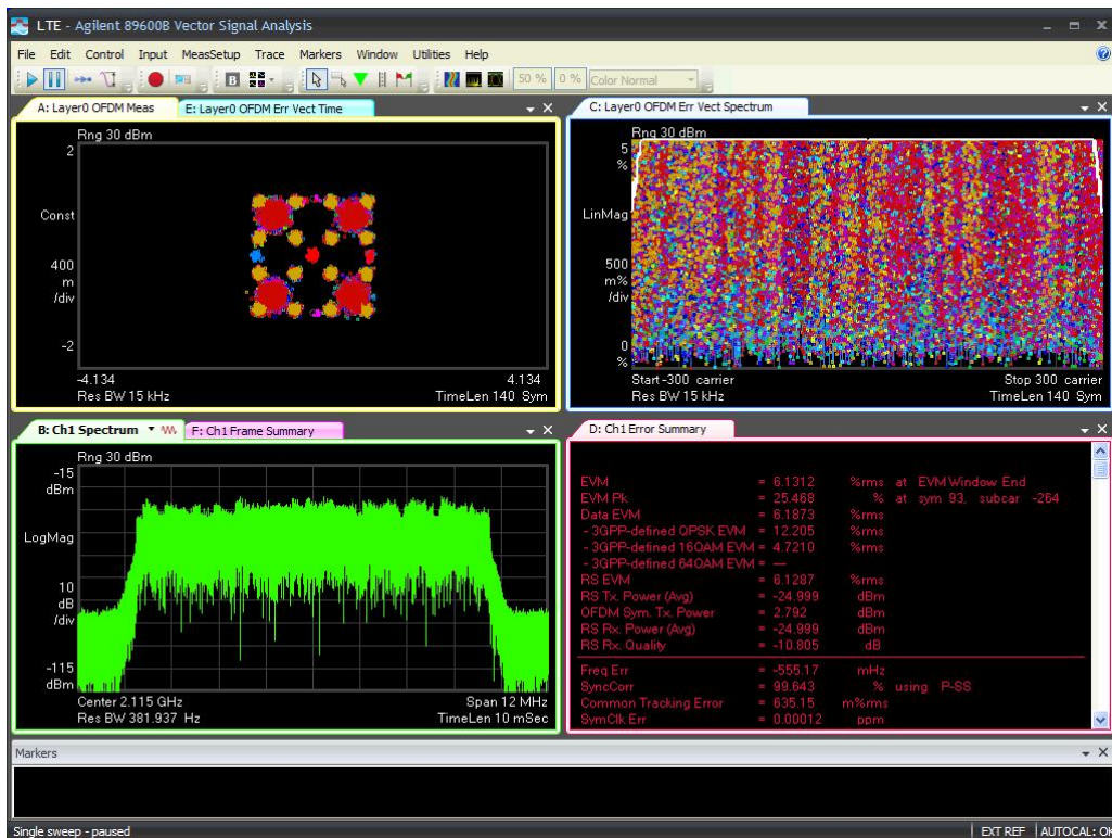
10M-Port 1 -2132.5MHz-TM2.0
