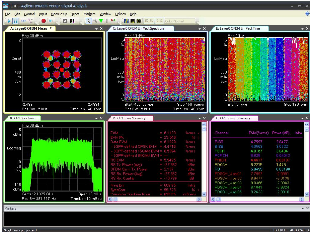
15M-Port 2-2132.5MHz-TM3.3
