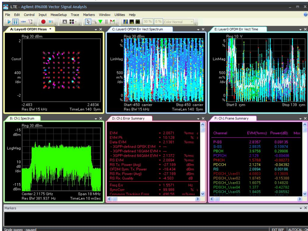
15M-Port 1 -2117.5MHz-TM2.0
