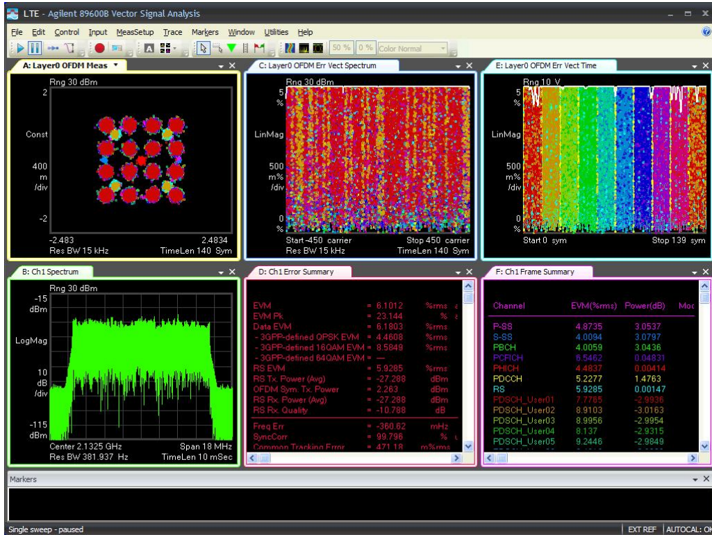
15M-Port 1 -2132.5MHz-TM3.3
