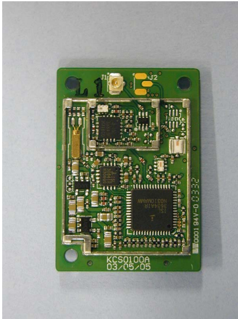
Solder side (without RF shielded) of Wireless LAN
