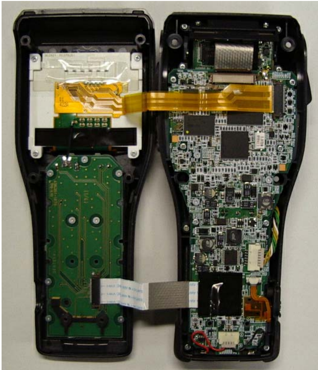
Assembling Case of Ber-code Handy Terminal
