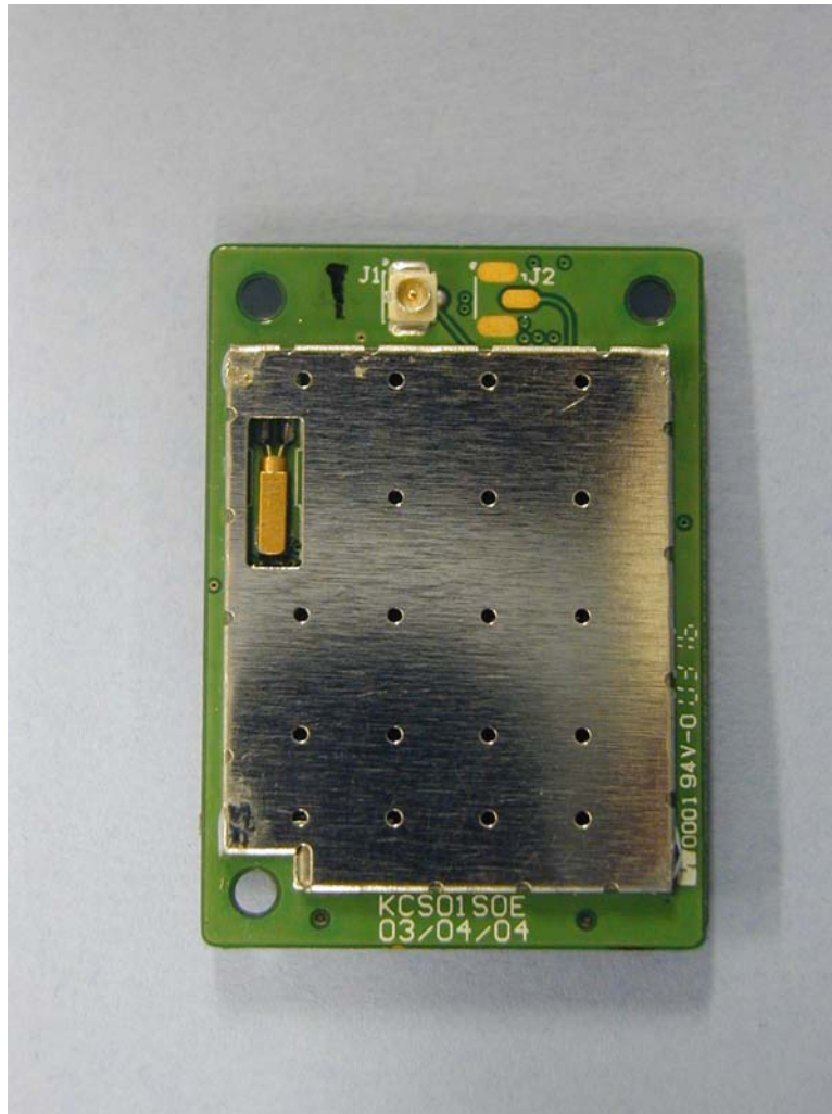
Solder side (with RF shield) of Wireless LAN
