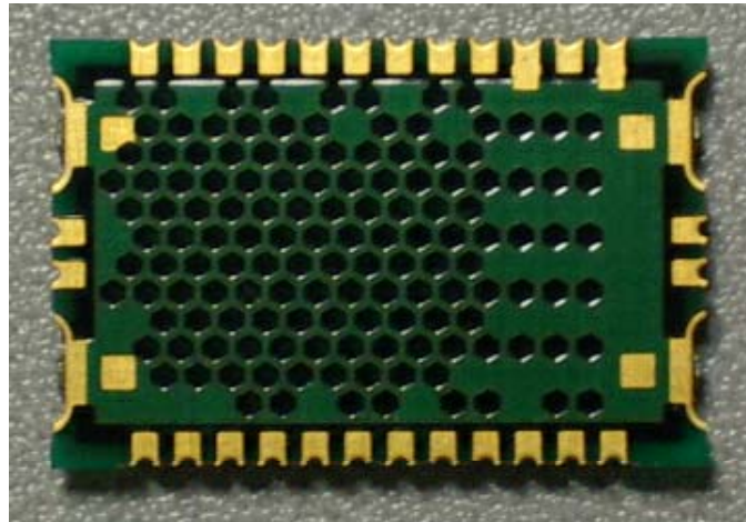
Rear of Bluetooth Module IC
