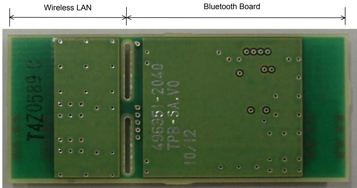
Rear of Solder Side
