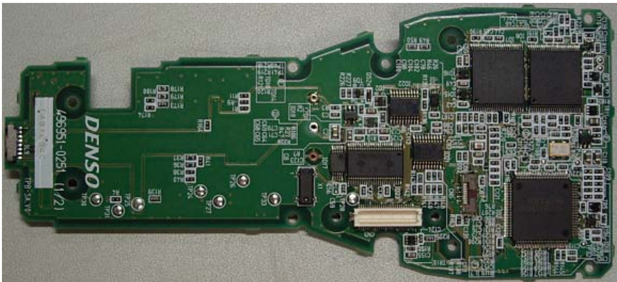
Solder Side of Main Board
