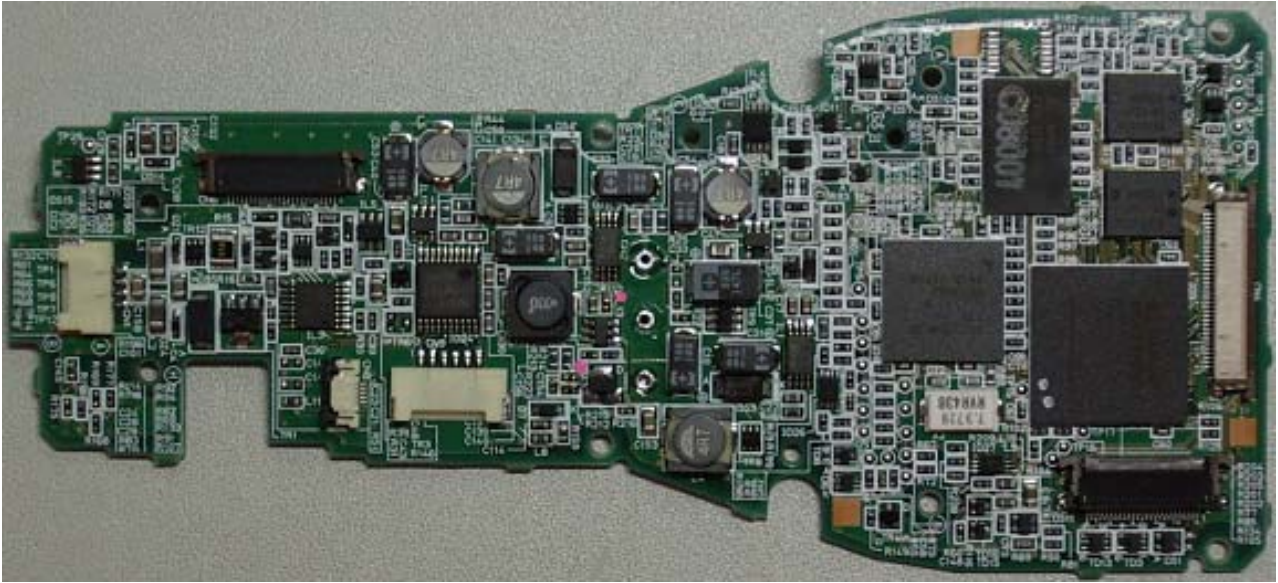
Component Side of Main Board
