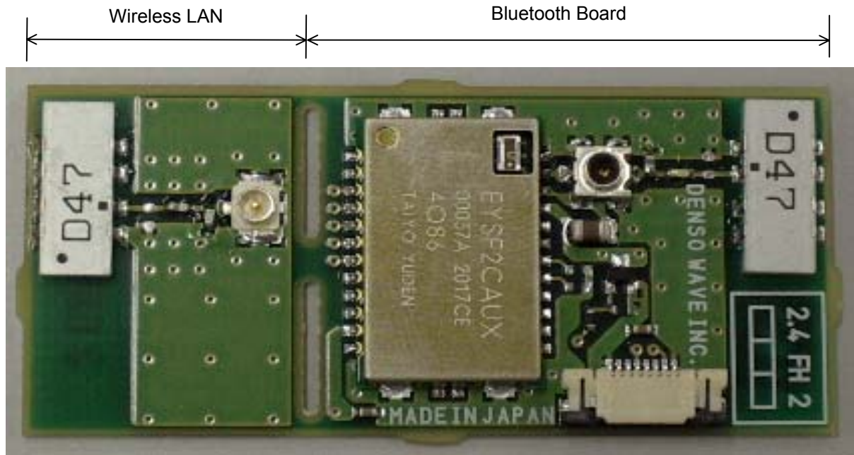
Front of Component Side
