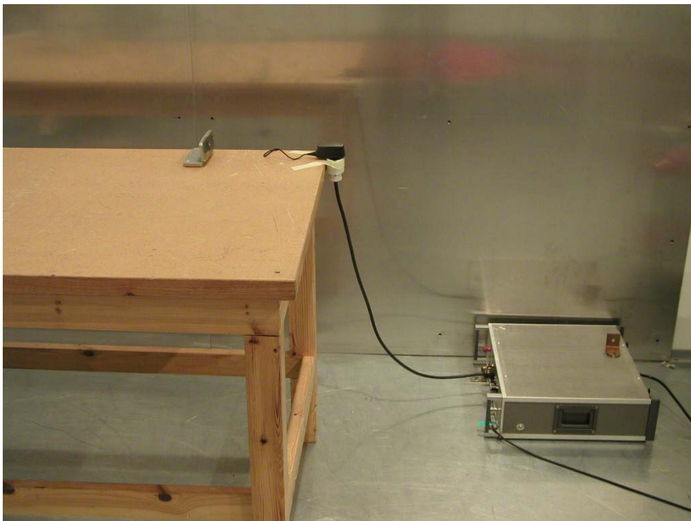
Photograph 2. AC power line conducted emissions test setup
