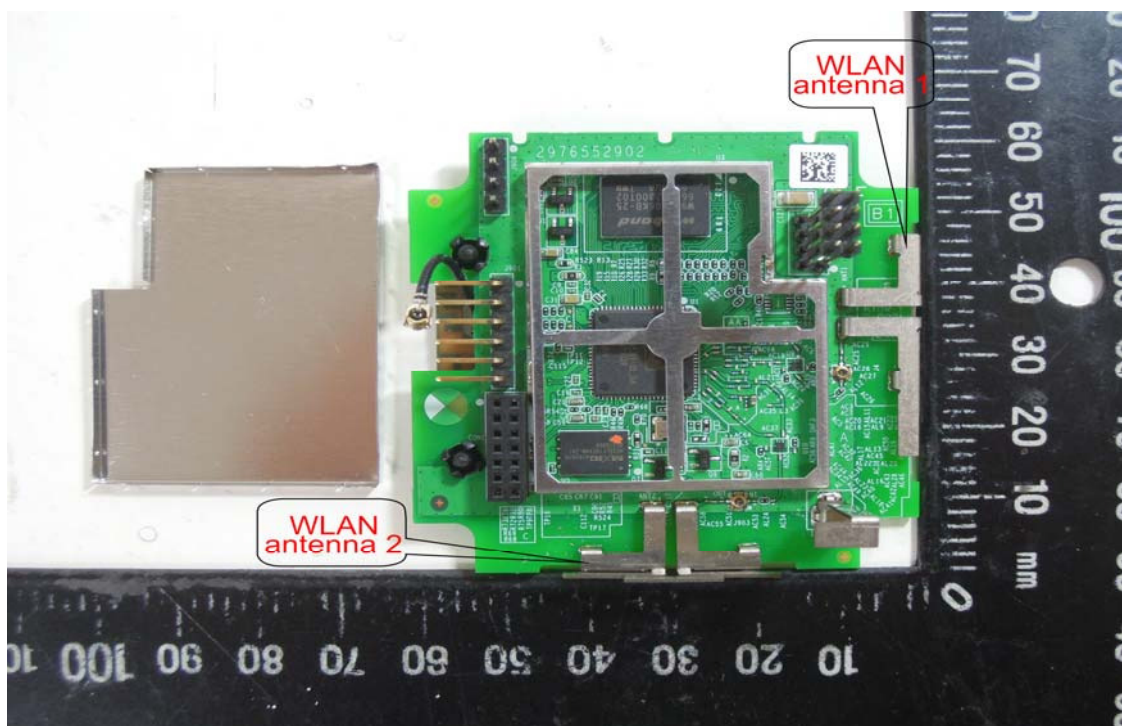
WLAN Antenna
