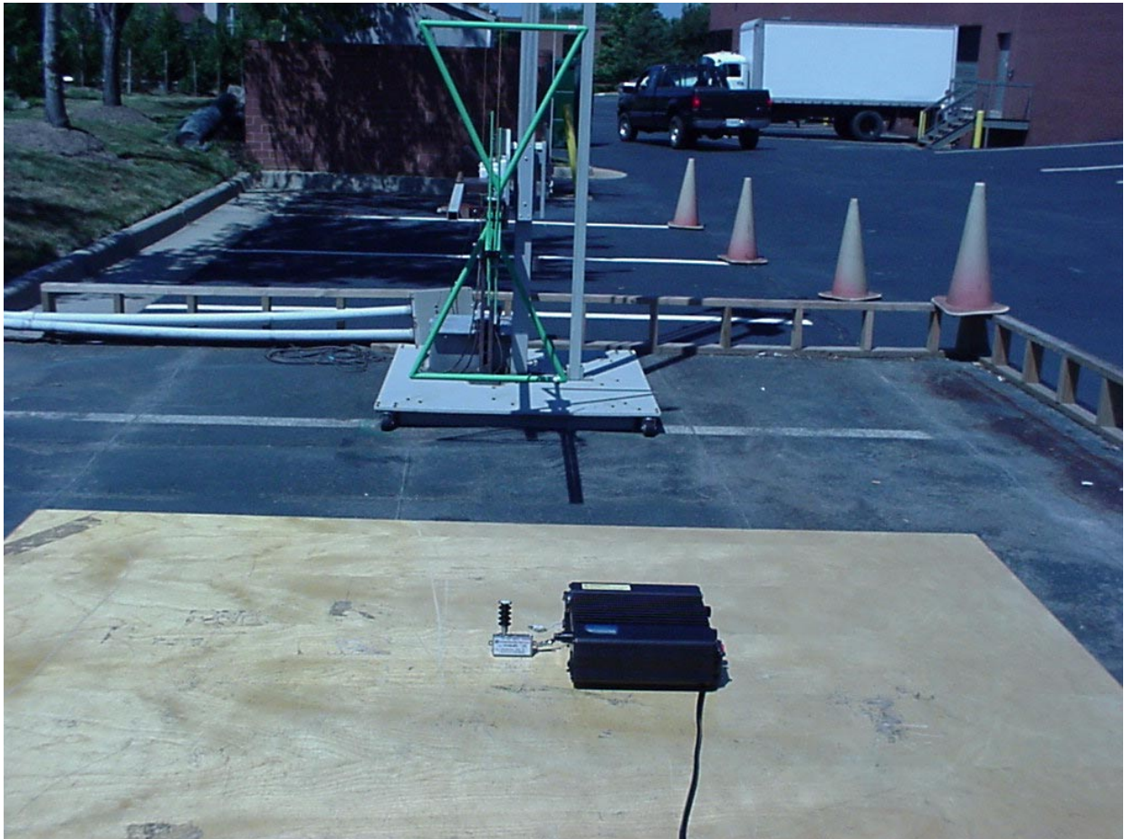
PHOTOGRAPH 1: RADIATED EMISSIONS FRONT VIEW (70 RX-M1)
