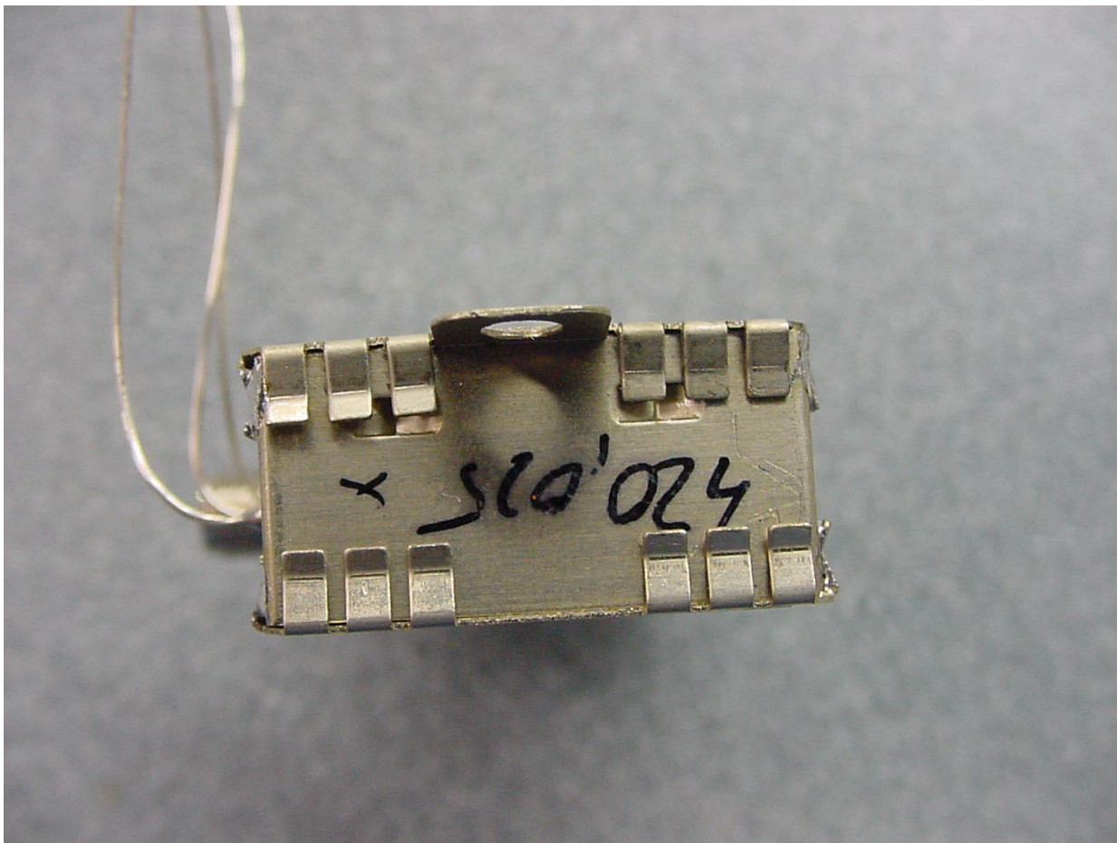
PHOTOGRAPH 6: RIGHT SIDE OF RECEIVER
