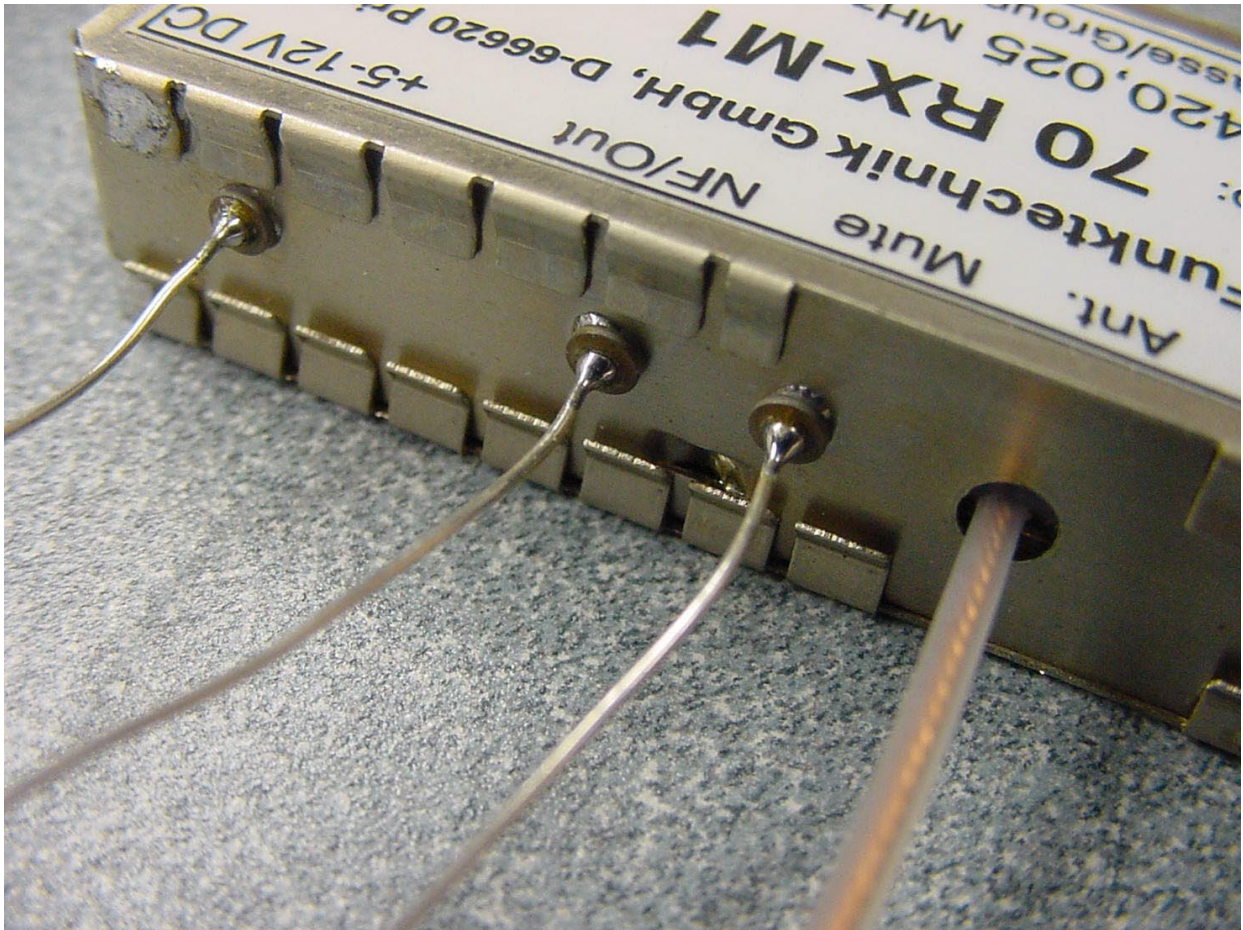
PHOTOGRAPH 11: VIEW OF CONNECTORS
