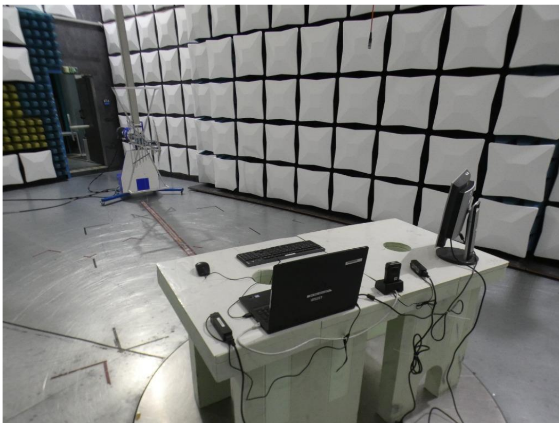
Photo 5: Test setup S03_AA01 for radiated emissions measurements below 1 GHz
