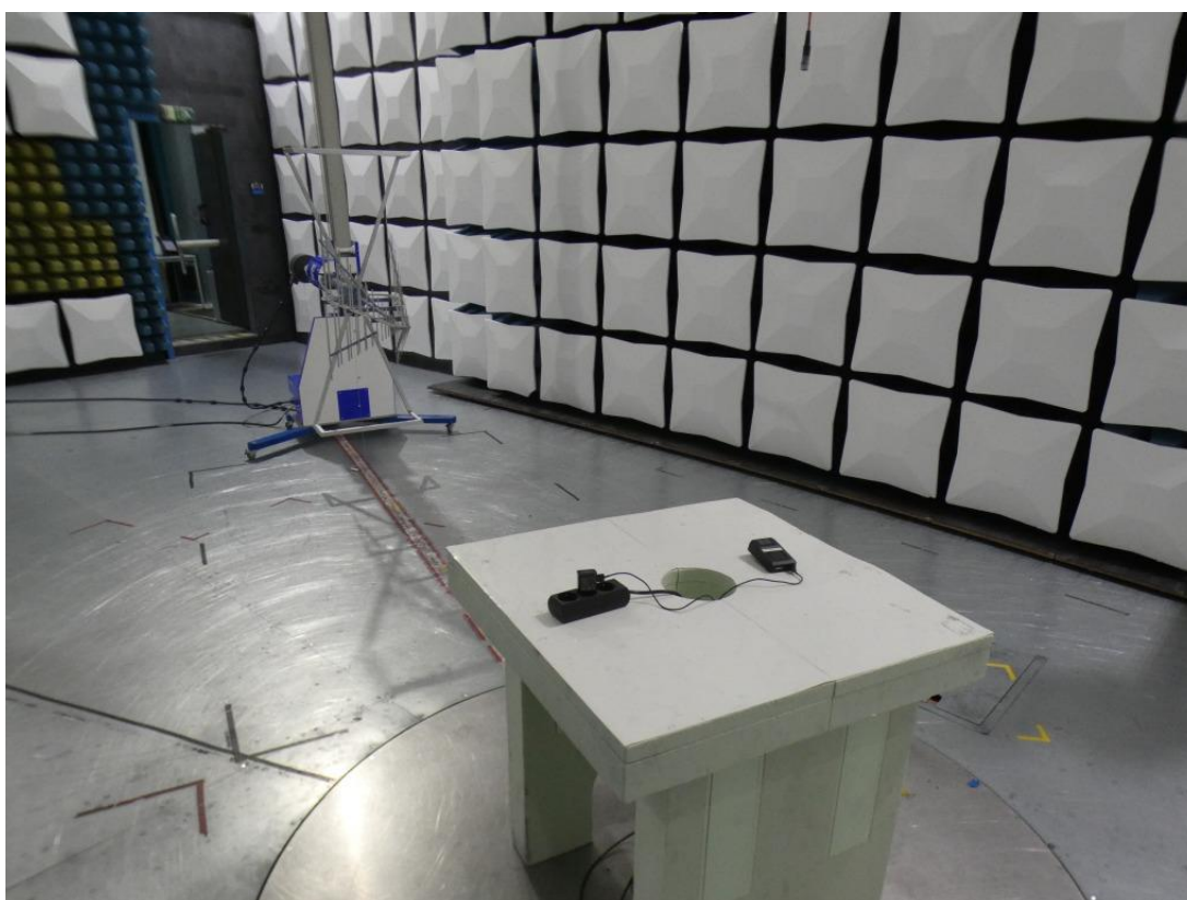
Photo 4: Test setup S02_AA01 for radiated emissions measurements below 1 GHz
