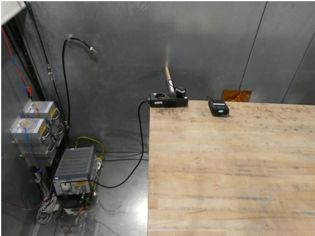
Photo 1: Test setup S02_AA01 for conducted emissions measurements below 30 MHz
