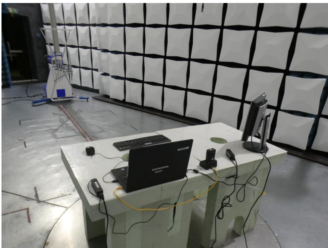
Photo 6: Test setup S04_AA01 for radiated emissions measurements below 1 GHz
