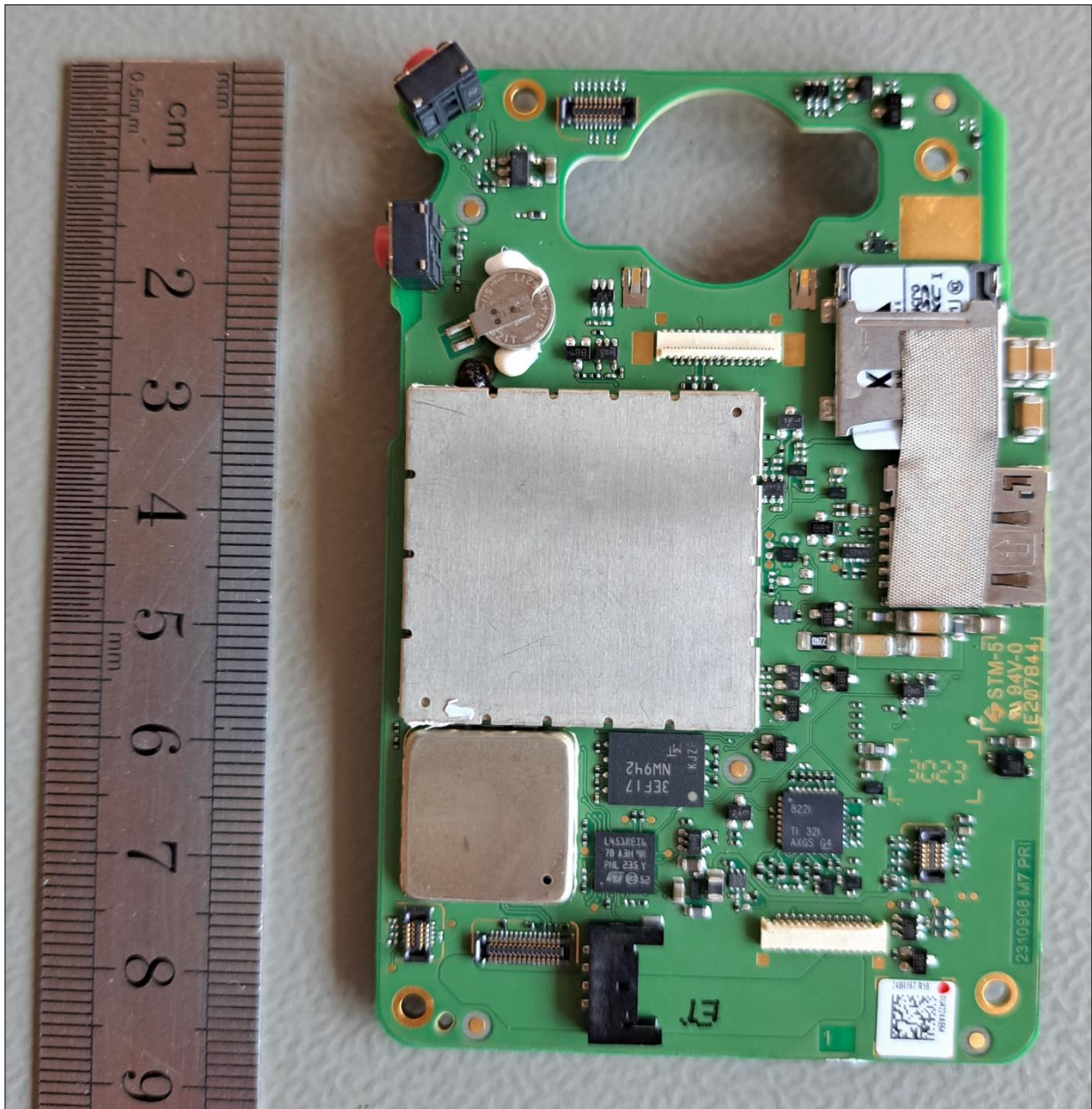
AXIS W120, main board, upper side.
