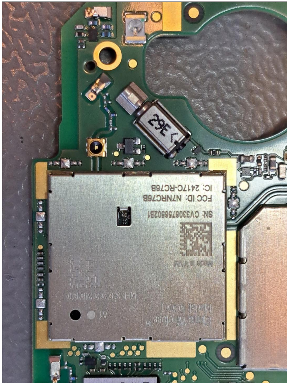
AXIS W120, main board detail: LTE module.
