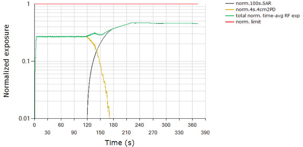
Total Normalized Time-averaged RF Exposure Tech: LTE, Band66/ Tech: NR5G MMW, Band n258
