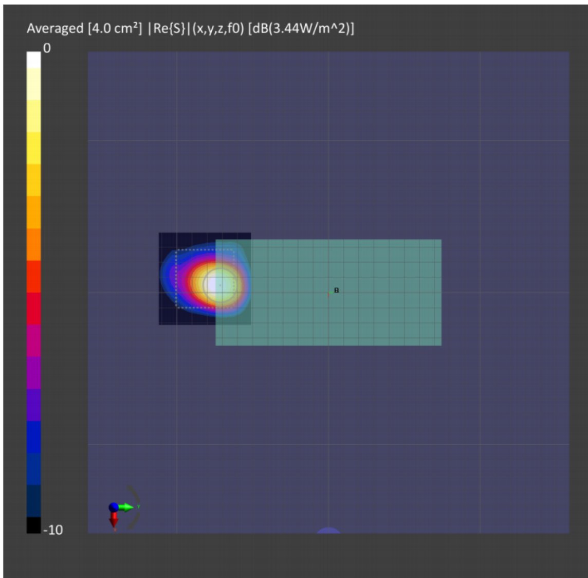
Figure 7-2: 4cm2-averaged power density distribution measured at input.power.limit of 7.6 dBm on the Top surface for n258 beam 20
