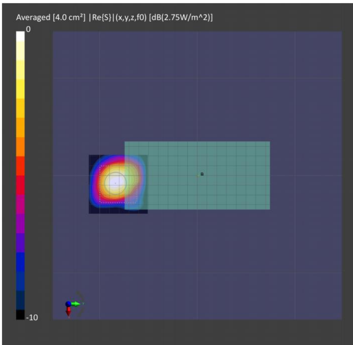
Figure 7-3: 4cm 2 -averaged power density distribution measured at input.power.limit of 7.68 dBm on the Top surface for n260 beam 28
