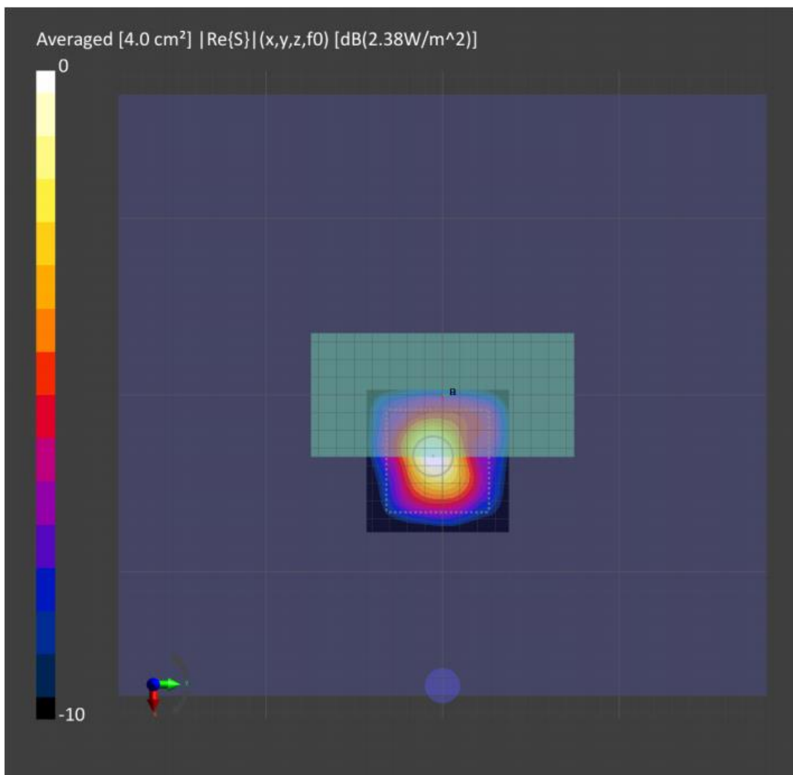
Figure 7-4: 4cm2-averaged power density distribution measured at input.power.limit of 13.34 dBm on the Top for n261 beam 0
