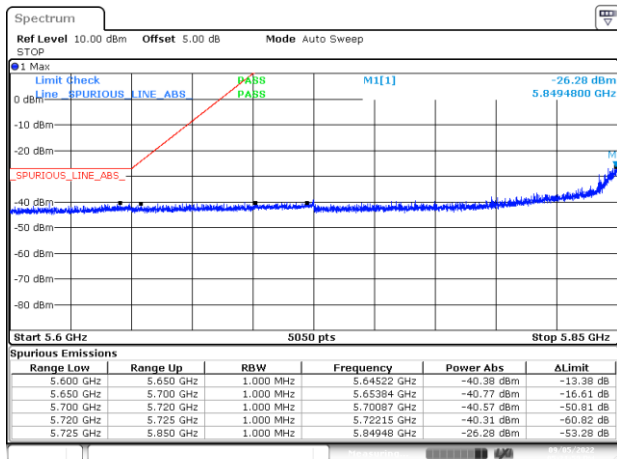
BE-NR-LOW, CHAIN A - DIV2, 802.11ax20-HE0, Ch177
