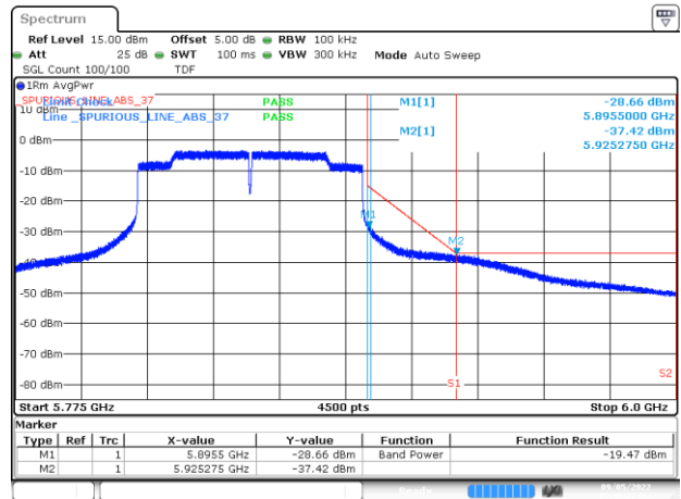
BE-NR-HIGH, CHAIN A - DIV2, 802.11ac80-VHT0, Ch171
