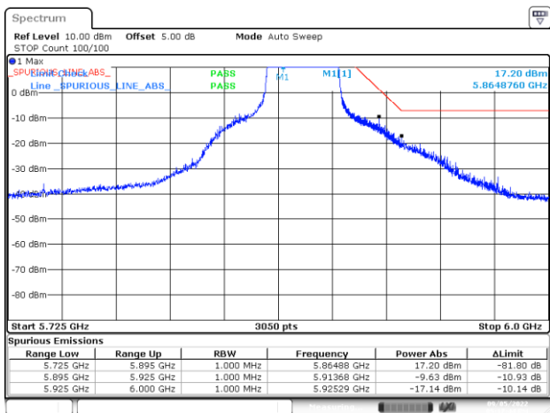
BE-NR-HIGH, CHAIN A - DIV2, 802.11n40-HT0, Ch175
