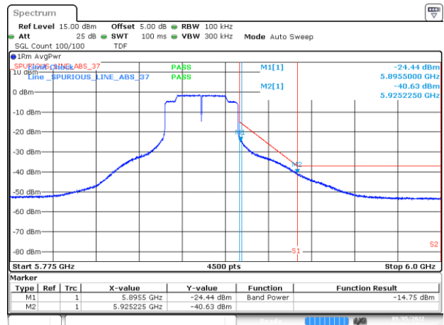
BE-NR-HIGH, CHAIN A - DIV1, 802.11ax40-HE0, Ch175
