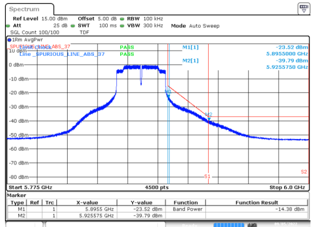
BE-NR-HIGH, CHAIN A - DIV2, 802.11n40-HT0, Ch175
