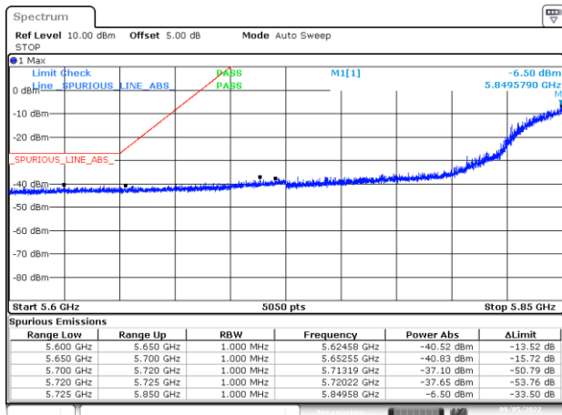
BE-NR-LOW, CHAIN A - DIV2, 802.11n40-HT0, Ch175
