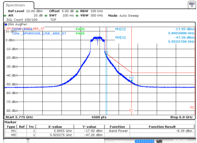
BE-NR-HIGH, CHAIN A - DIV2, 802.11a20-6Mbps, Ch177
