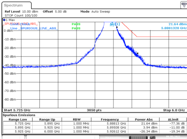
BE-NR-HIGH, CHAIN A - DIV1, 802.11a20-6Mbps, Ch177
