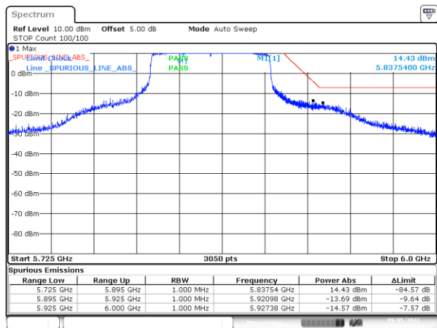
BE-NR-HIGH, CHAIN A - DIV2, 802.11ac80-VHT0, Ch171
