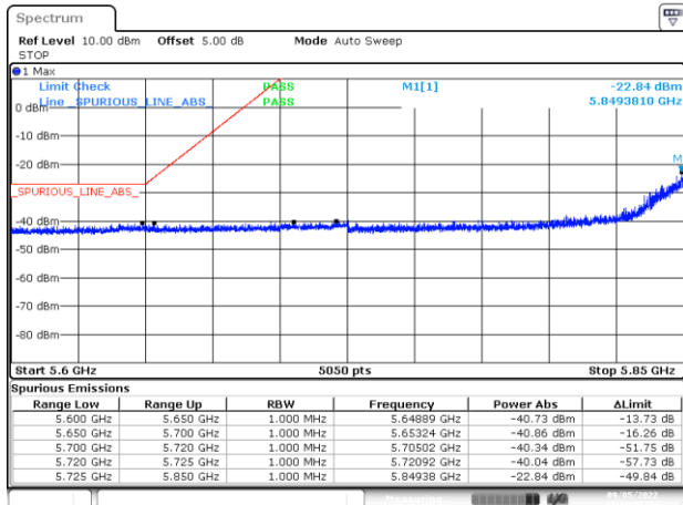
BE-NR-LOW, CHAIN A - DIV2, 802.11a20-6Mbps, Ch177
