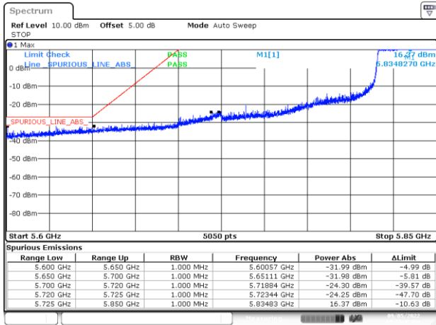
BE-NR-LOW, CHAIN A - DIV2, 802.11ax80-HE0, Ch171
