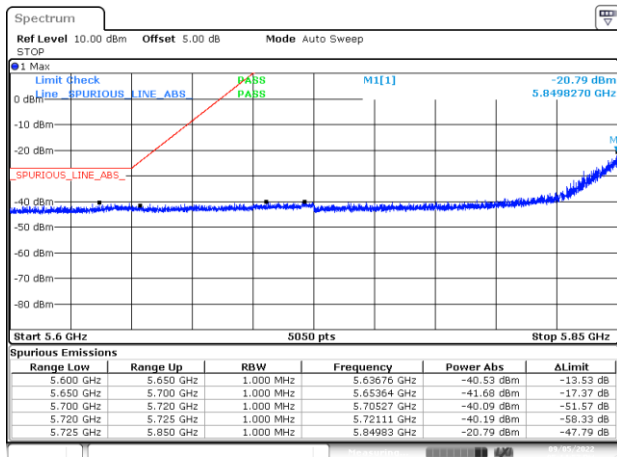
BE-NR-LOW, CHAIN A - DIV2, 802.11n20-HT0, Ch177
