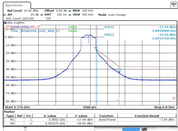
BE-NR-HIGH, CHAIN A - DIV1, 802.11ax20-HE0, Ch177
