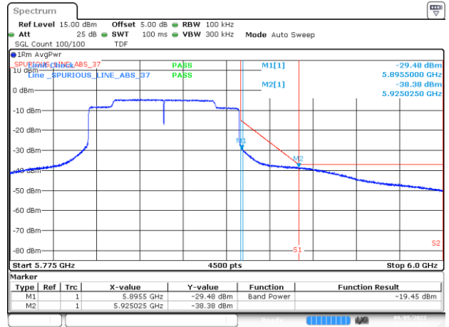
BE-NR-HIGH, CHAIN A - DIV2, 802.11ax80-HE0, Ch171
