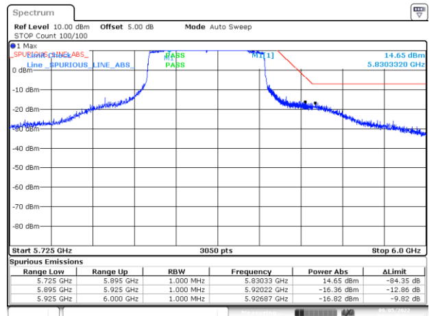
BE-NR-HIGH, CHAIN A - DIV1, 802.11ac80-VHT0, Ch171
