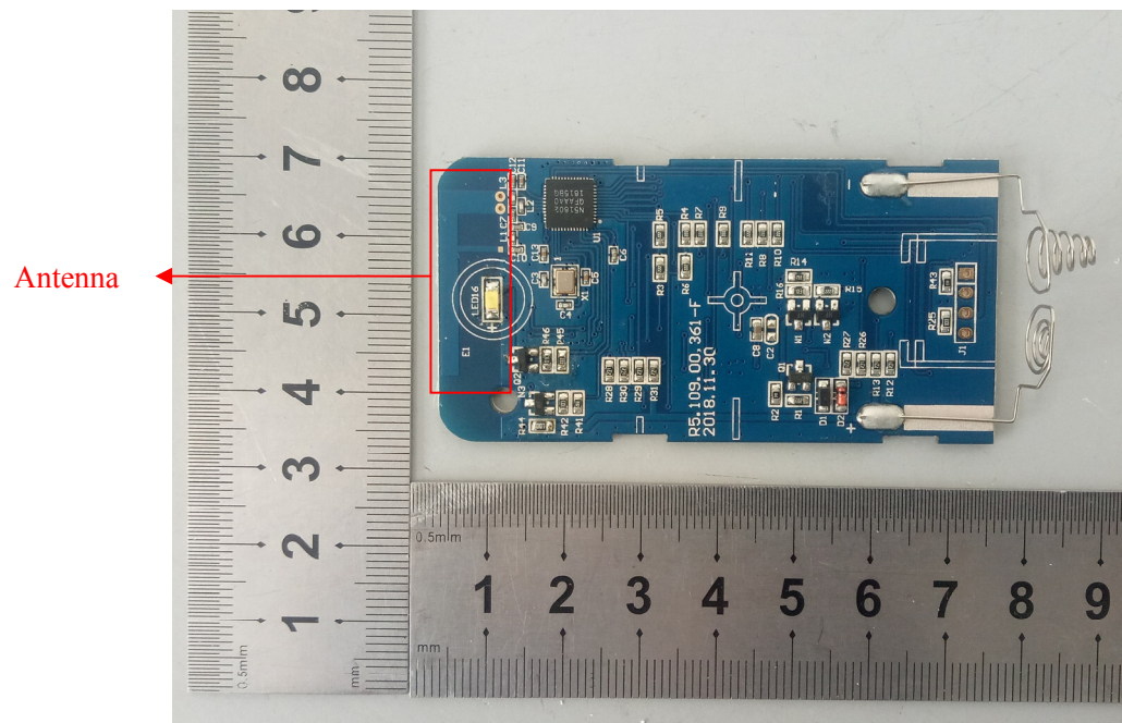
EUT – PCB Bottom Chip View
