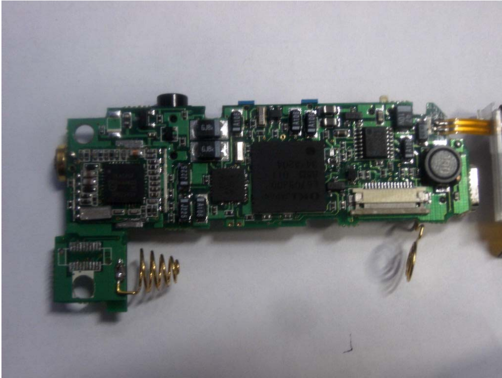
<Rear Photo of MainBoard>
