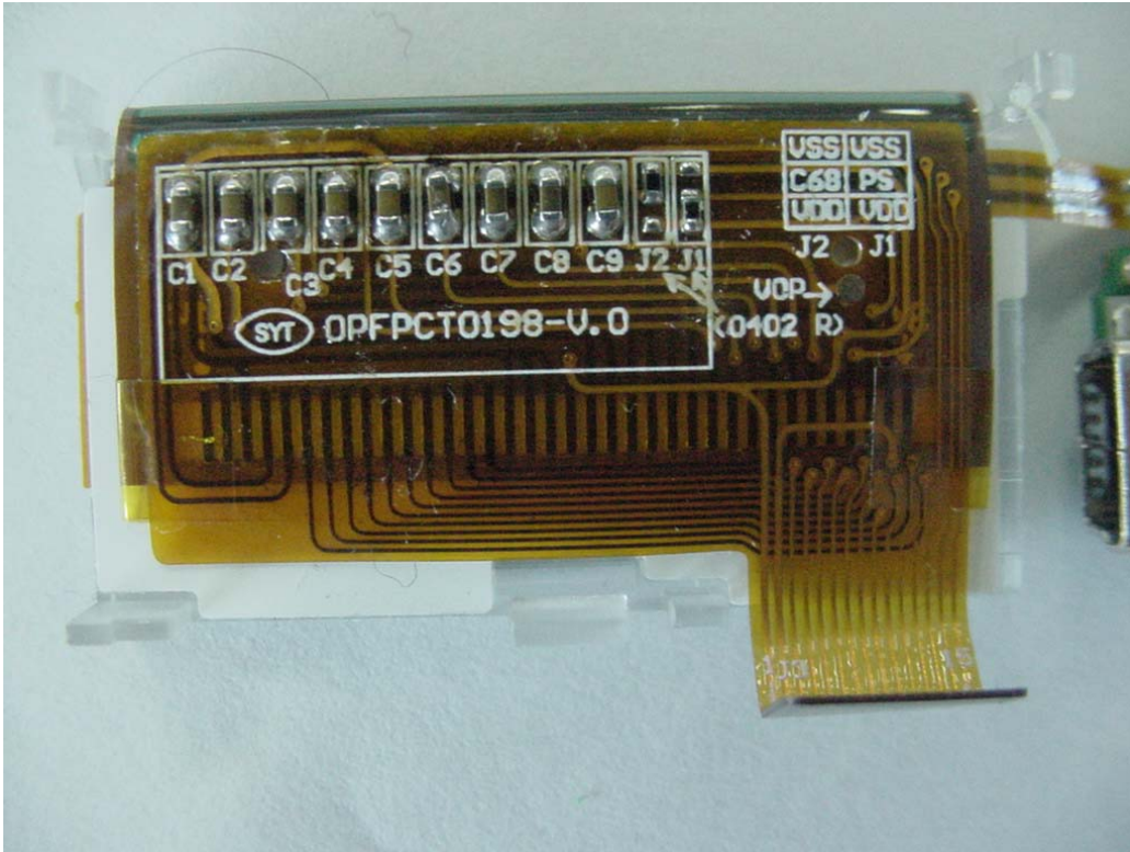
<Rear Photo of Display>
