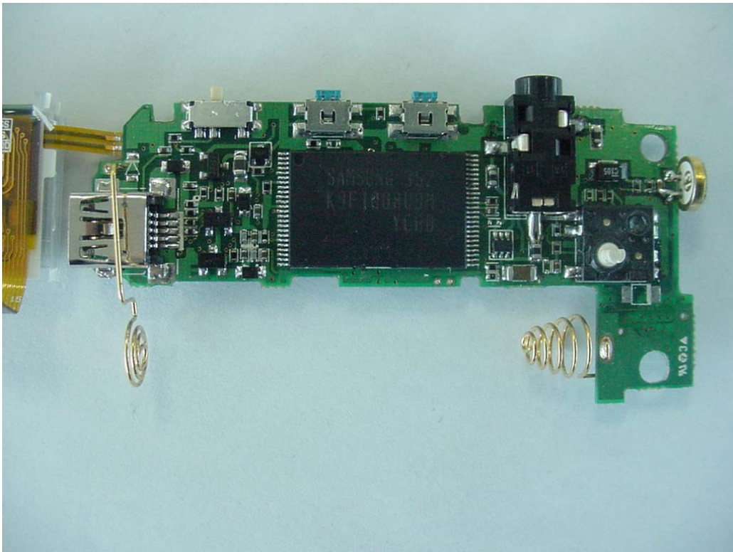
<Front Photo of MainBoard>
