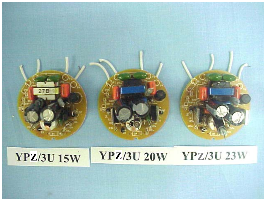
FIGURE 2 ENERGY SAVING LAMP (M/N: YPZ/3U 15W/20W/23W) MAIN BOARD (COMPONENT SIDE)
