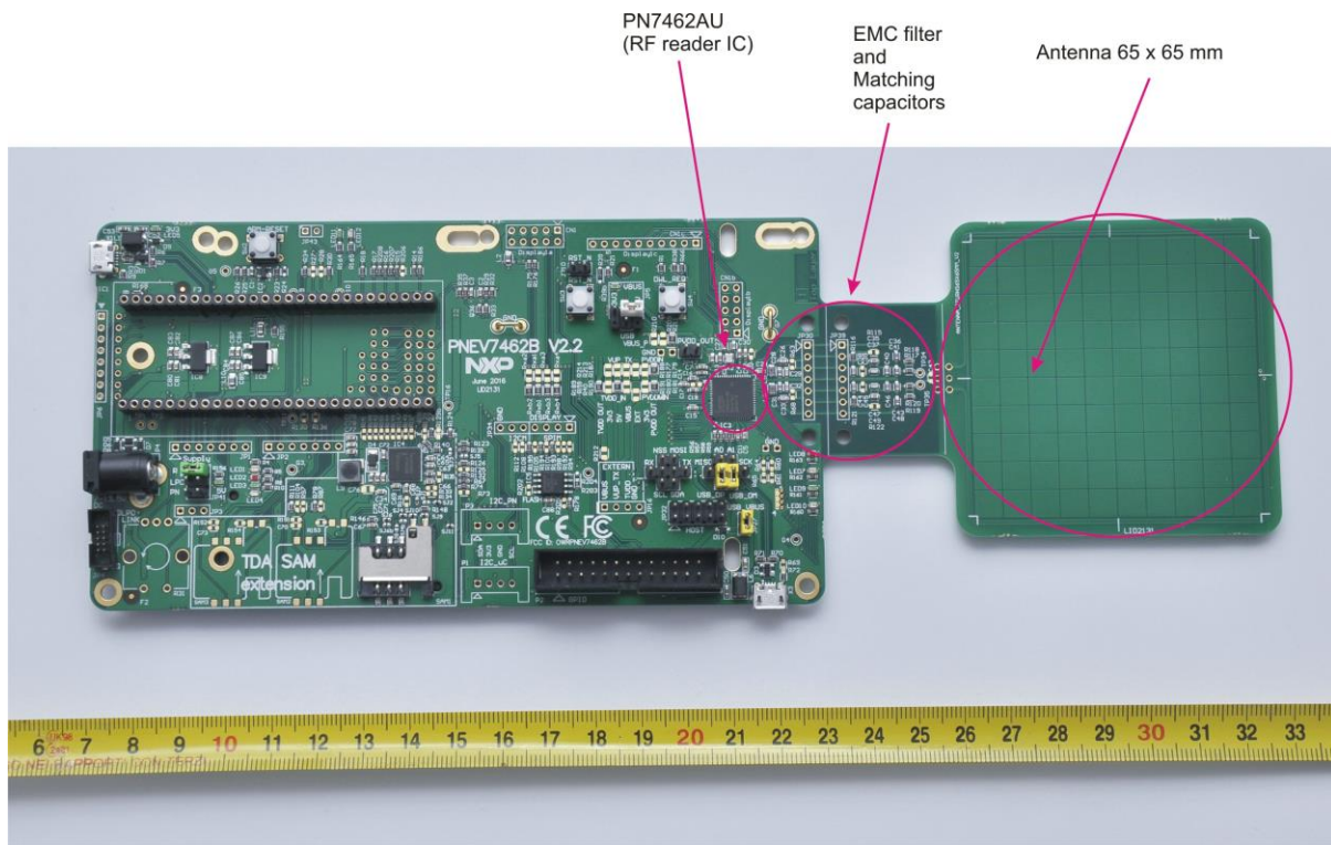
Picture 1: Customer Development Board PNEV7462B - top view.
