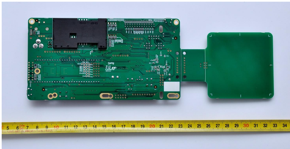
Picture 2: Customer Development Board PNEV7462B - bottom view.
