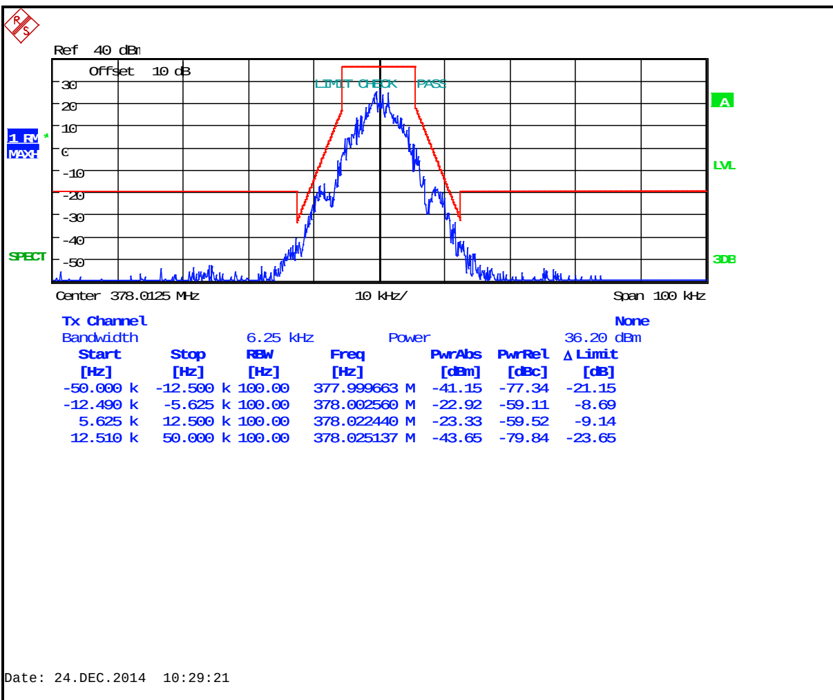
Plot 7-37: Occupied Bandwidth – 378.0125 MHz; EDACS Narrowband 2-level FSK 9600 (Mask D)
