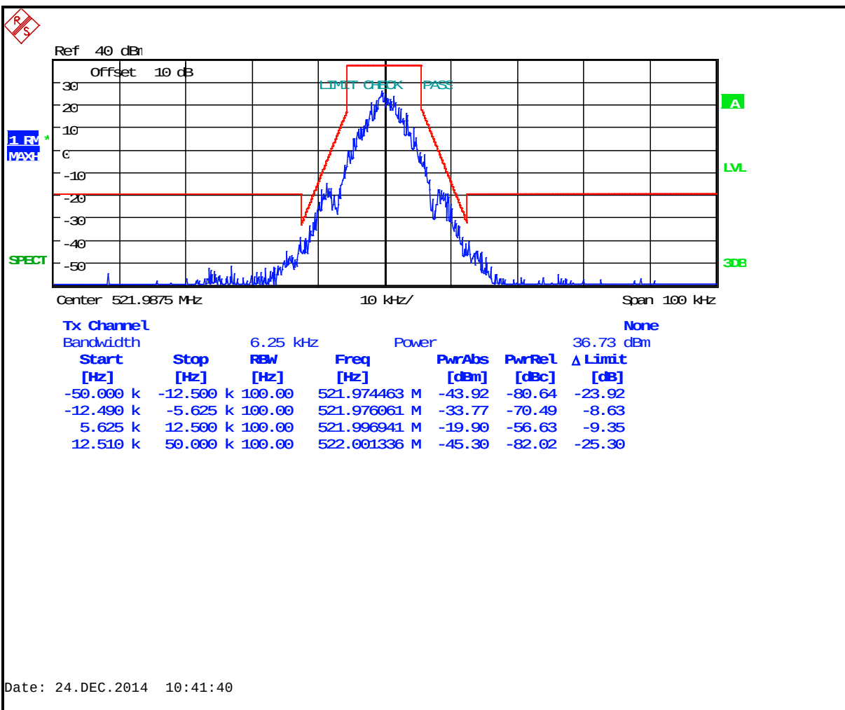
Plot 7-48: Occupied Bandwidth – 521.9875 MHz; EDACS Narrowband 2-level FSK 9600 (Mask D)
