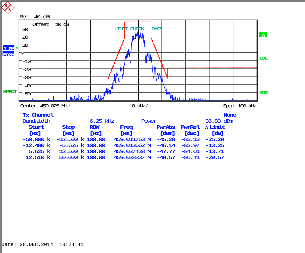
Plot 7-32: Occupied Bandwidth – 459.0250 MHz; EDACS Narrowband 2-level FSK 4800 (Mask D)
