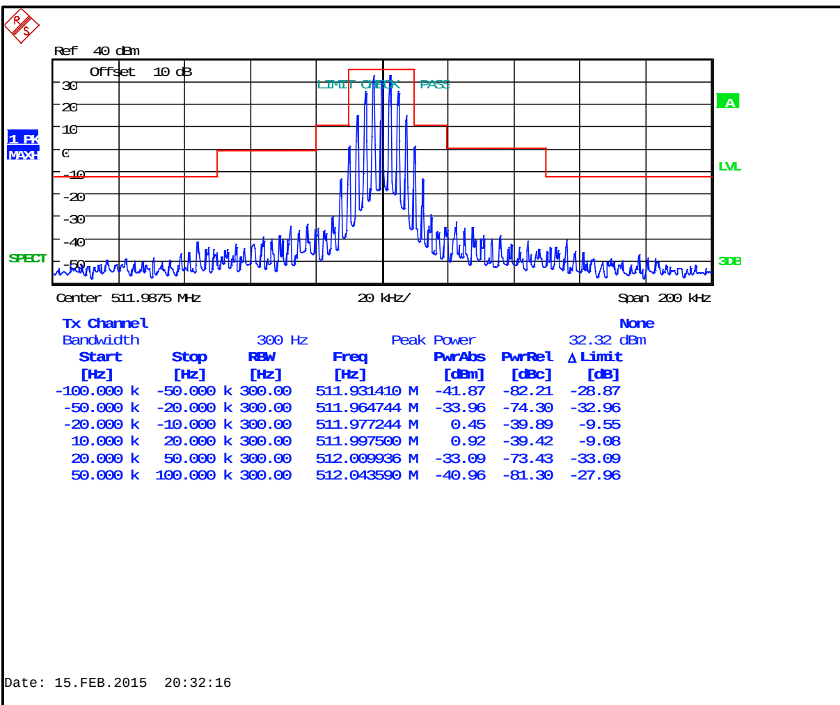
Plot 7-23: Occupied Bandwidth – 511.9875 MHz; Wideband Analog (Mask B)
