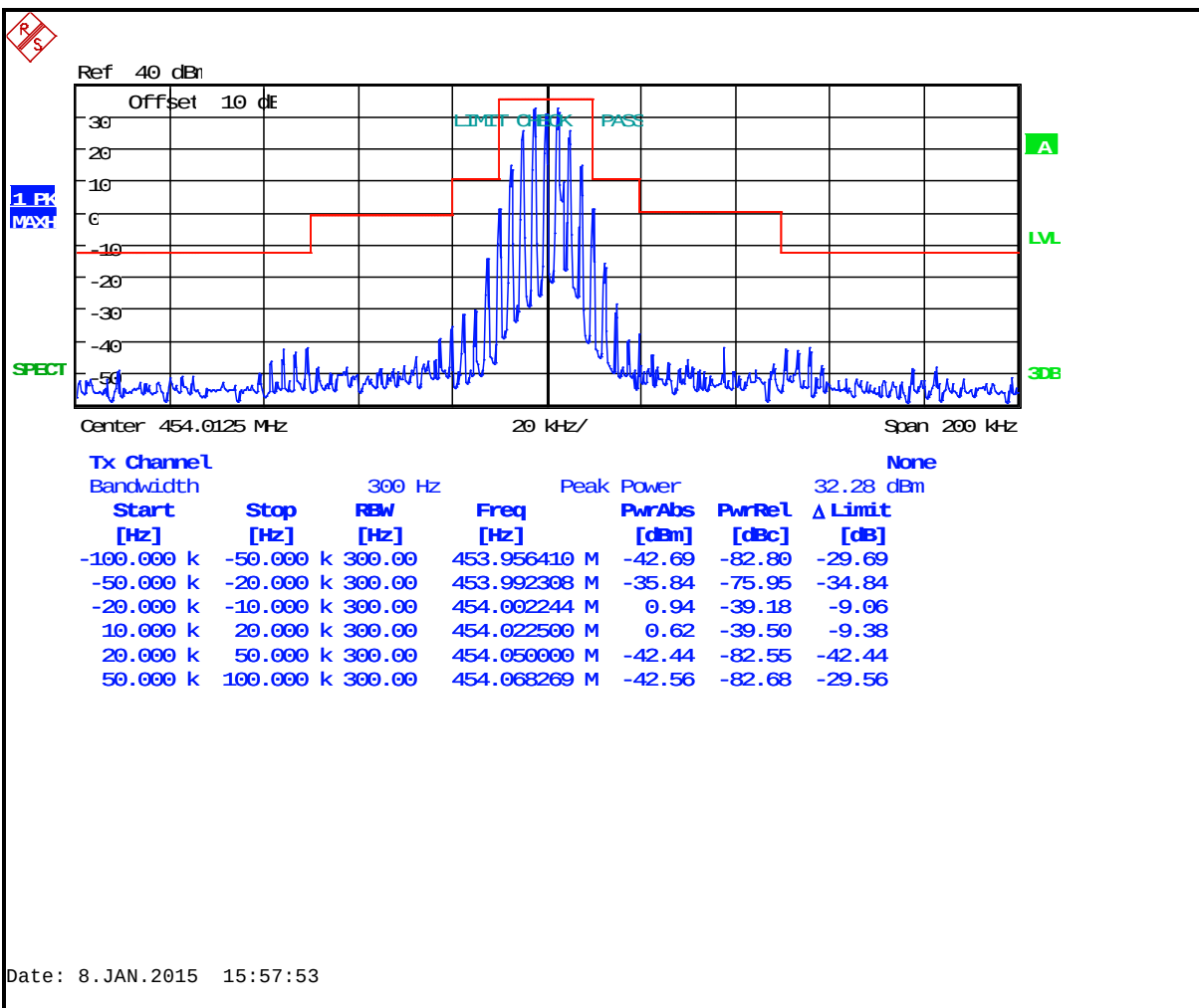
Plot 7-18: Occupied Bandwidth – 454.0125 MHz; Wideband Analog (Mask B)
