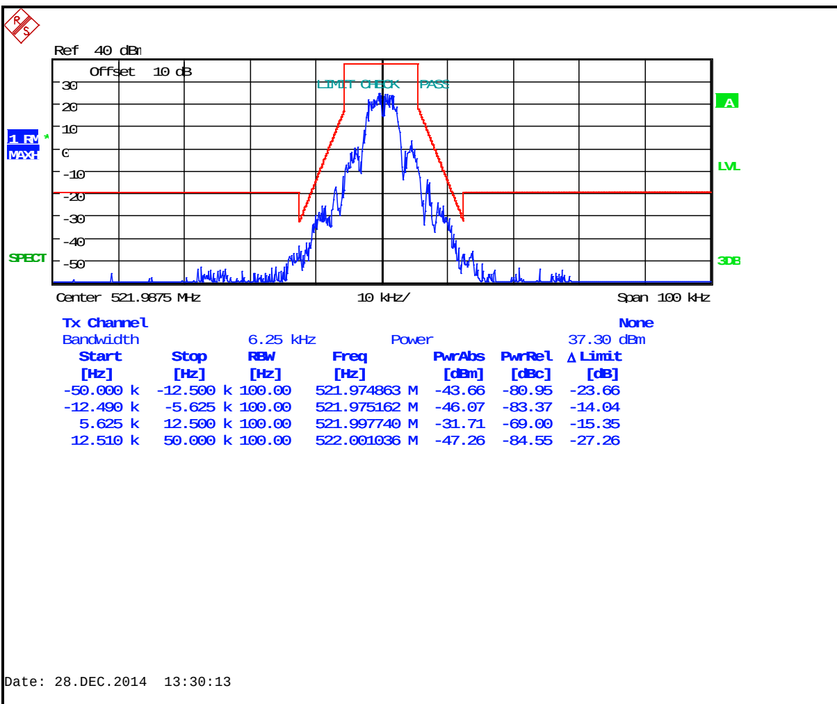
Plot 7-36: Occupied Bandwidth – 521.9875 MHz; EDACS Narrowband 2-level FSK 4800 (Mask D)
