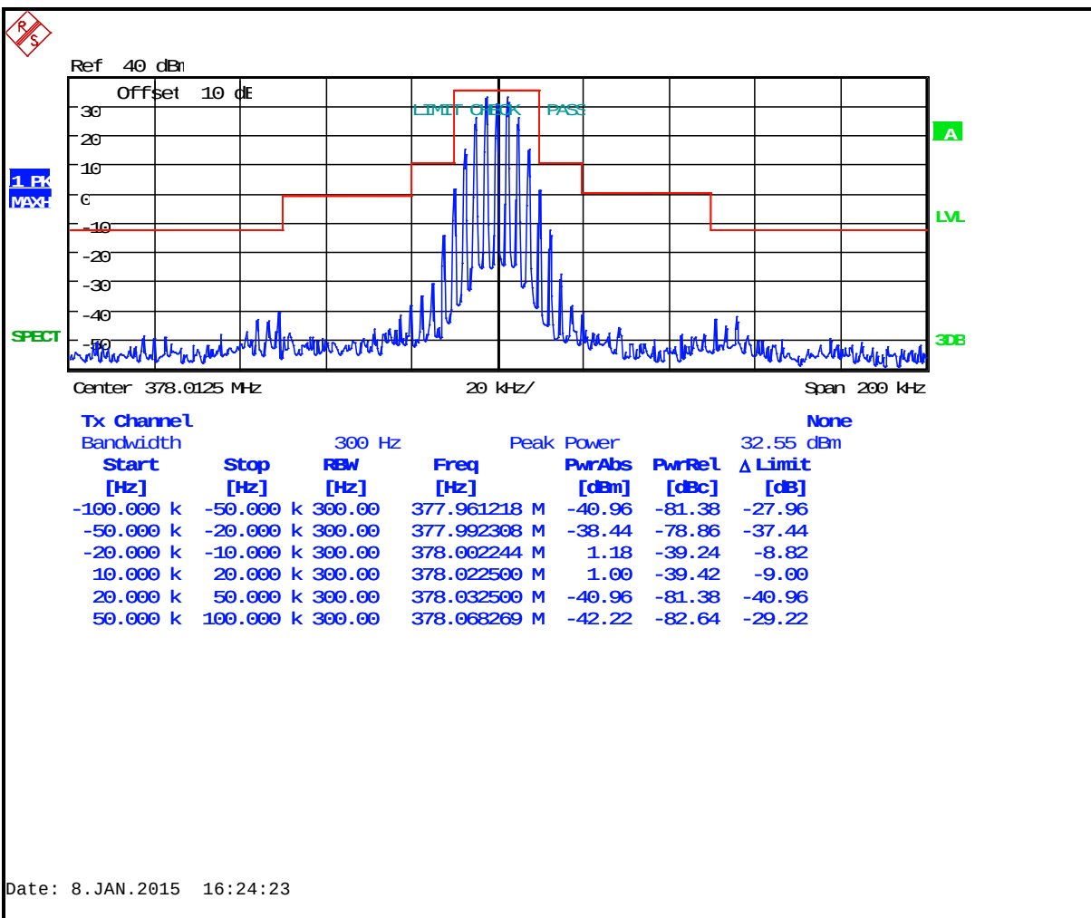
Plot 7-13: Occupied Bandwidth – 378.0125 MHz; Wideband Analog (Mask B)
