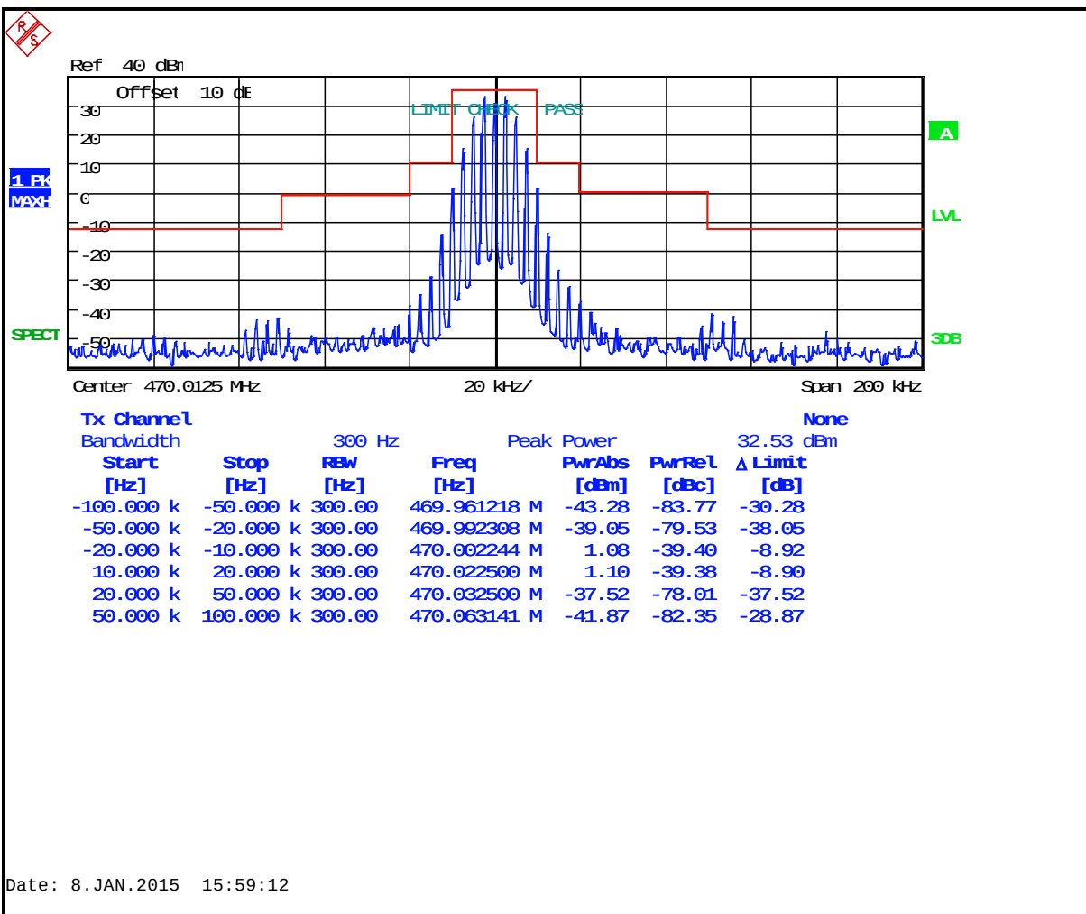
Plot 7-22: Occupied Bandwidth – 470.0125 MHz; Wideband Analog (Mask B)
