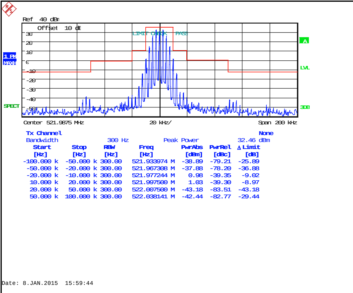
Plot 7-24: Occupied Bandwidth – 521.9875 MHz; Wideband Analog (Mask B)
