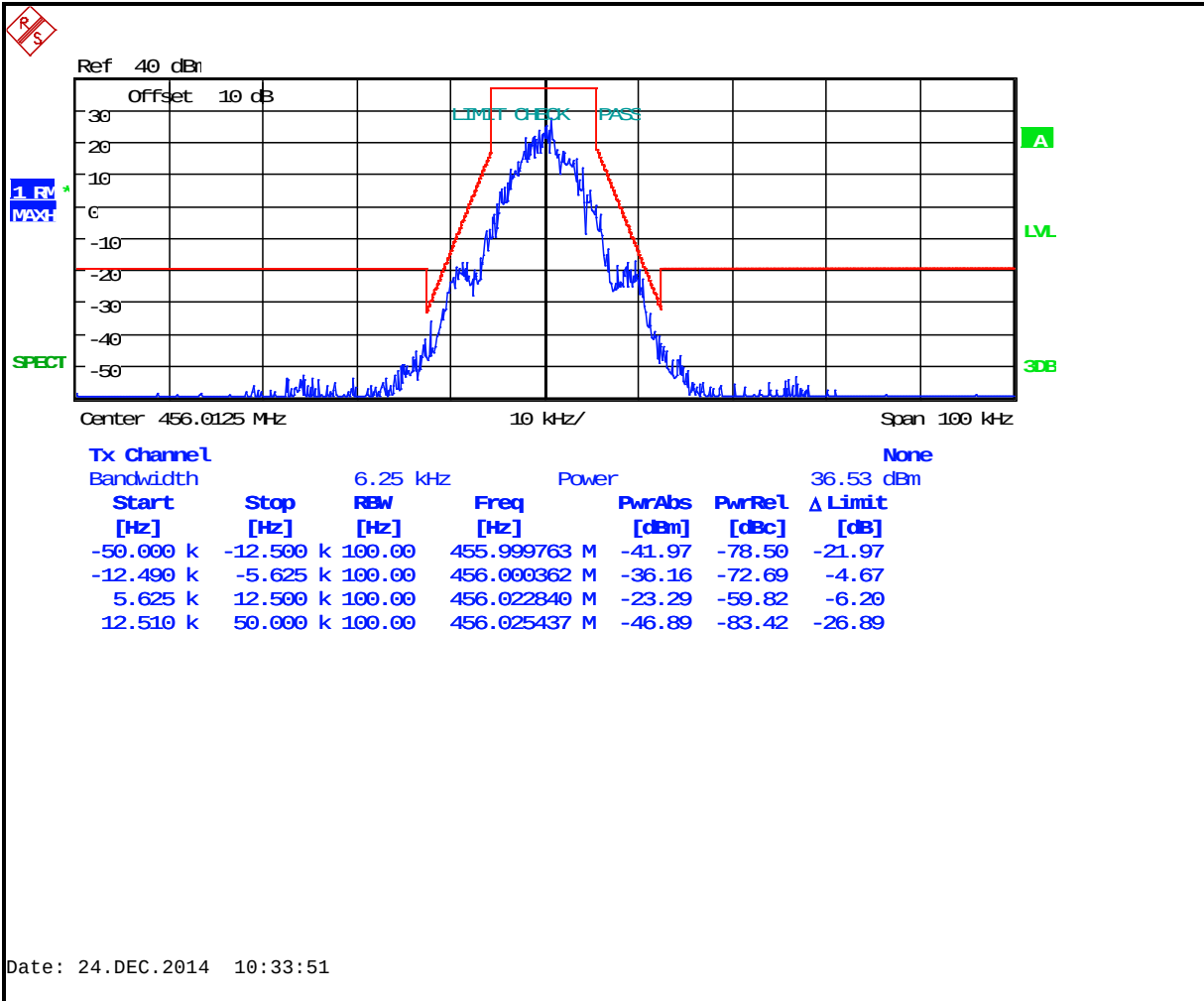
Plot 7-43: Occupied Bandwidth – 456.0125 MHz; EDACS Narrowband 2-level FSK 9600 (Mask D)
