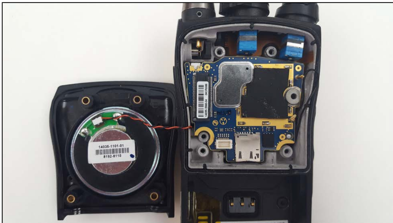
Rear Cover Removed; Expansion Board without LTE Module
