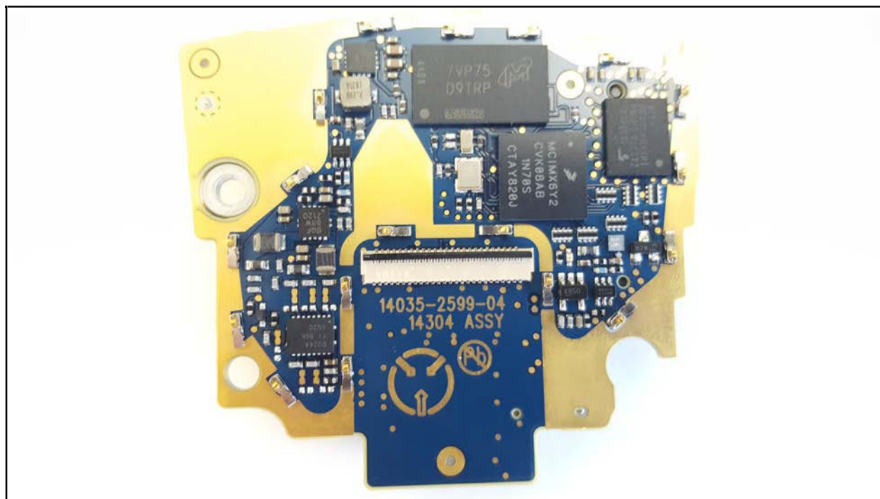
Expansion Board without LTE Processor Shield – Bottom
