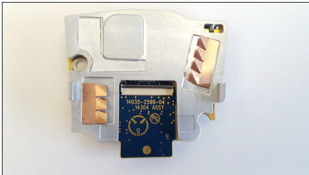
Expansion Board with LTE Processor Shield – Bottom
