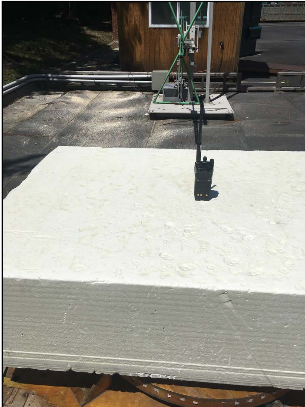
Photograph 4: Radiated Emissions (Spurious/Harmonics) Under 1 GHz, Back View
