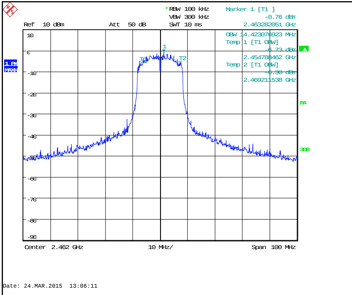
Plot 5-6: 6 dB Bandwidth Channel 11 (TX Frequency 2462 MHz) - 802.11g
