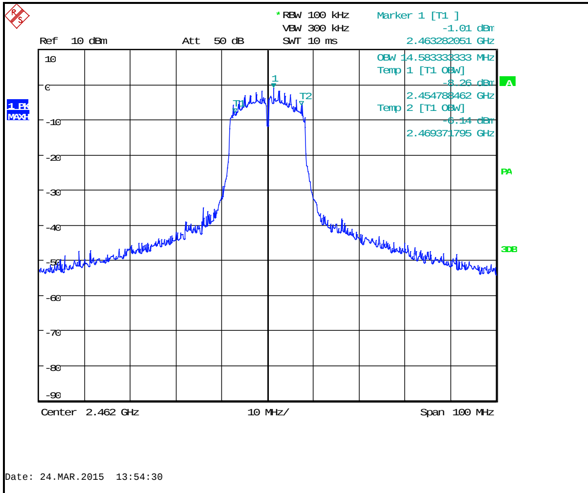
Plot 5-9: 6 dB Bandwidth Channel 11 (TX Frequency 2462 MHz-20 MHz BW) - 802.11n
