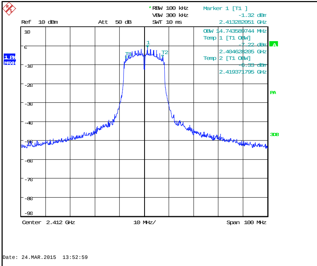
Plot 5-7: 6 dB Bandwidth Channel 1 (TX Frequency 2412 MHz-20 MHz BW) - 802.11n
