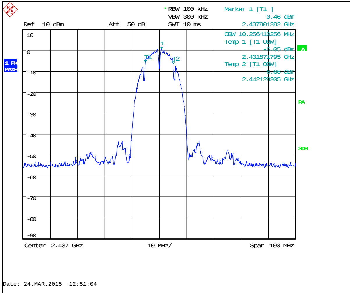
Plot 5-2: 6 dB Bandwidth Channel 6 (TX Frequency 2437 MHz) - 802.11b
