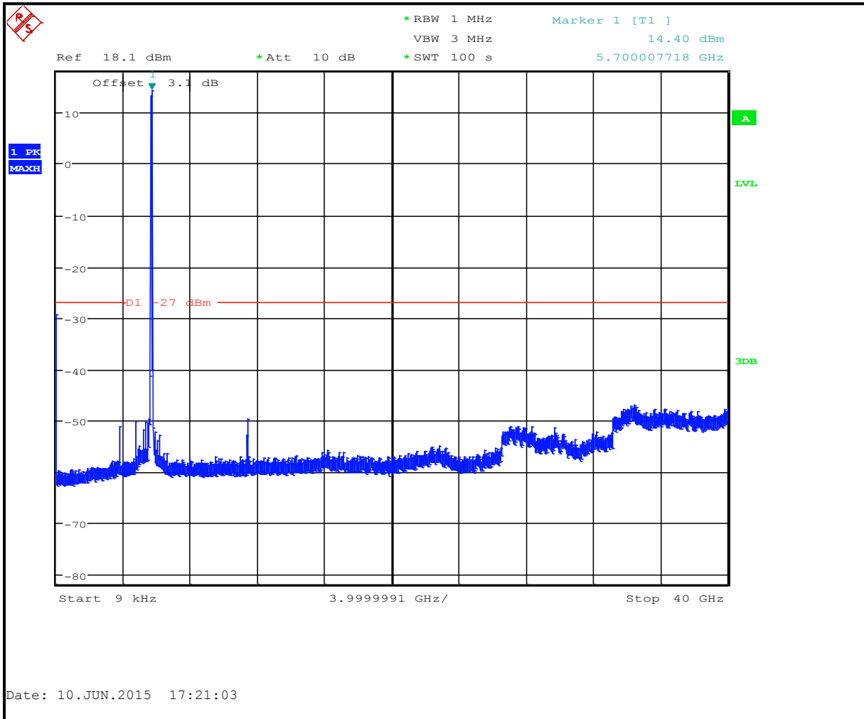
Plot 7-12: Undesirable Emissions Channel 140 (5700 MHz)
