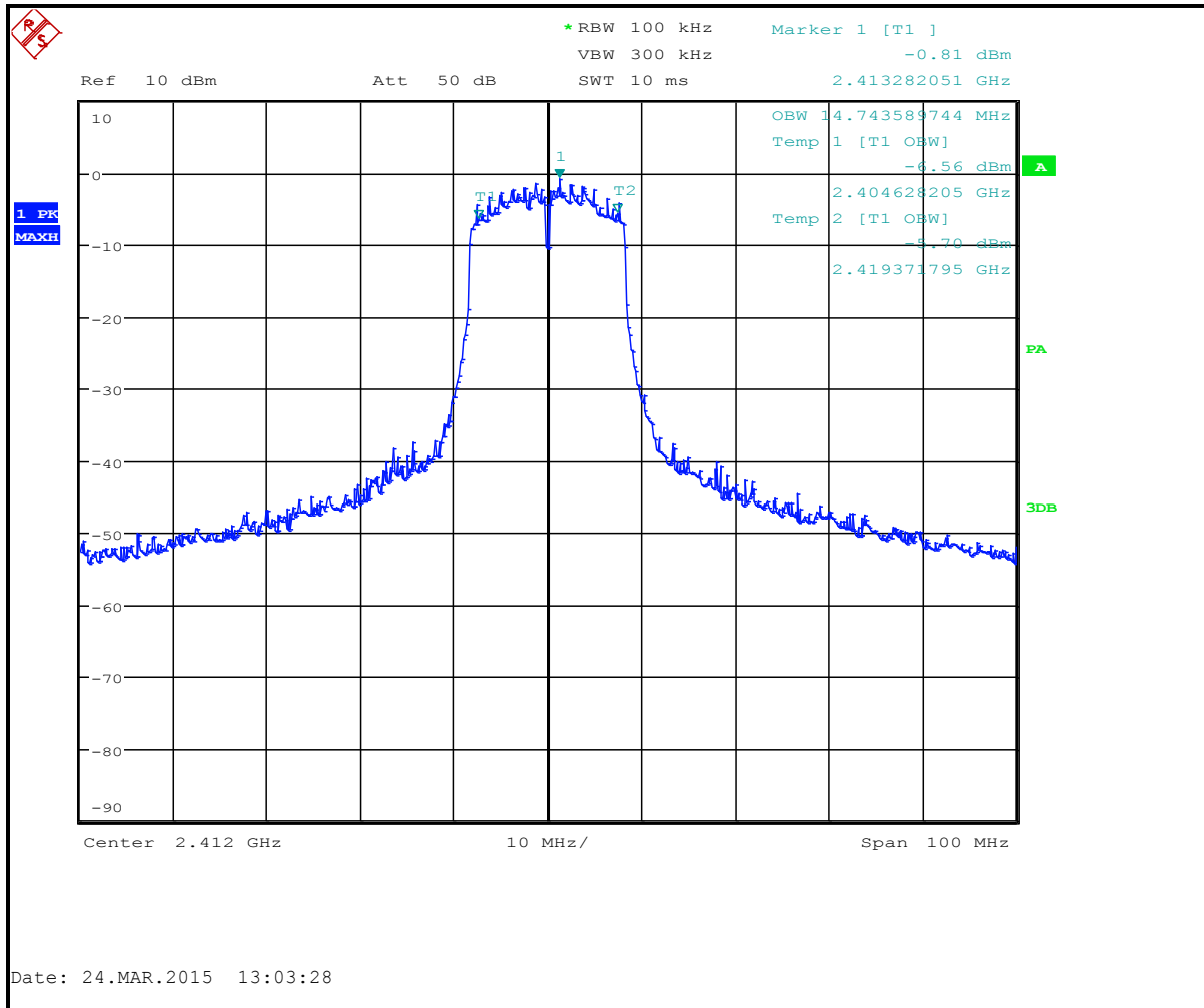
Plot 5-4: 6 dB Bandwidth Channel 1 (TX Frequency 2412 MHz) - 802.11g
