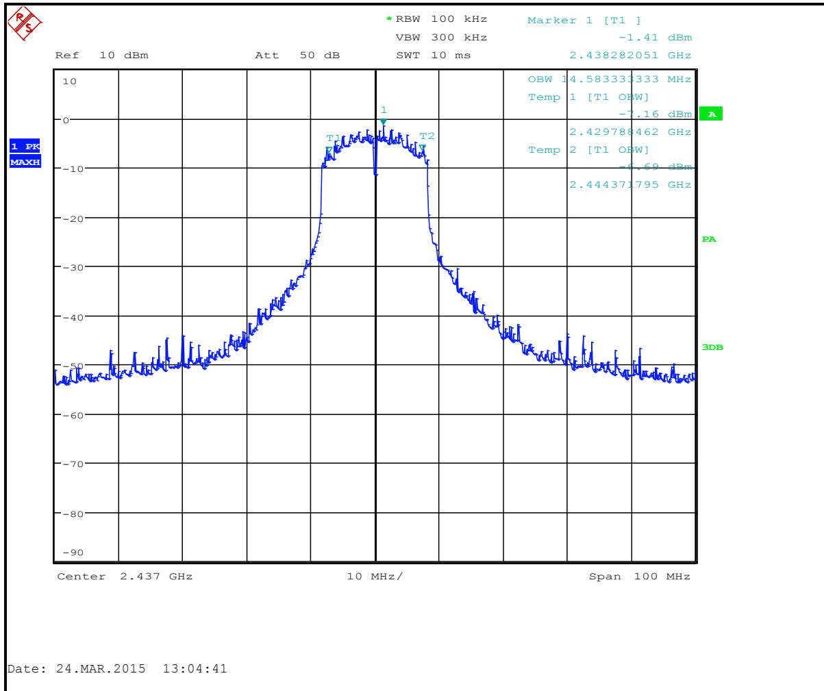
Plot 5-5: 6 dB Bandwidth Channel 6 (TX Frequency 2437 MHz) - 802.11g
