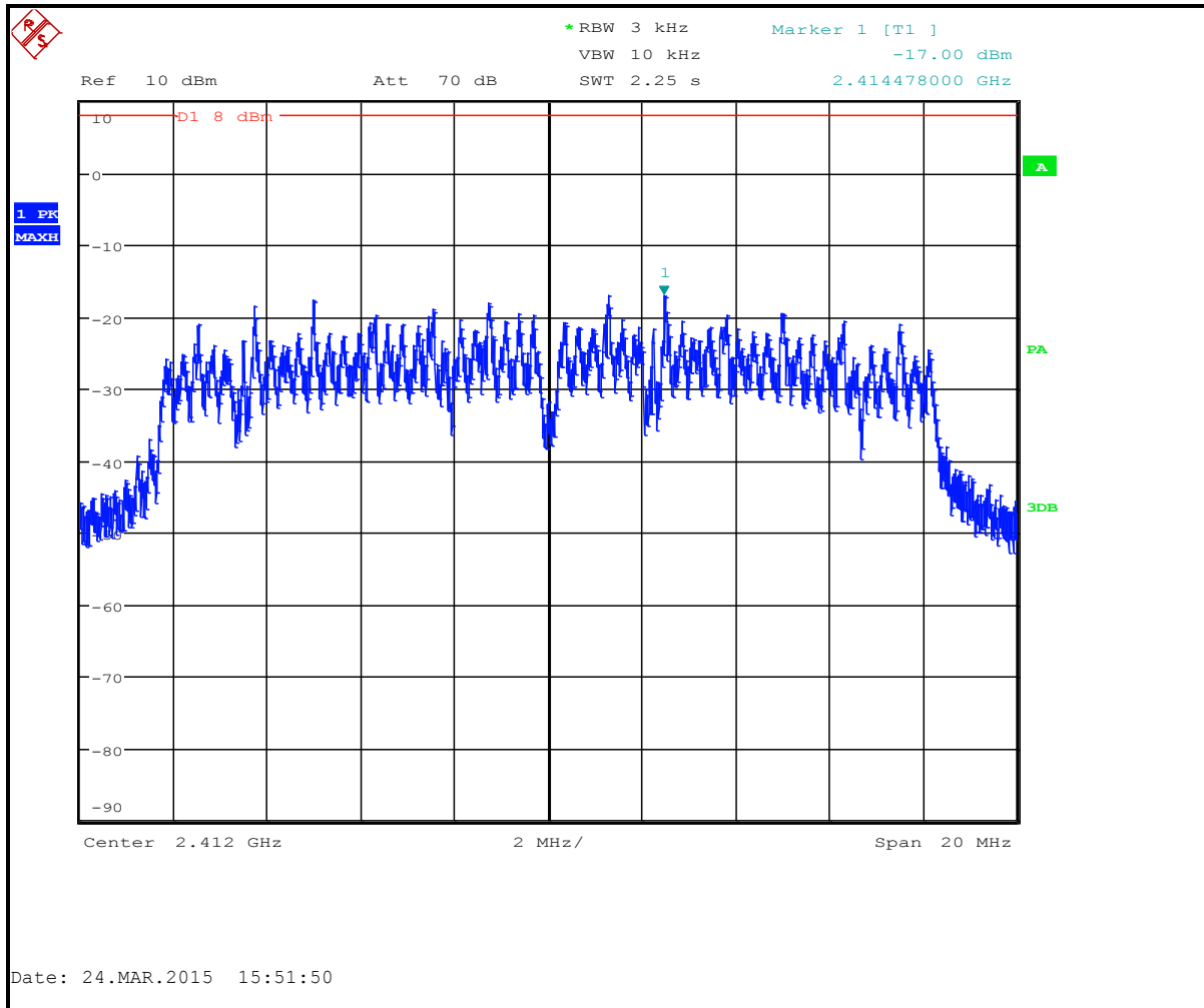
Plot 6-7: Power Spectral Density: Channel 1 (2412 MHz); 802.11n (13 Mbps)
