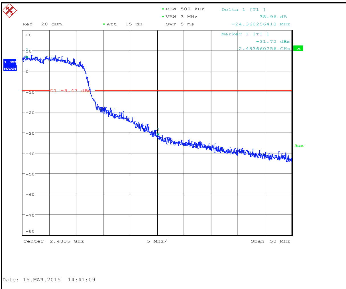
Plot 4-4: In Band Emissions - Channel 11 (2462 MHz); 802.11g (12 Mbps)
