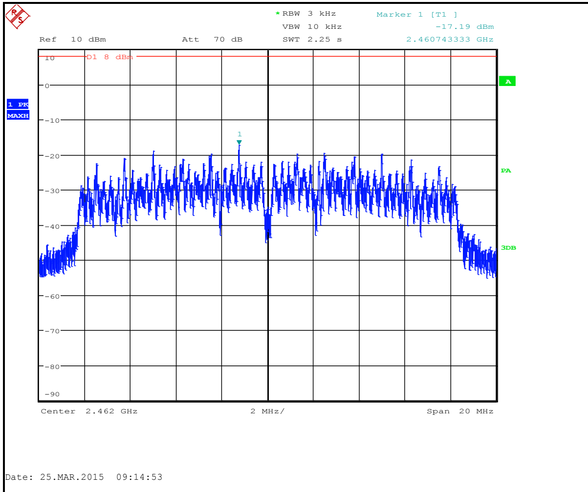
Plot 6-6: Power Spectral Density: Channel 11 (2462 MHz); 802.11g (18 Mbps)
