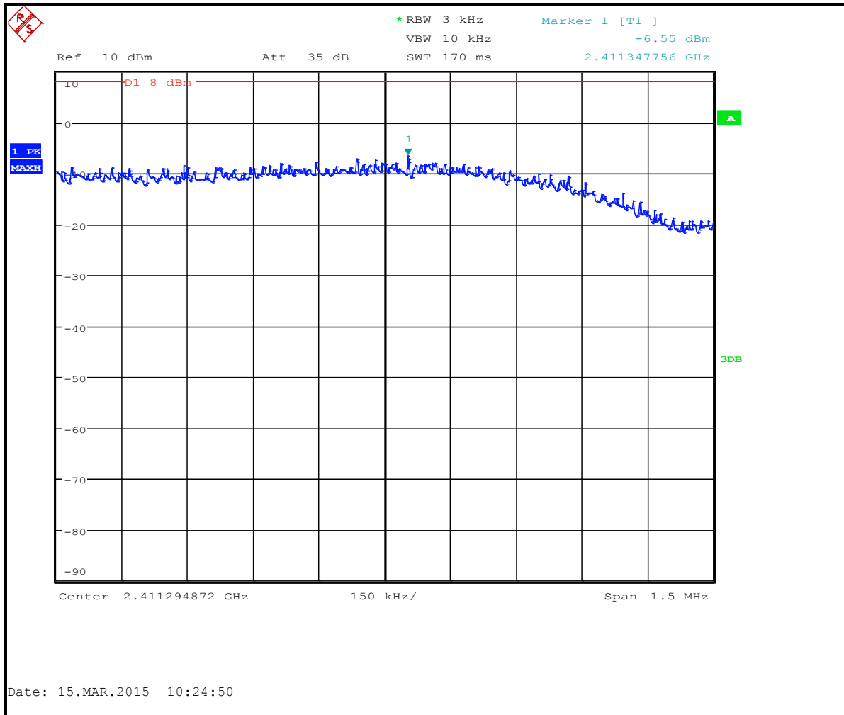
Plot 6-1: Power Spectral Density: Channel 1 (2412 MHz); 802.11b (2 Mbps)
