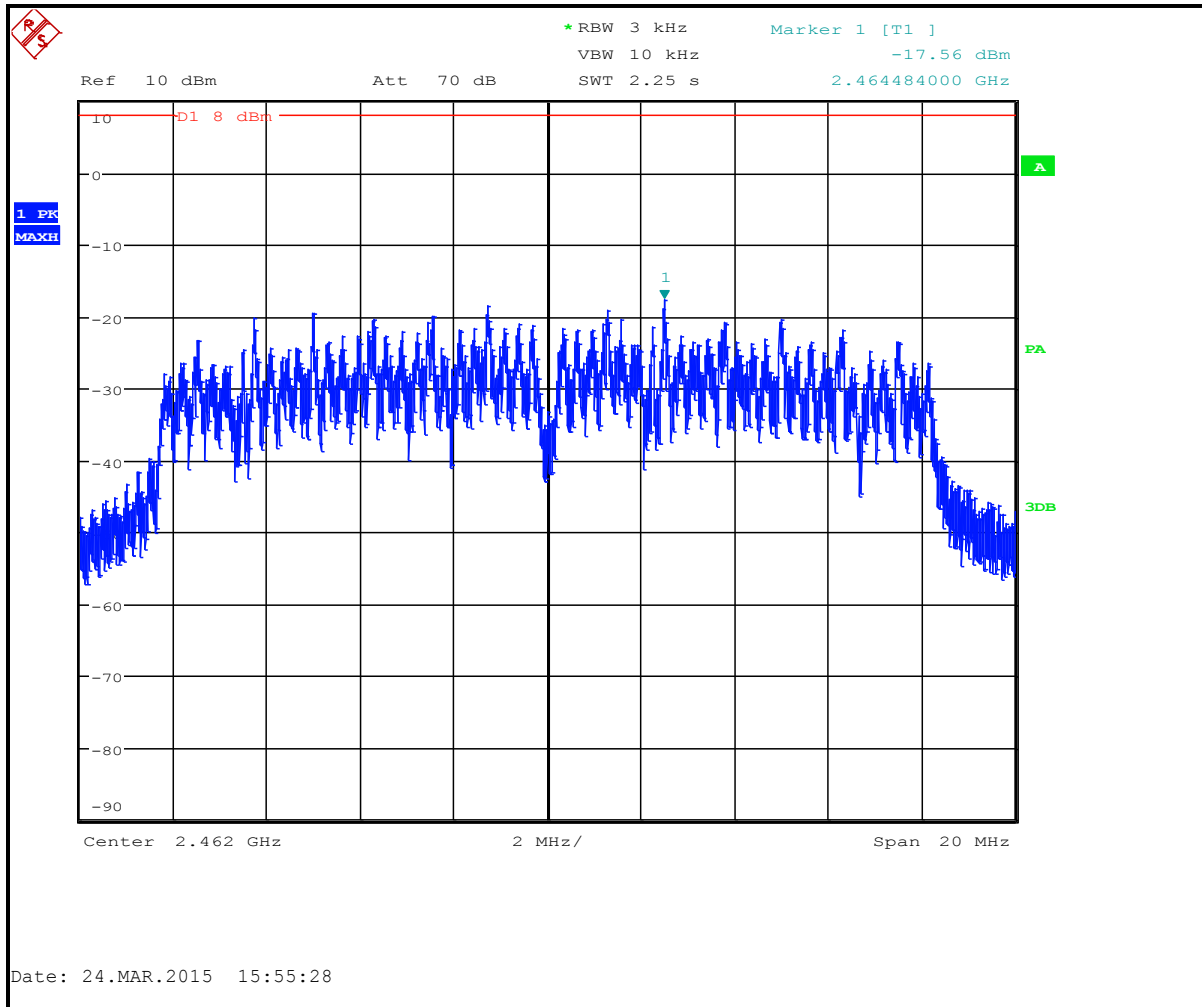
Plot 6-9: Power Spectral Density: Channel 11 (2462 MHz); 802.11n (13 Mbps)
