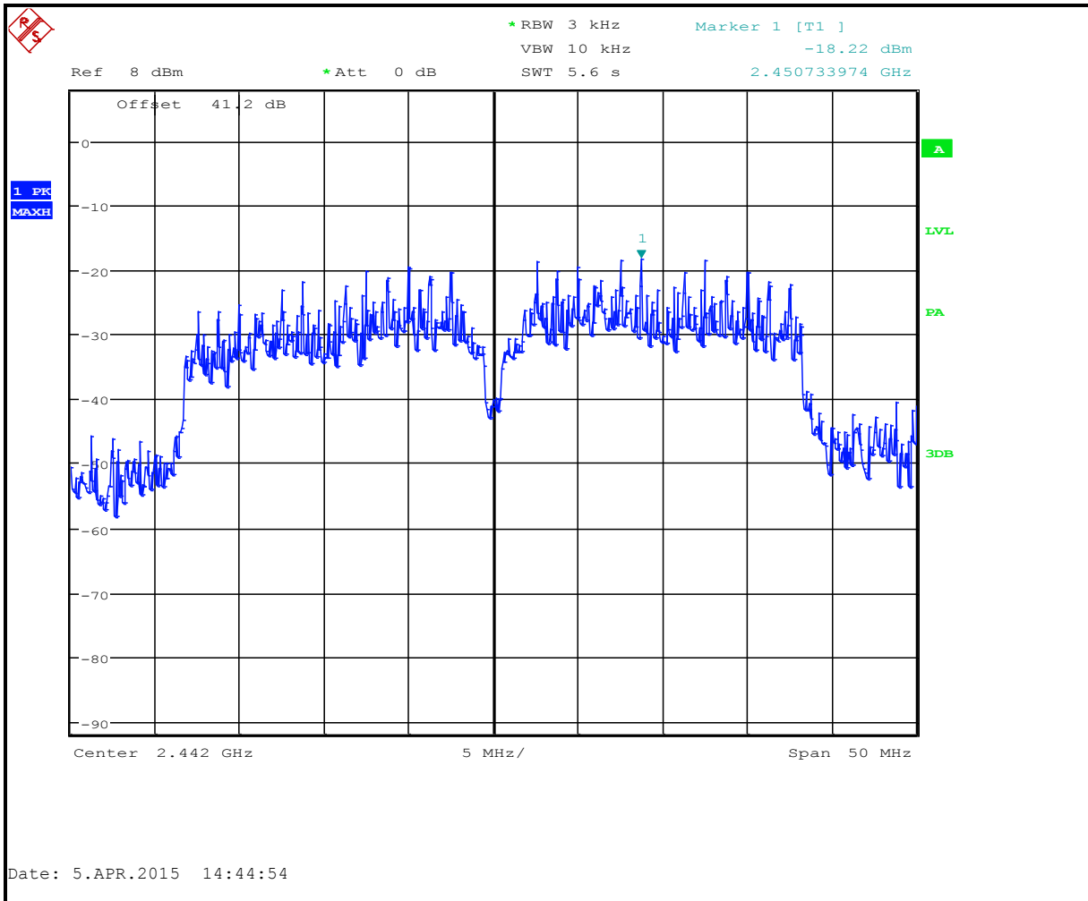
Plot 6-10: Power Spectral Density: Channel 5 (2442 MHz); 802.11n (40MHz BW)
