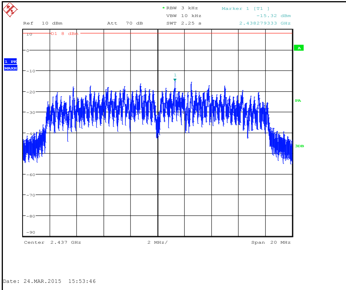
Plot 6-8: Power Spectral Density: Channel 6 (2437 MHz); 802.11n (13 Mbps)
