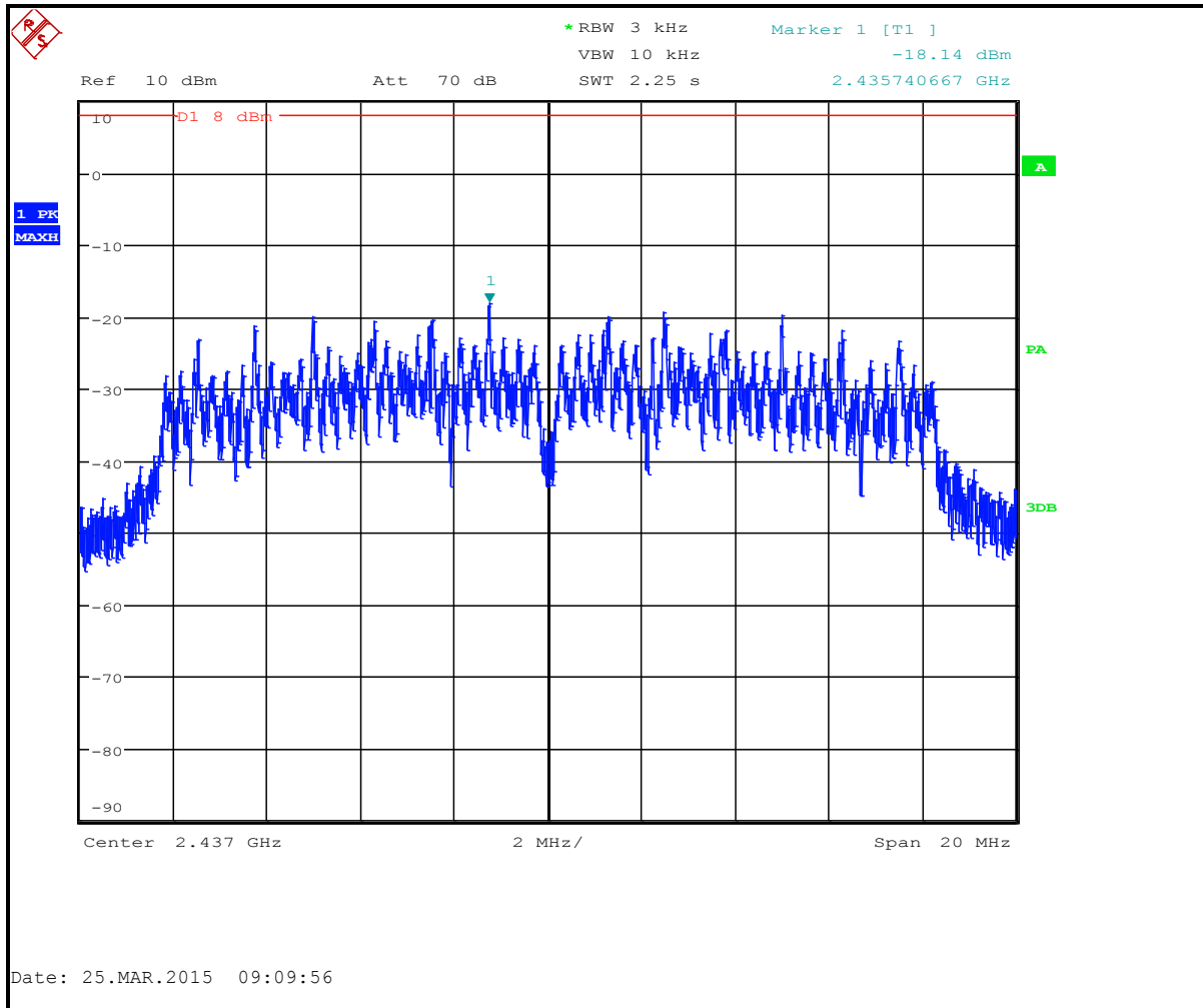
Plot 6-5: Power Spectral Density: Channel 6 (2437 MHz); 802.11g (18 Mbps)
