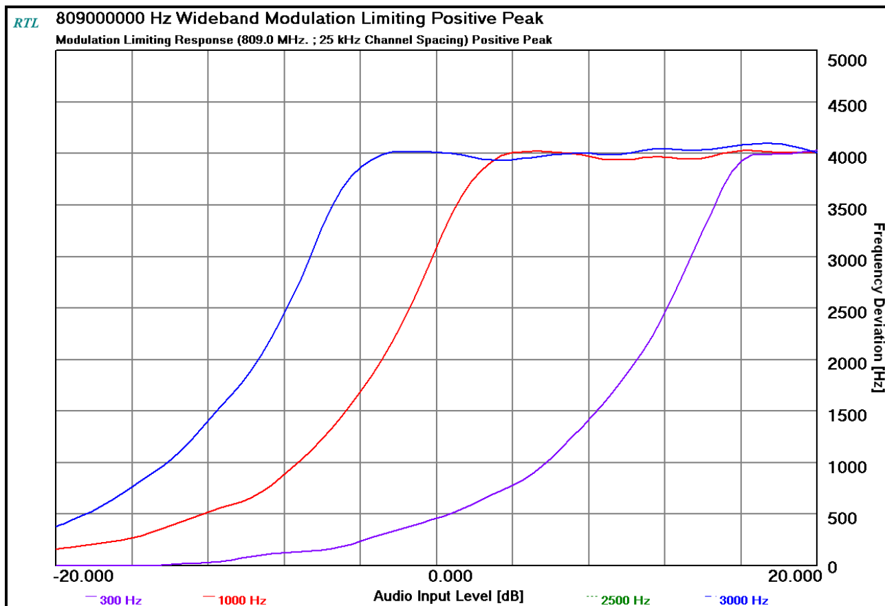
Plot 10-75: Modulation Characteristics – Modulation Limiting – 809.0000 MHz; Positive Peak; WB
