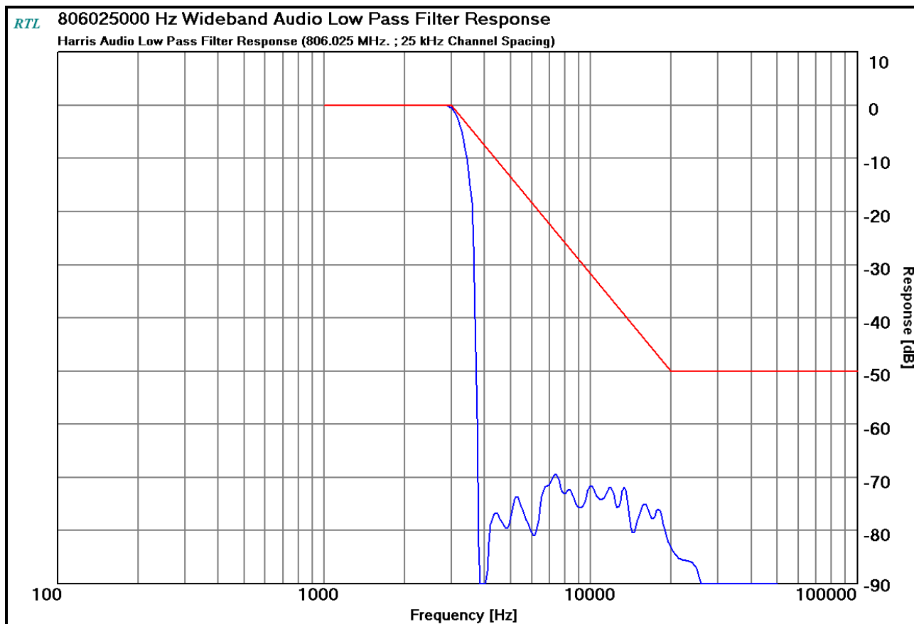
Plot 10-25: Modulation Characteristics – Audio Low Pass Filter – 806.0250 MHz
