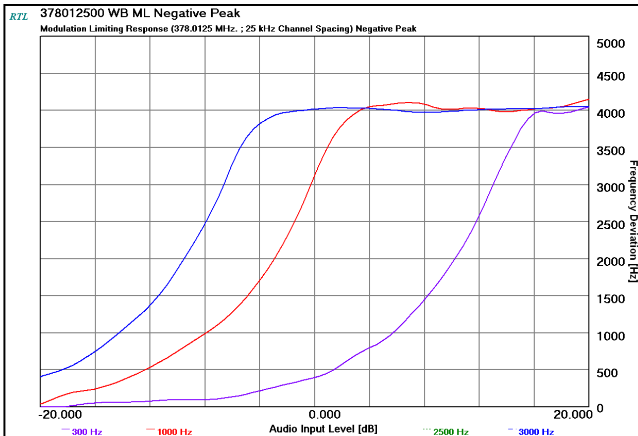
Plot 10-68: Modulation Characteristics – Modulation Limiting – 378.0125 MHz; Negative Peak; WB
