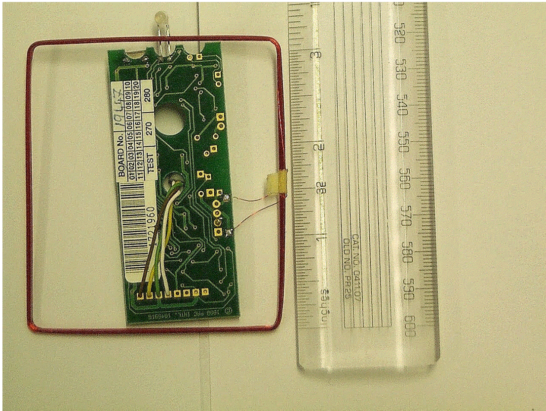
PCB Assembly (Solder side)
