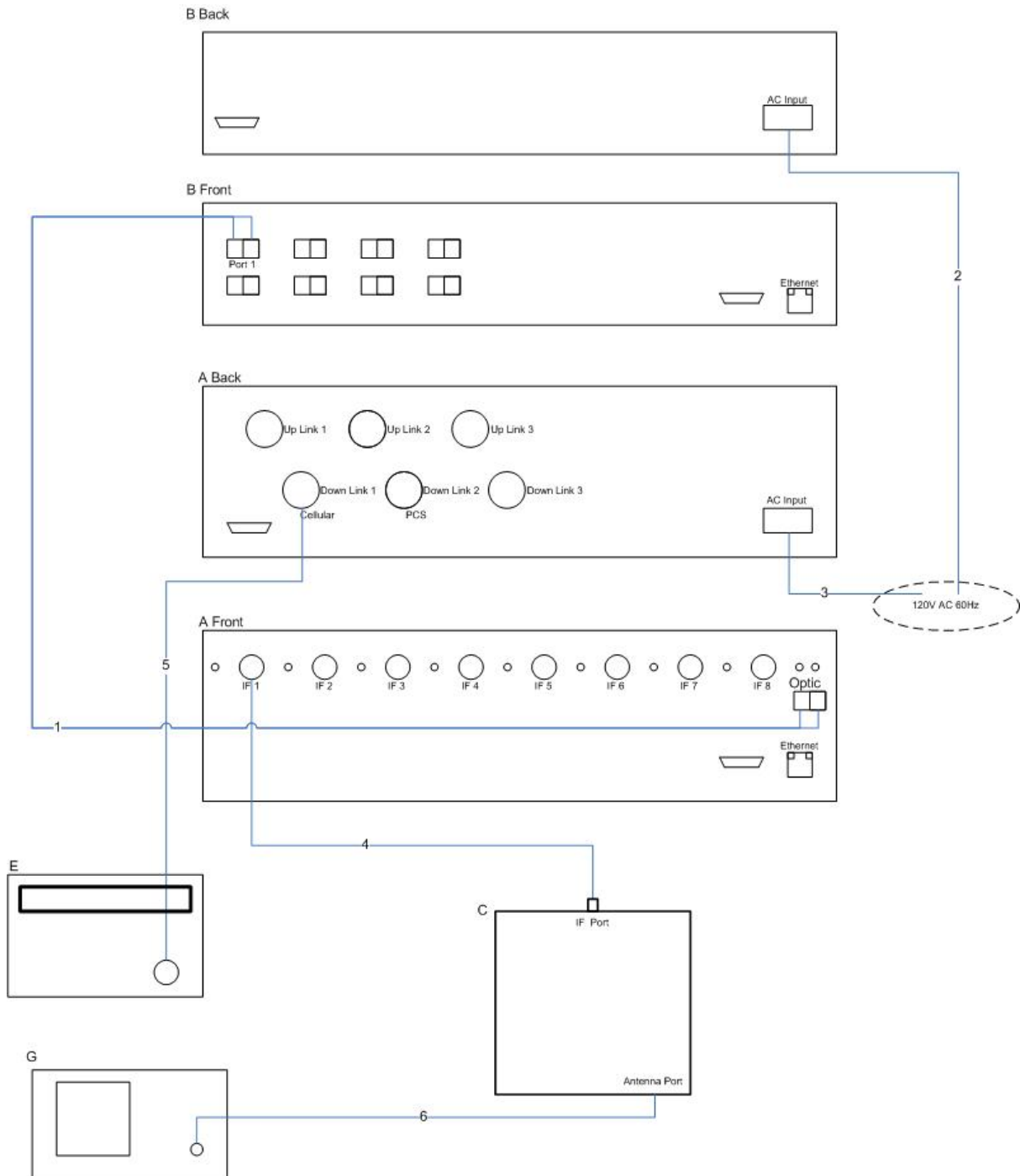
Figure 1. Block Diagram of Test Configuration (Downlink Cellular - Conducted Measurement & Frequency Stability)
