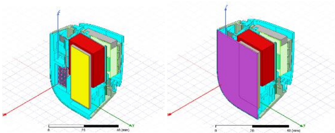
Figure C-5 Right module
