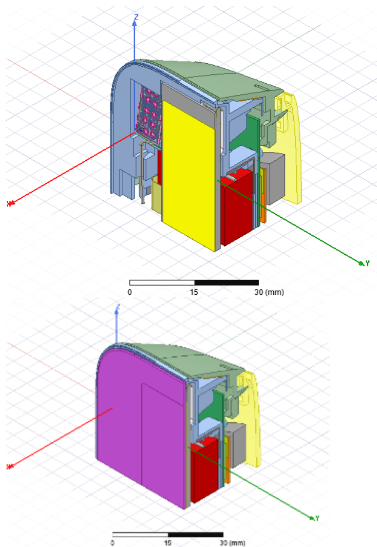
Figure C-4 Left module
