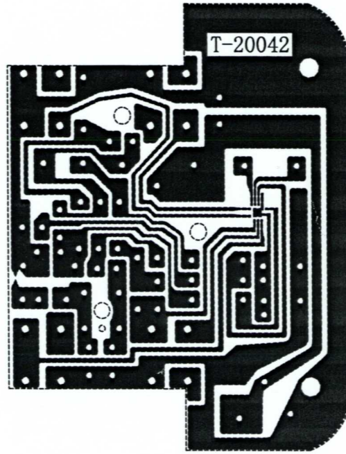
PCB Layout Diagram
