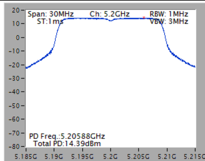
5150-5250MHz - Worst Power Spectral Density Plots
