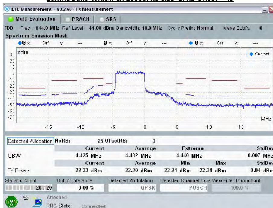
10MHz Band Width: Ch 20600, RB Size=25; RB Offset = 0
