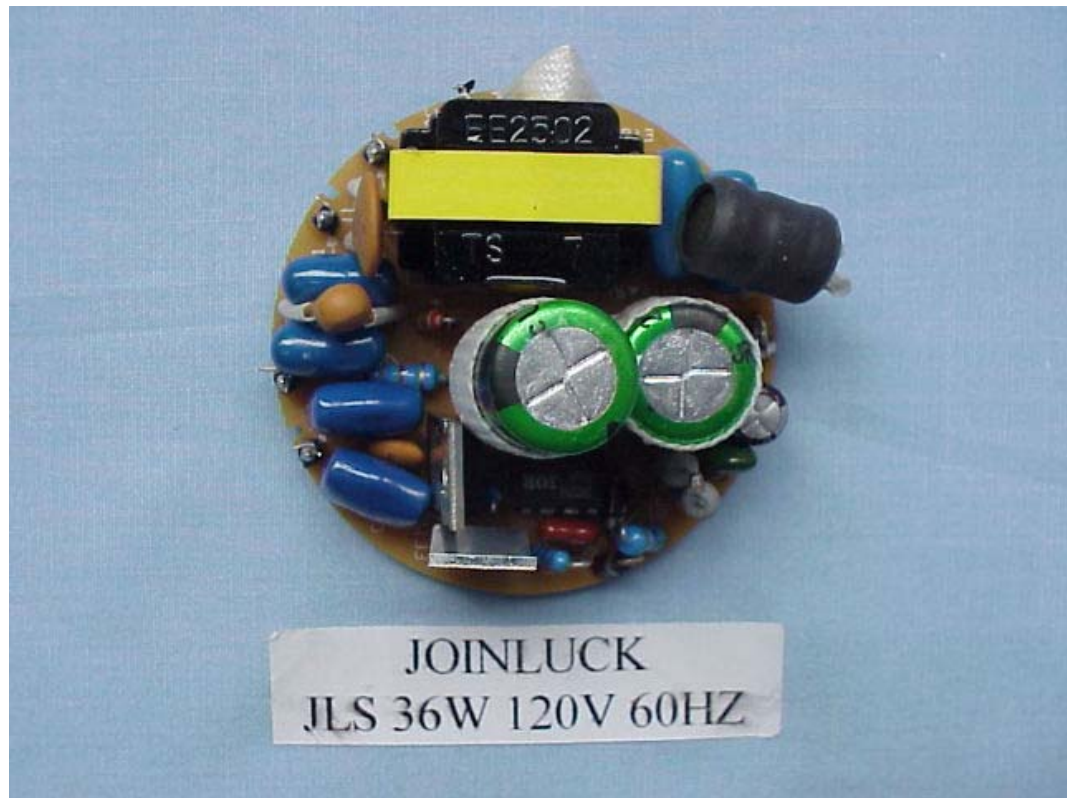
FIGURE 5 ENERGY SAVING LAMP (M/N: JLS 36W) MAIN BOARD (COMPONENT SIDE)
