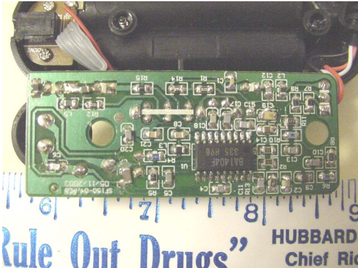
RF Main Board Bottom View and Component View of Connector Board
