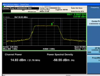
Antenna D
