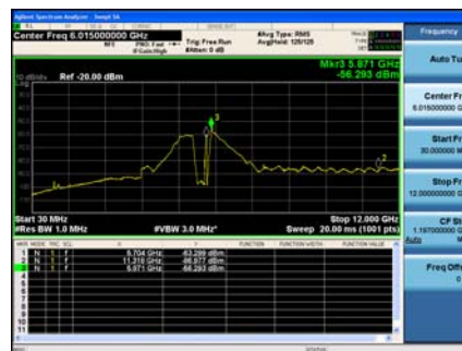
Antenna B
