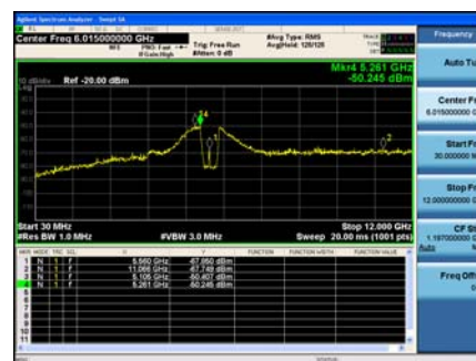
Antenna D
