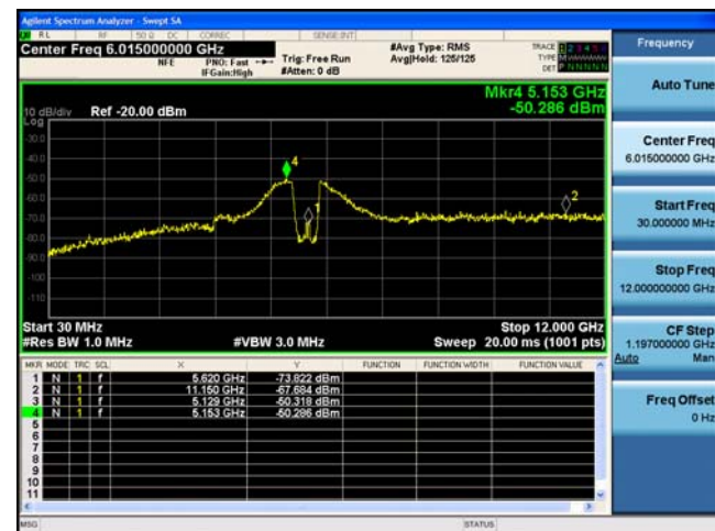
Antenna D
