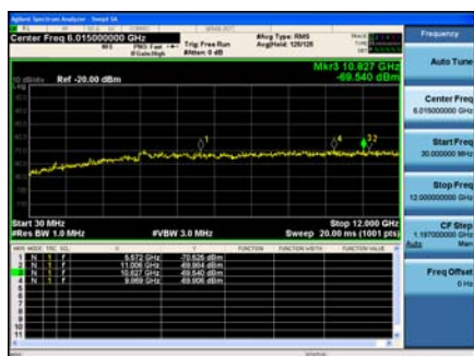
Antenna C
