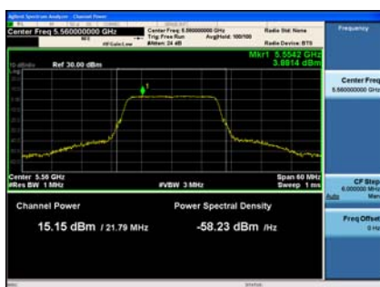
Antenna C
