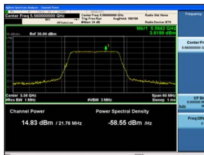
Antenna D
