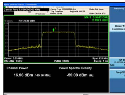
Antenna B
