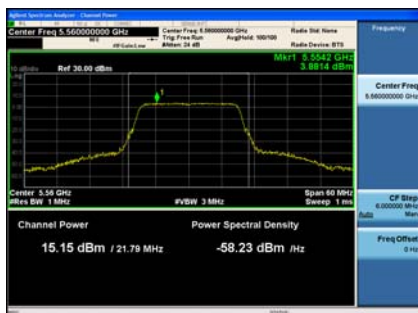
Antenna C
