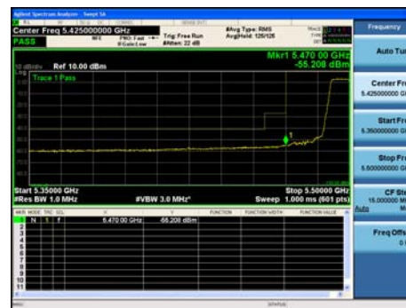
Antenna D
