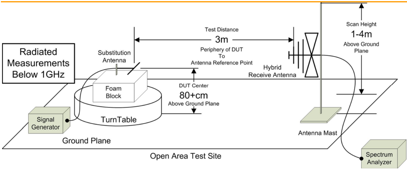
Figure A.4 – Test Setup Radiated Emissions Measurements 30 – 1000MHz Signal Substitution
