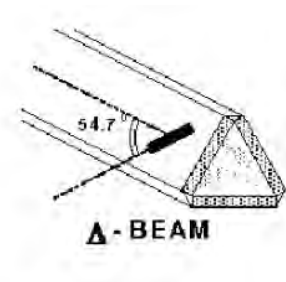
Figure 2.2 Triangular Probe Configurations
