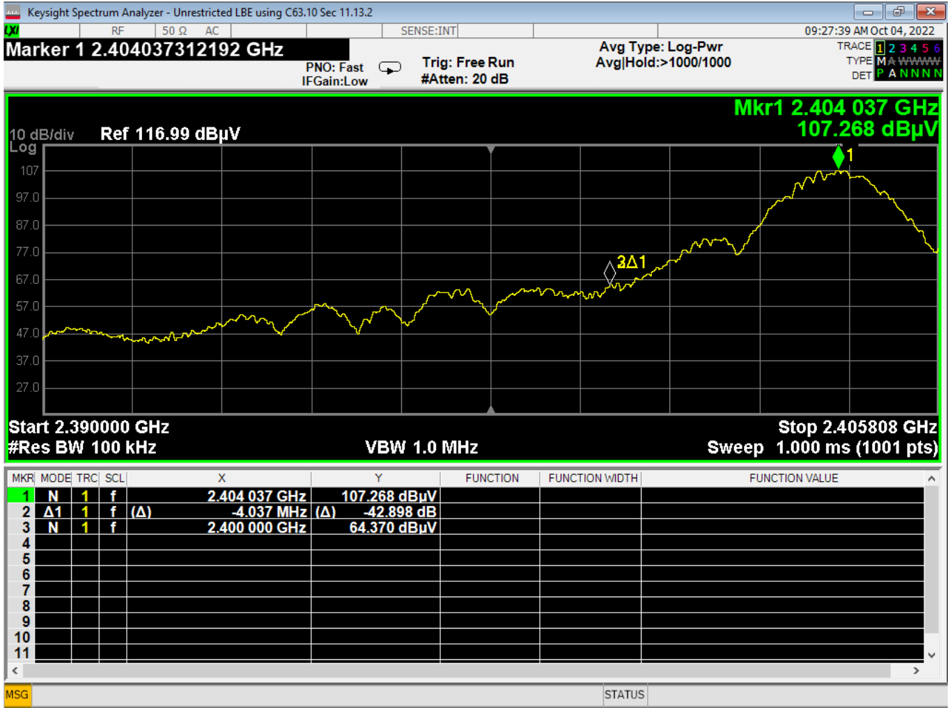
36 Lower Bandedge, Unrestricted, GMSK 2MB
