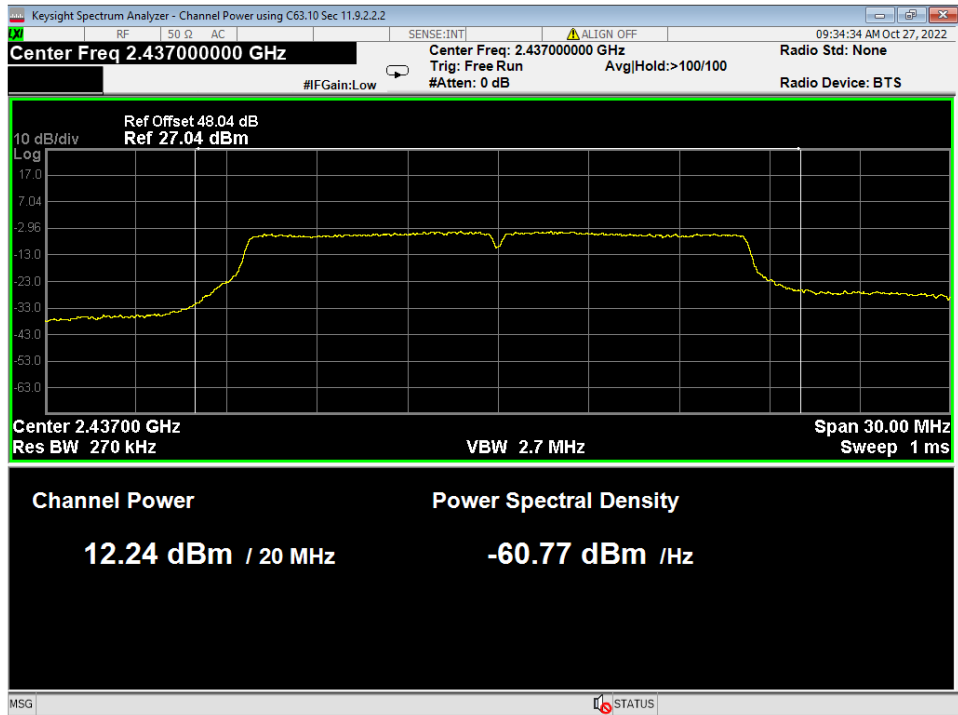
Figure 22 – Radiated Average Power Measurement, 802.11g 6MB Reference offset includes EIRP conversion and corrections
