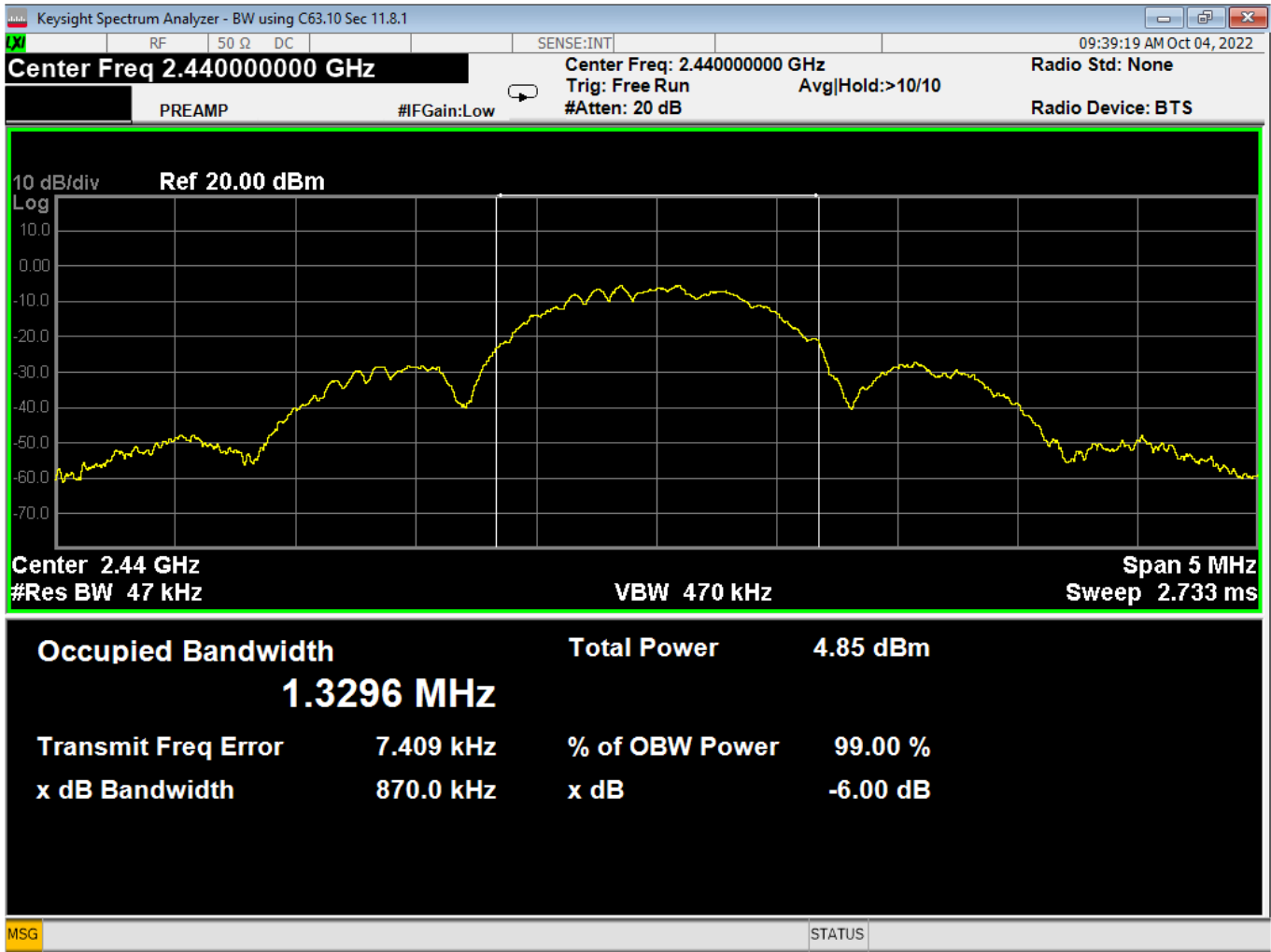
41 Occupied Bandwidth, Mid Channel, GFSK
