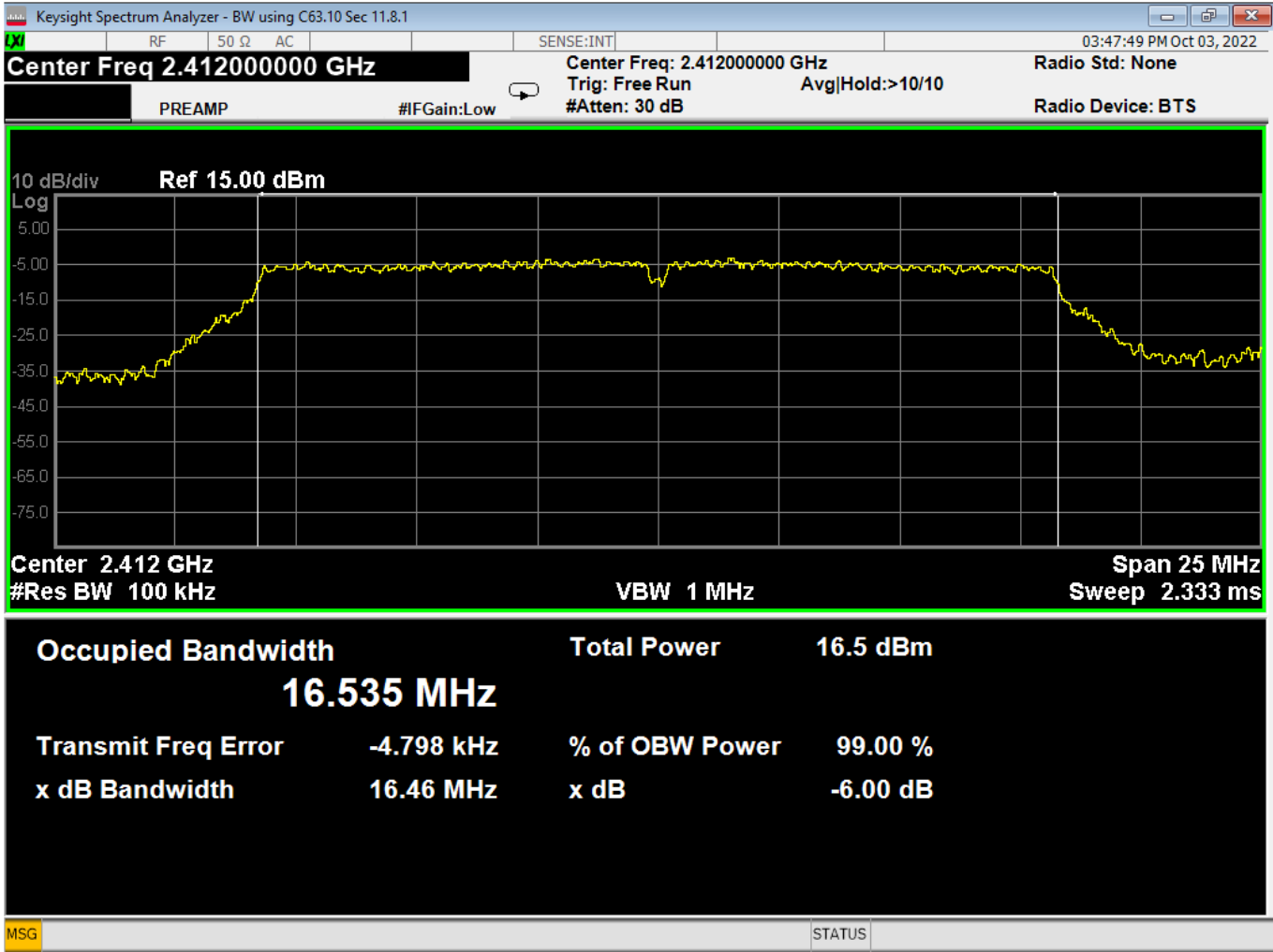
82 6dB Bandwidth, Low, Wifi G, Low Data Rate
