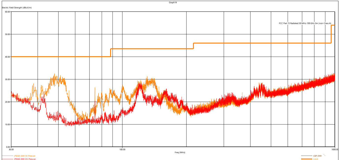
Figure 32 - Radiated Emissions Plot, 802.11n, High Data Rate
