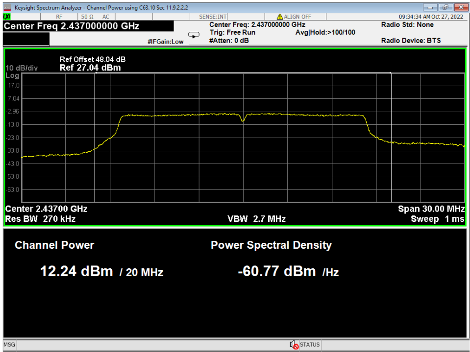
Figure 34 – Radiated Average Power Measurement, 802.11g 6MB Reference offset includes EIRP conversion and corrections
