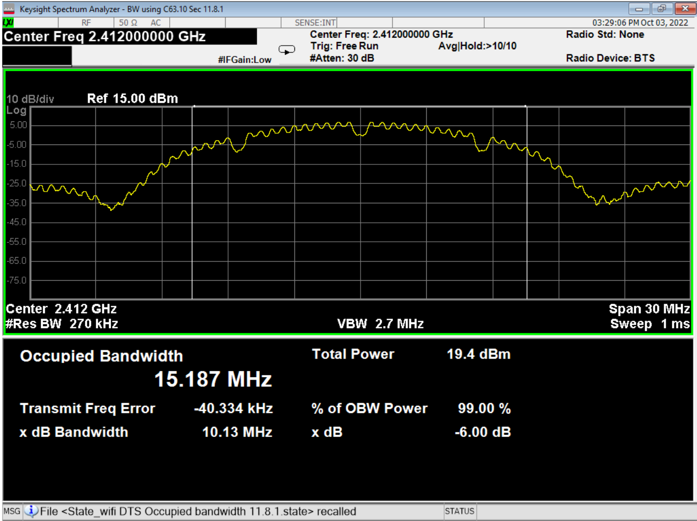
04 Bandwidth, Low, Wifi B, Low Data Rate
