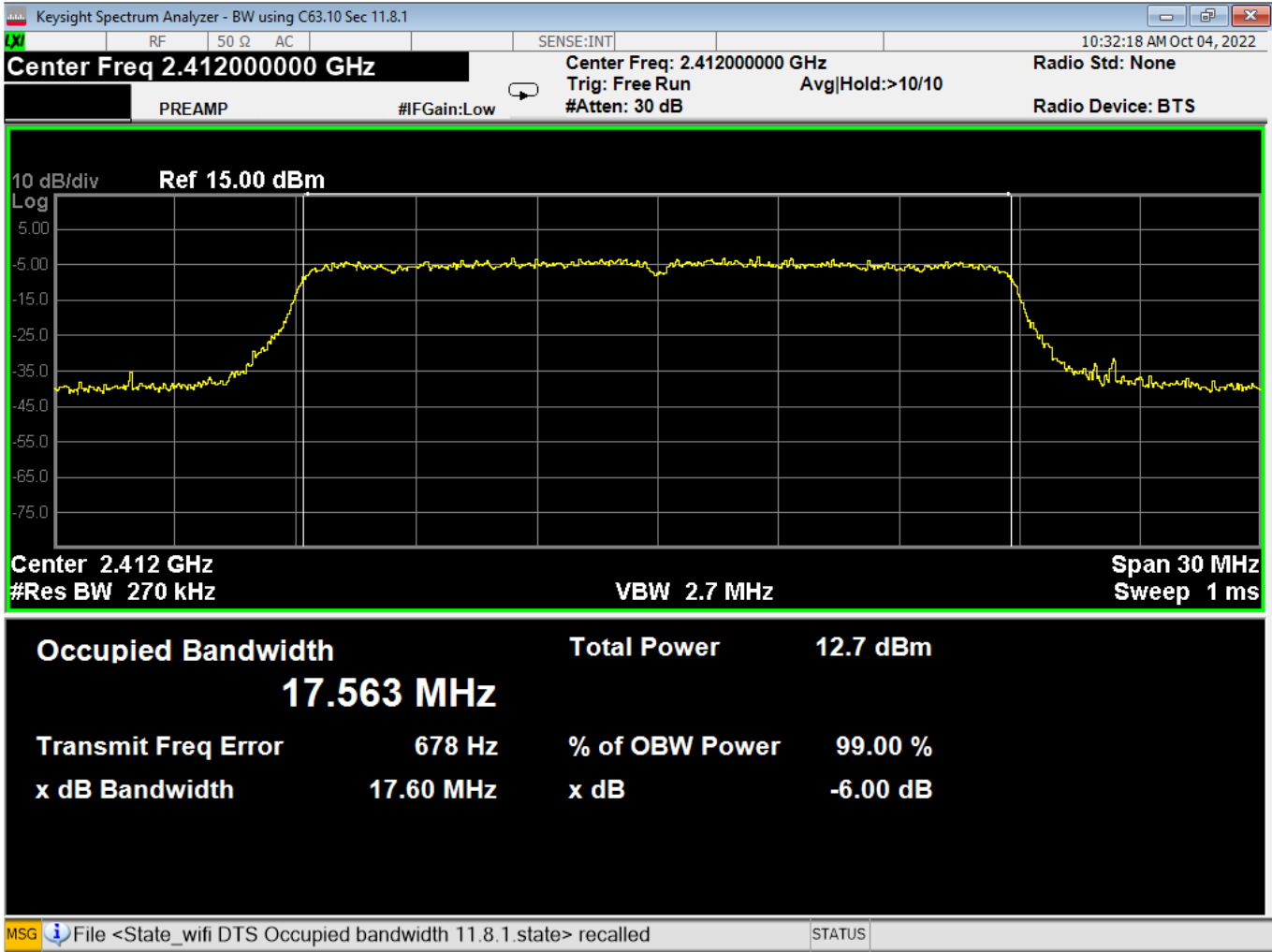
69 Bandwidth, Low, Wifi N, High Data Rate
