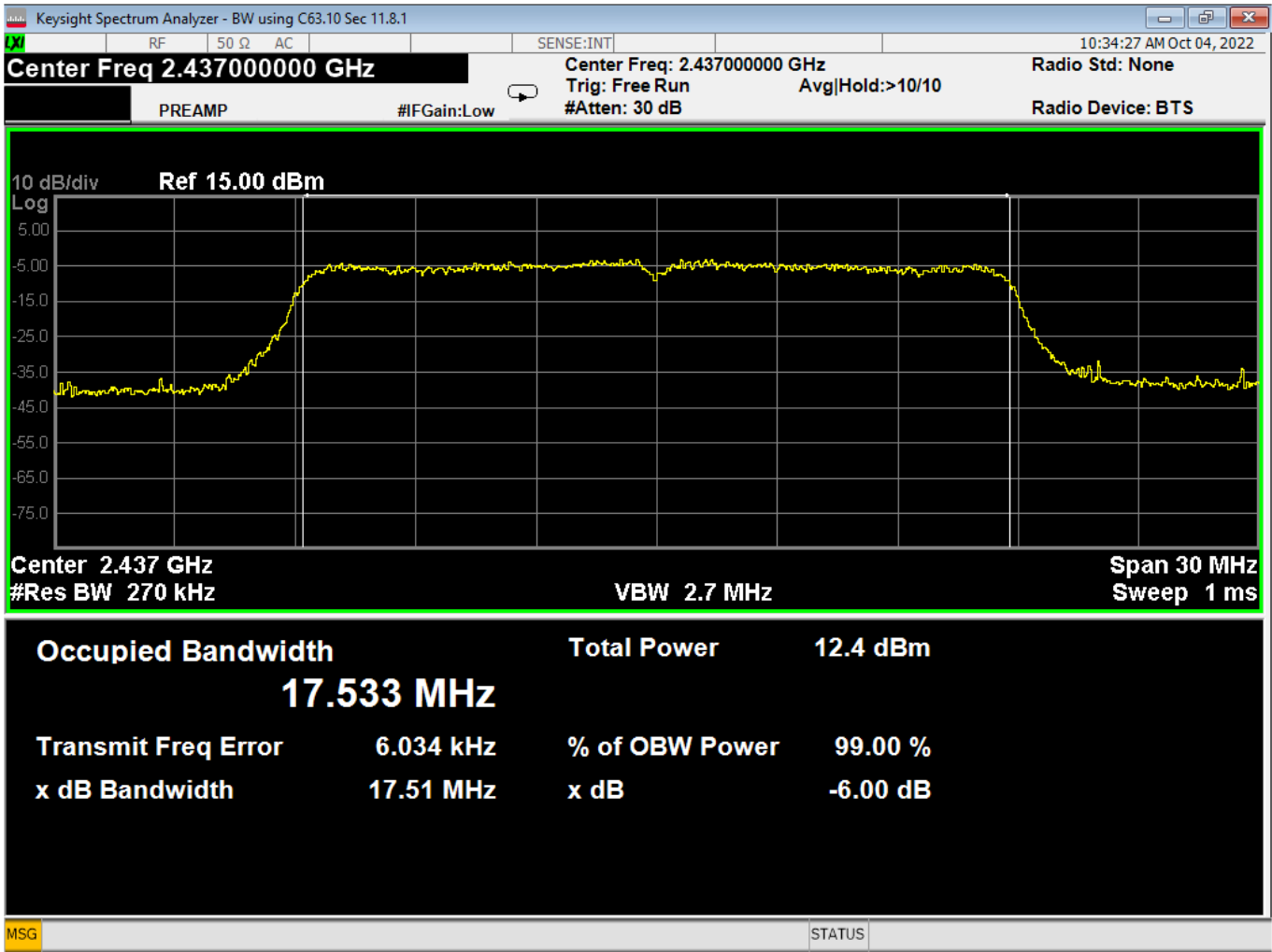
70 Bandwidth, Mid, Wifi N, High Data Rate
