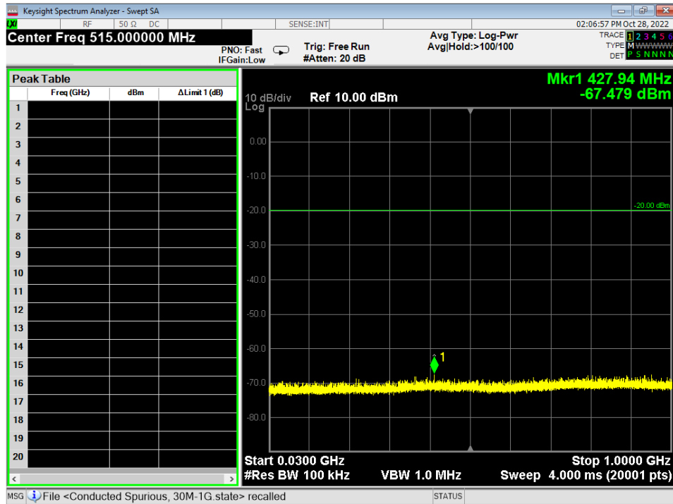
Figure 18 - Conducted Emissions Plot, Wifi N MCS7, 30M – 1G
