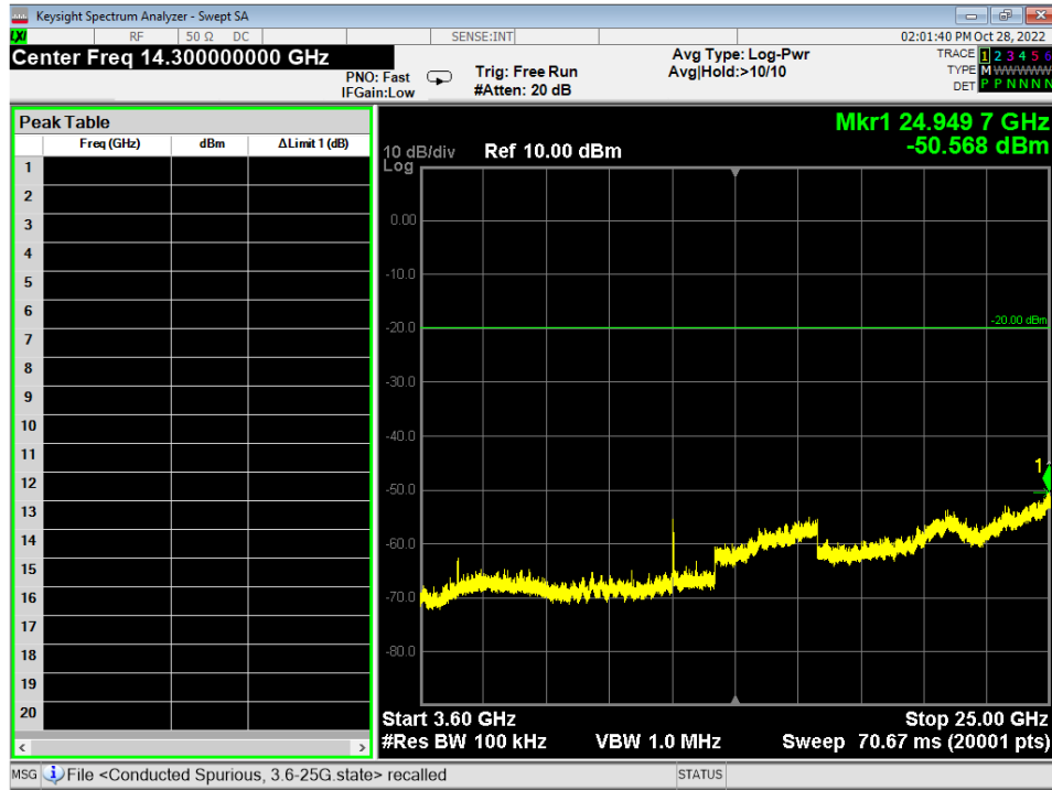
Figure 17 - Conducted Emissions Plot, Wifi G 54MB, 3.6G – 25G
