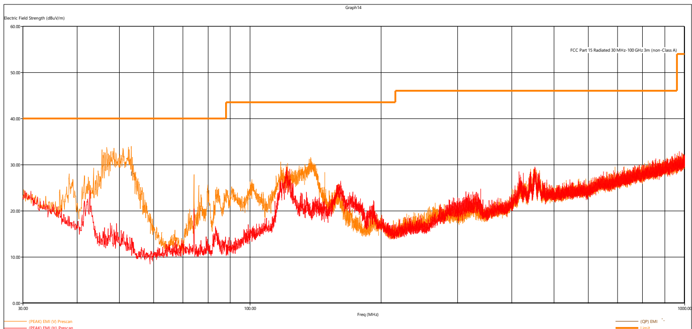
Figure 31 - Radiated Emissions Plot, 802.11g, High Data Rate
