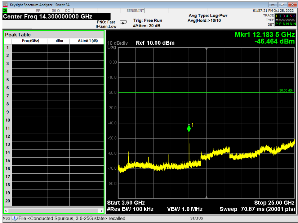
Figure 14 - Conducted Emissions Plot, Wifi B 11MB, 3.6G – 25G
