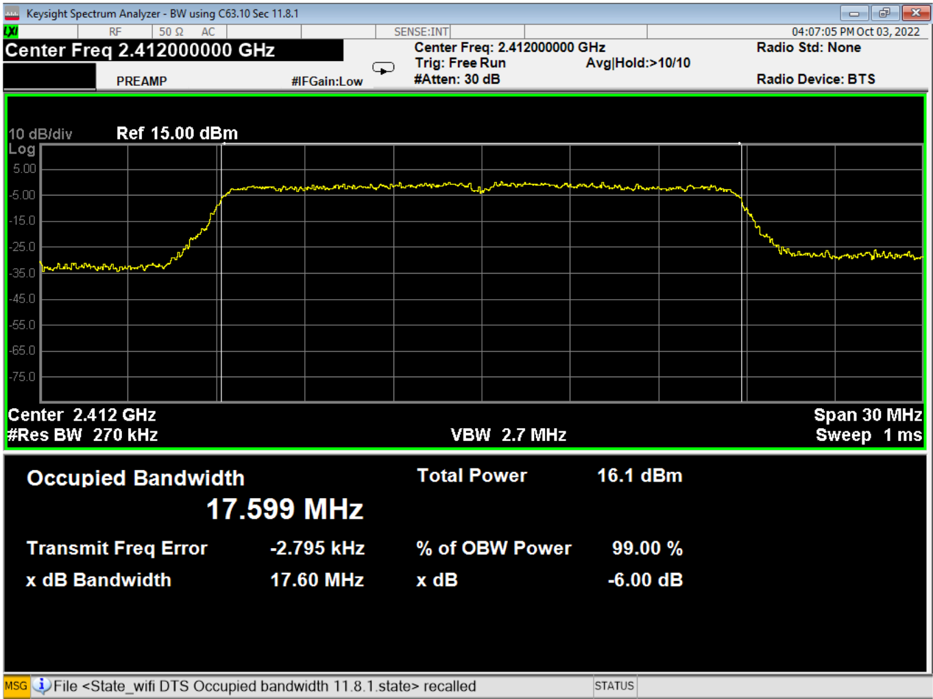
30 Bandwidth, Low, Wifi N, Low Data Rate
