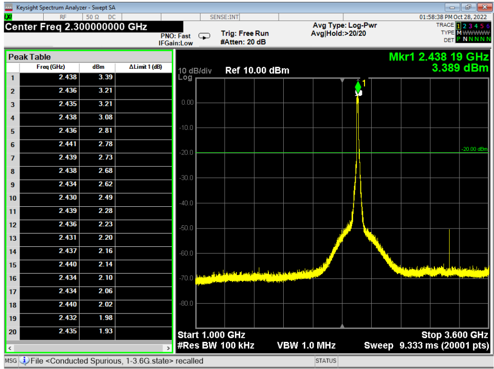
Figure 13 - Conducted Emissions Plot, Wifi B 11MB, 1G – 3.6G
