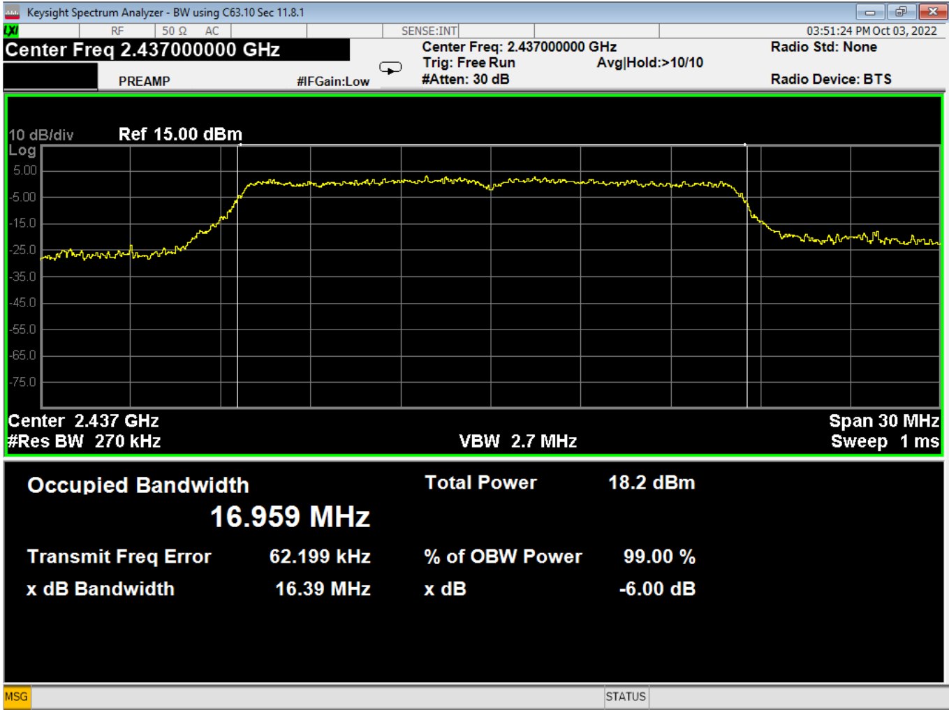
18 Bandwidth, Mid, Wifi G, Low Data Rate
