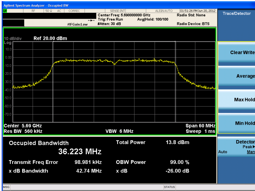
Plot 6-25. 26dB Bandwidth Plot (40MHz BW 802.11n (UNII Band 3) – Ch. 138)
