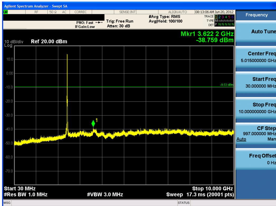
Plot 6-57. Conducted Spurious Plot (802.11b – Ch. 6)
