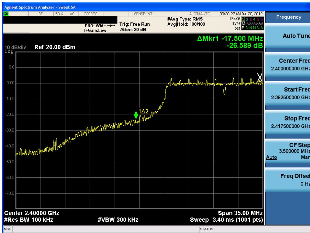
Plot 6-41. Band Edge Plot (802.11g– Ch. 1)
