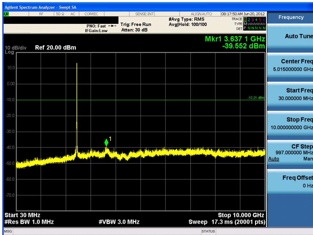
Plot 6-59. Conducted Spurious Plot (802.11b – Ch. 11)
