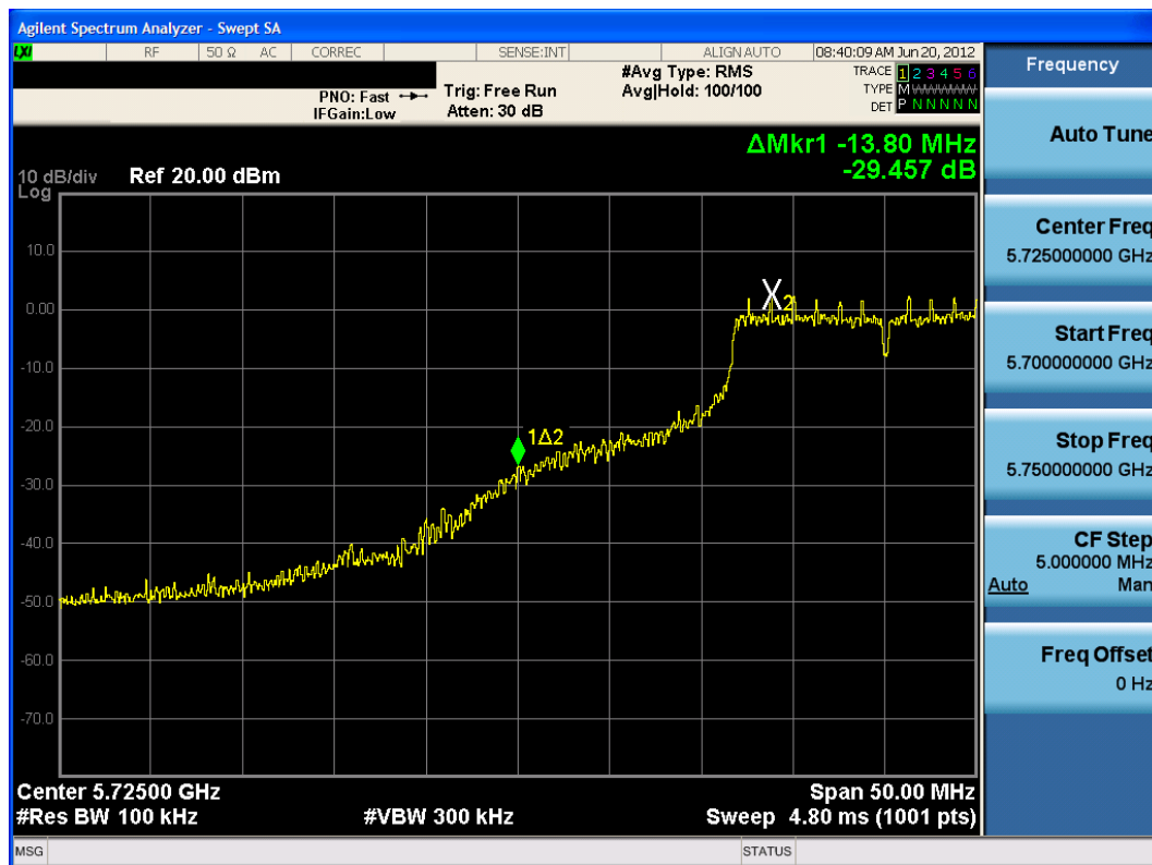
Plot 6-49. Band Edge Plot (802.11a – Ch. 149)
