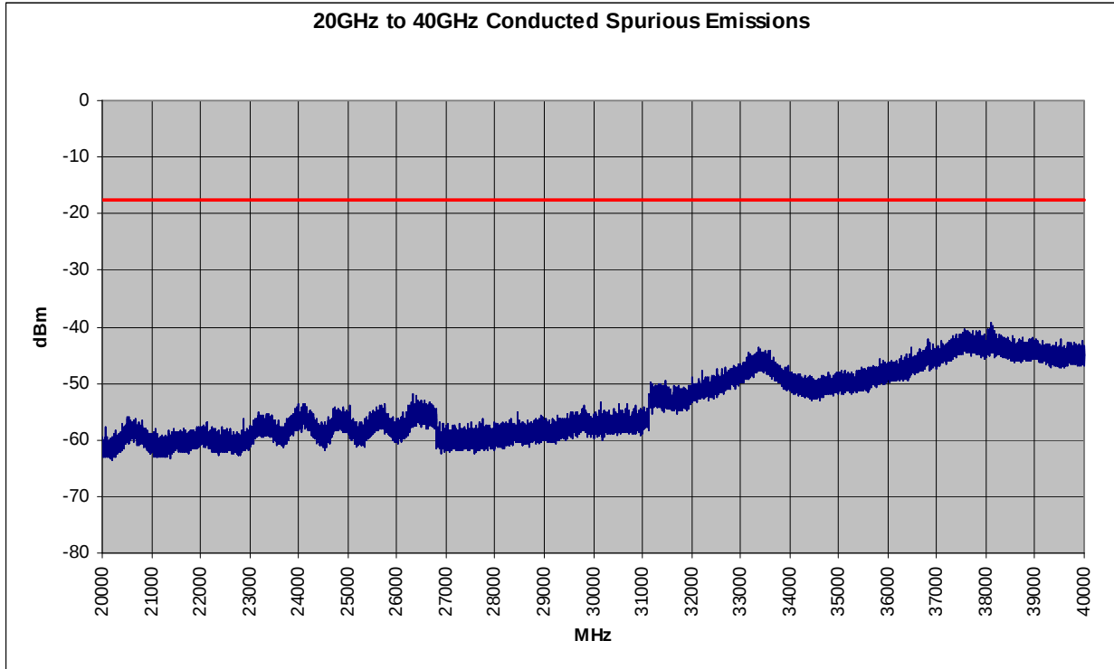
Plot 6-62. Conducted Spurious Plot (802.11a – Ch. 149)
