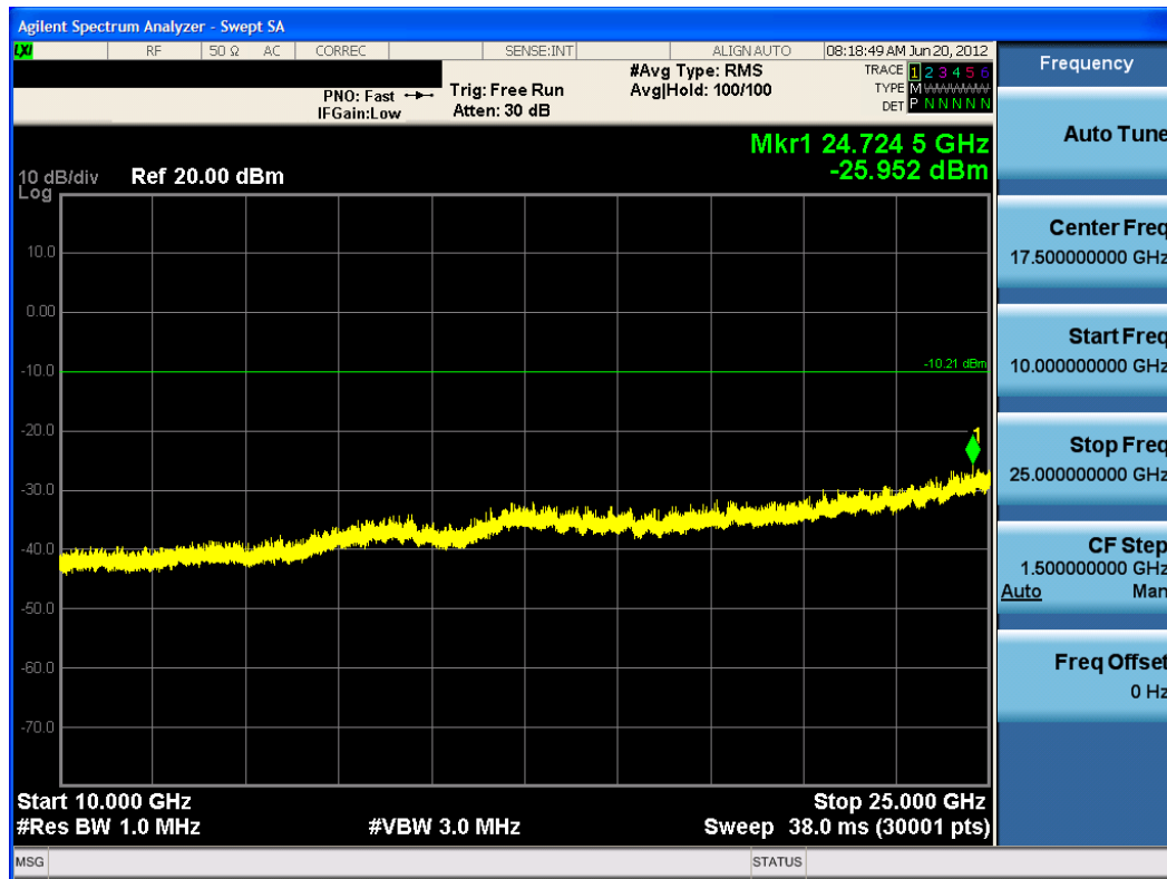
Plot 6-60. Conducted Spurious Plot (802.11b – Ch. 11)
