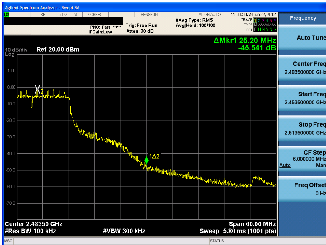
Plot 6-47. Band Edge Plot with Un-Reduced Power (802.11n (2.4GHz) – Ch. 10)
