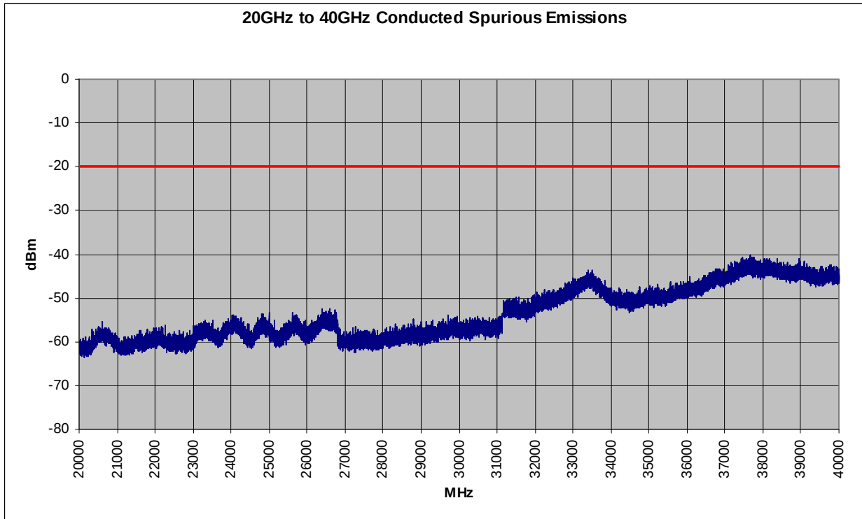
Plot 6-66. Conducted Spurious Plot (802.11a – Ch. 165)
