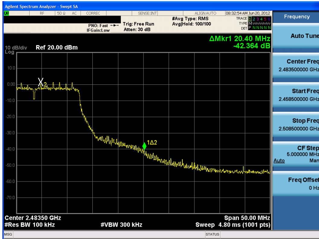
Plot 6-48. Band Edge Plot (802.11n (2.4GHz) – Ch. 11)
