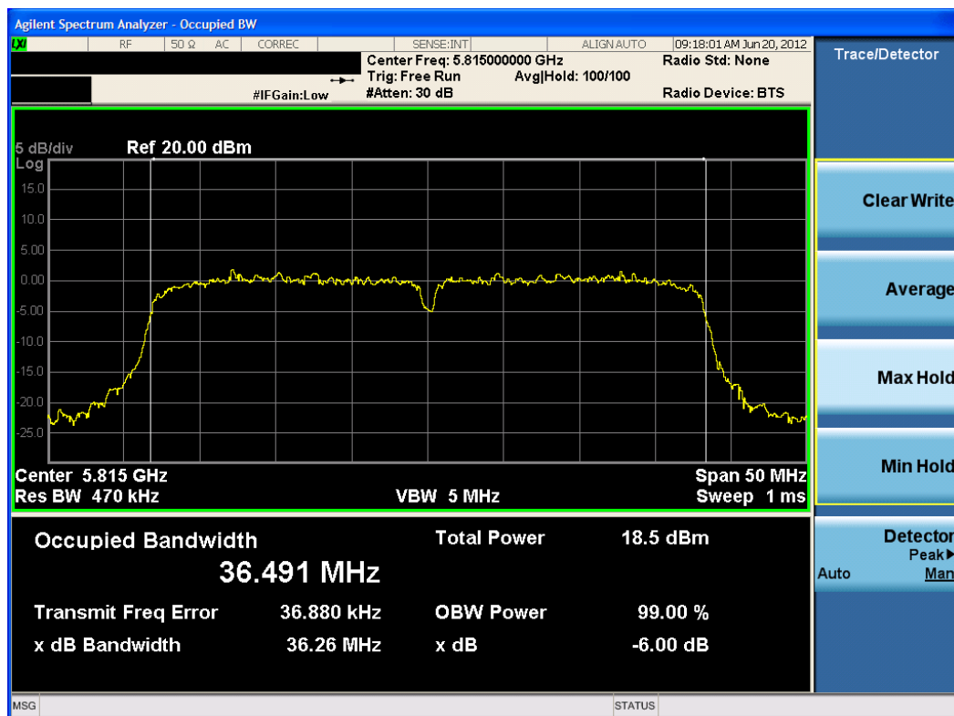
Plot 6-18. 6dB Bandwidth Plot (40MHz BW 802.11n (5.8GHz) – Ch. 163)
