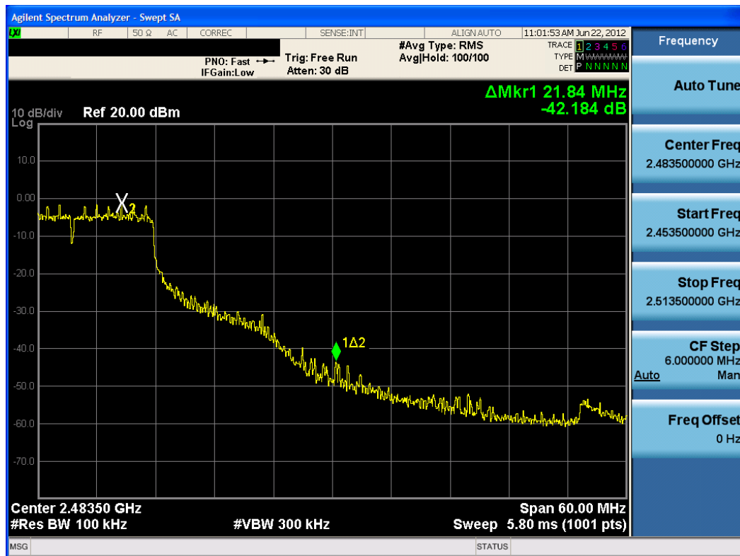
Plot 6-43. Band Edge Plot with Un-Reduced Power (802.11g – Ch. 10)
