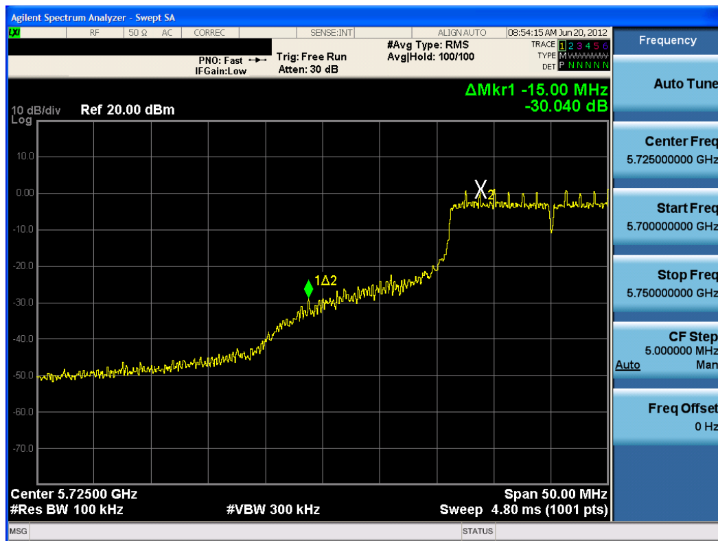
Plot 6-51. Band Edge Plot (20MHz BW 802.11n (5.8GHz) – Ch. 149)
