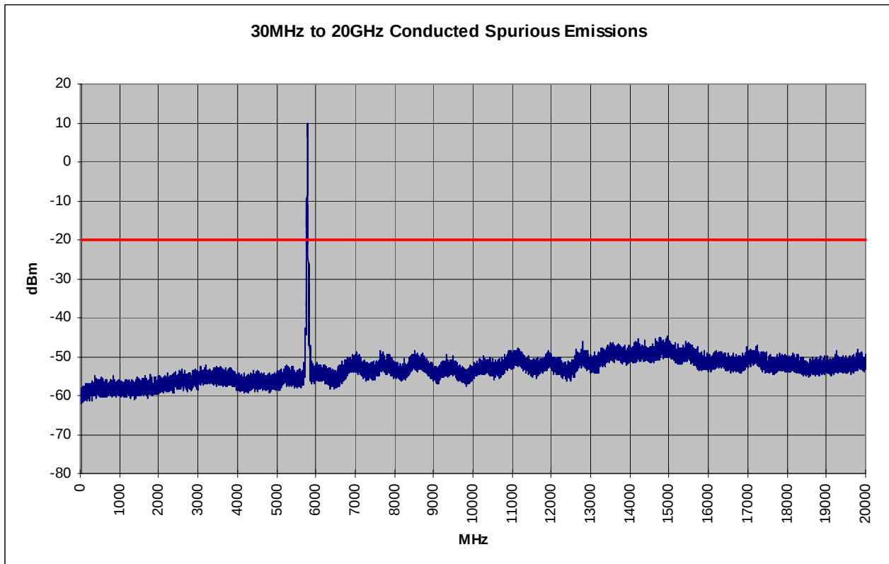
Plot 6-63. Conducted Spurious Plot (802.11a – Ch. 157)
