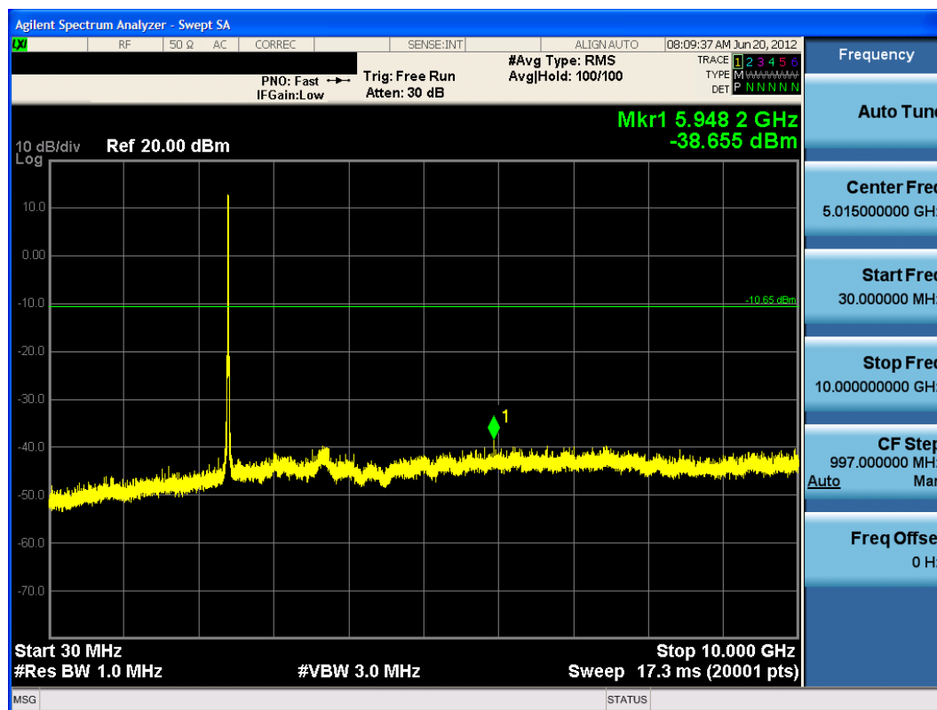
Plot 6-55. Conducted Spurious Plot (802.11b – Ch. 1)
