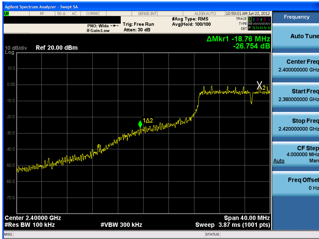
Plot 6-42. Band Edge Plot with Un-Reduced Power (802.11g – Ch. 2)
