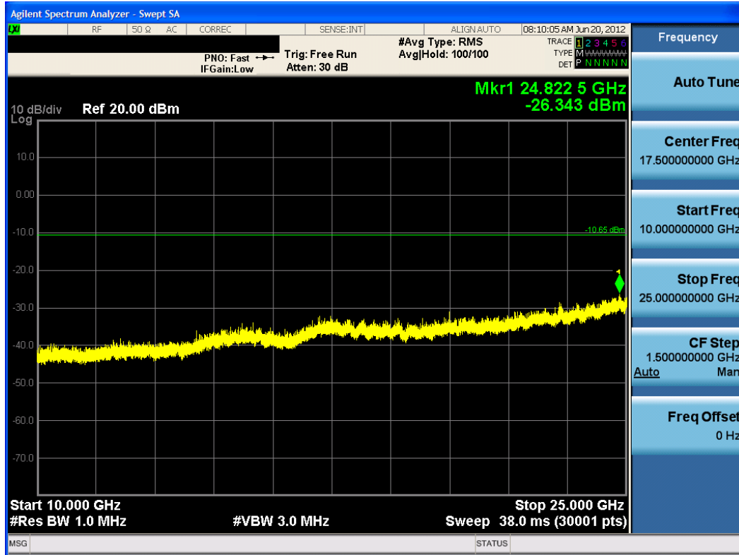
Plot 6-56. Conducted Spurious Plot (802.11b – Ch. 1)
