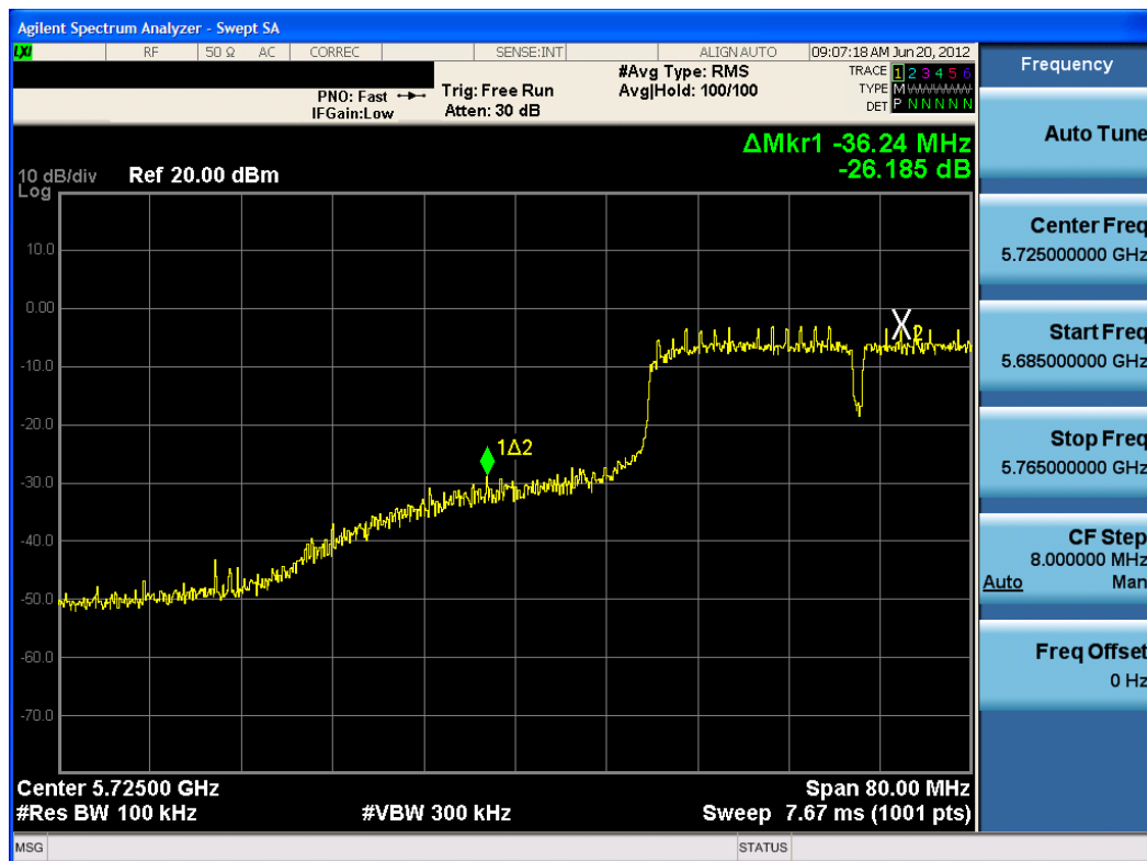
Plot 6-53. Band Edge Plot (40MHz BW 802.11n (5.8GHz) – Ch. 151)
