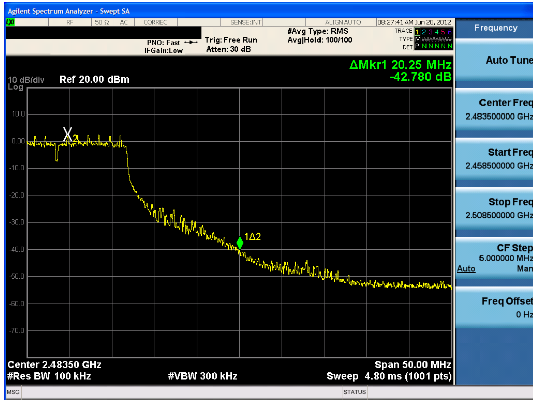
Plot 6-44. Band Edge Plot (802.11g – Ch. 11)
