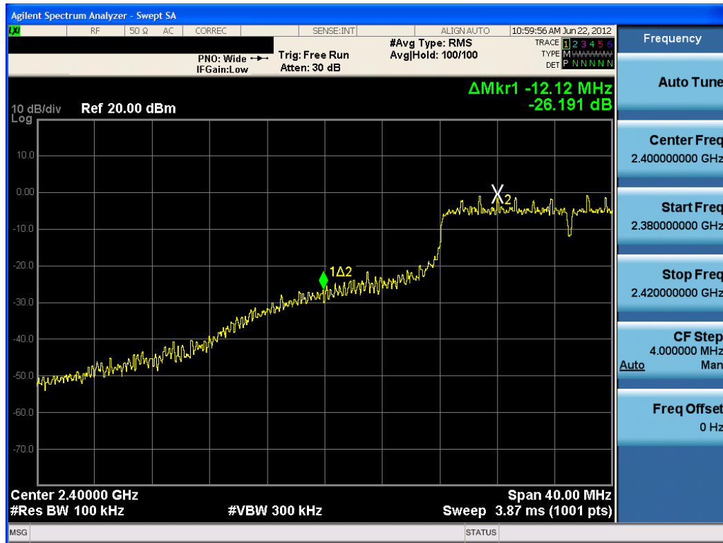
Plot 6-46. Band Edge Plot with Un-Reduced Power (802.11n (2.4GHz) – Ch. 2)
