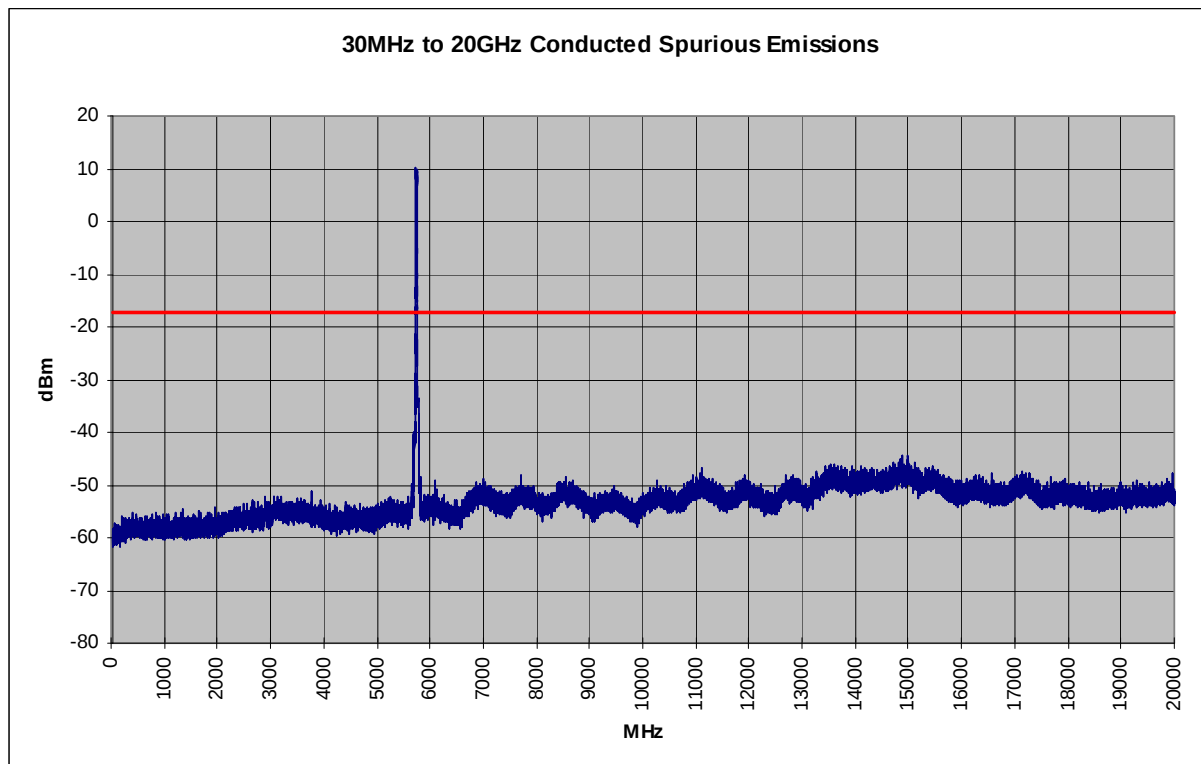
Plot 6-61. Conducted Spurious Plot (802.11a – Ch. 149)
