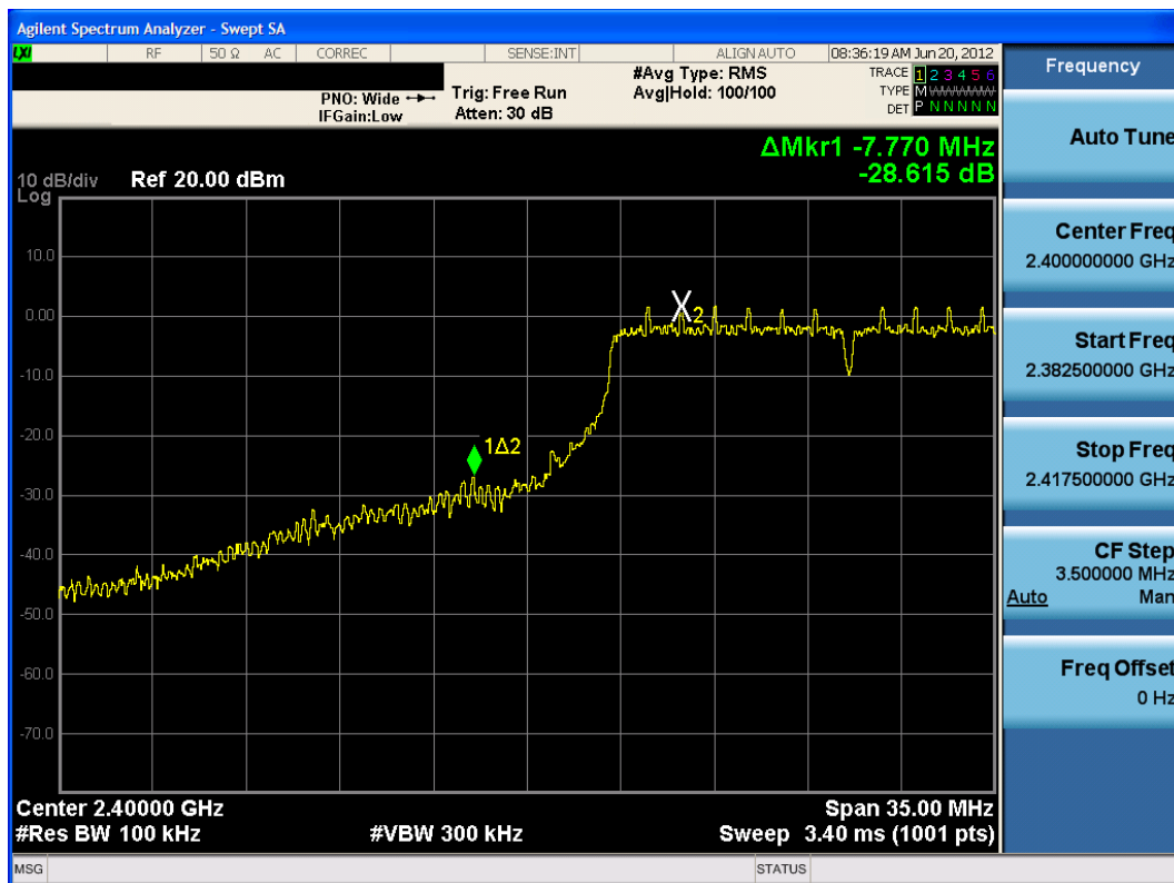
Plot 6-45. Band Edge Plot (802.11n (2.4GHz) – Ch. 1)
