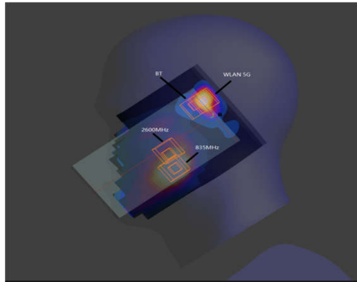
WWAN+ WLAN 5GHz+Bluetooth_Left Cheek 0mm
