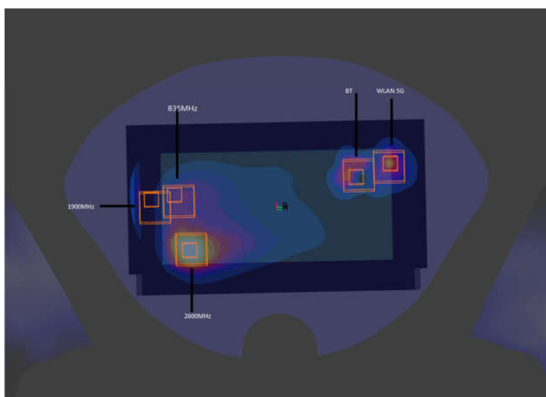
WWAN+ WLAN 5GHz+Bluetooth_Back 5mm
