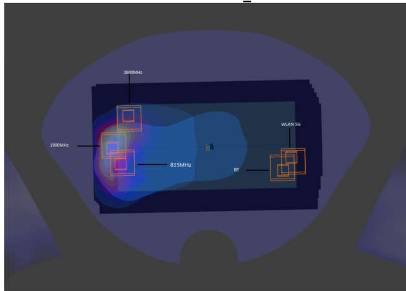
WWAN+ WLAN 5GHz+Bluetooth_Front 5mm
