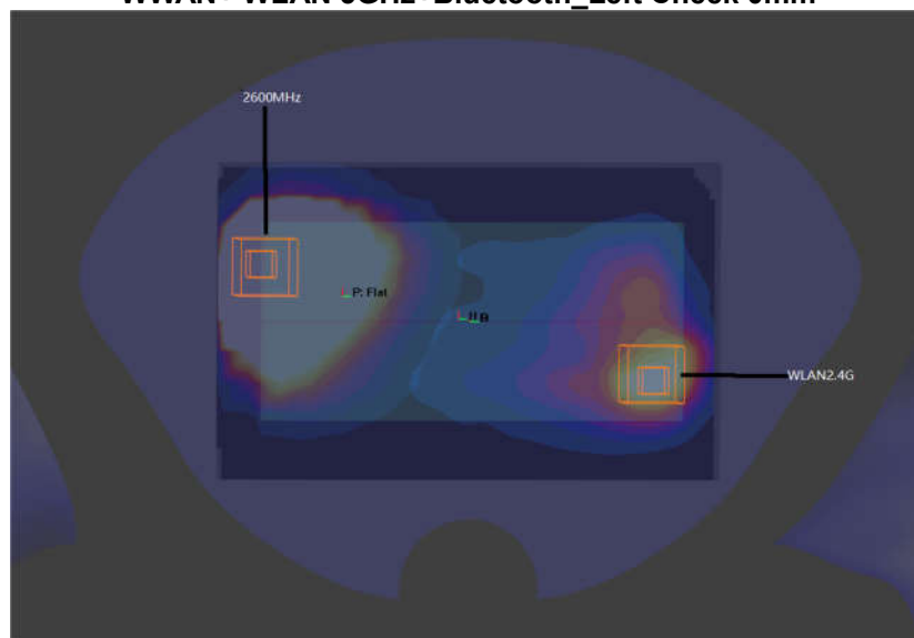
WWAN+ WLAN 2.4GHz_Front 5mm
