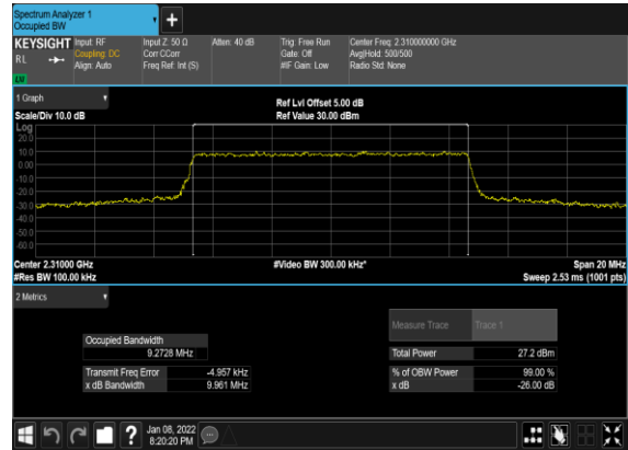
B2_N30(10M)_CP-OFDM_16 QAM_Outer_Full_Low_CH
