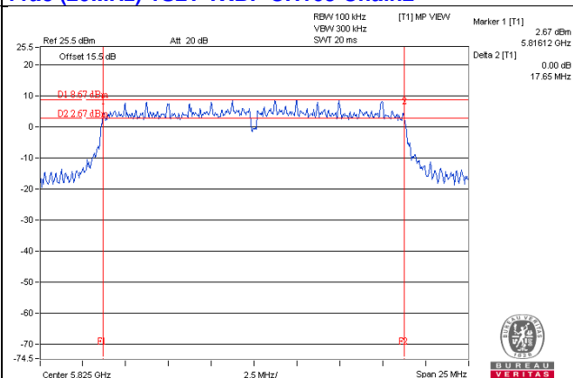
11ac (20MHz) 1S2T TXBF CH165 Chain2
