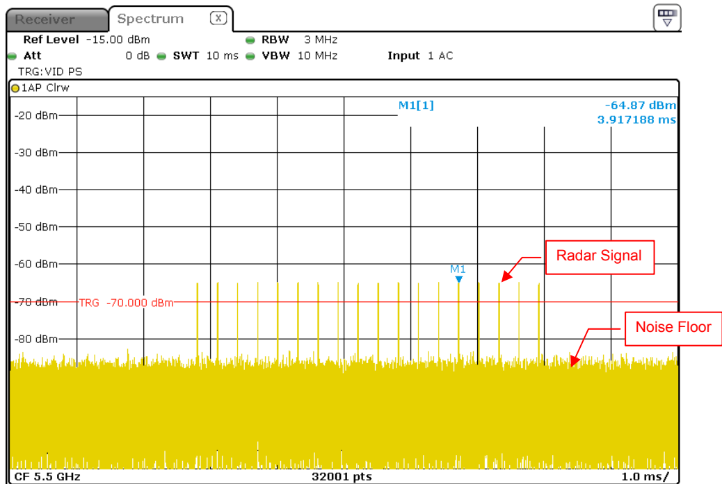
Radar Signal 3
