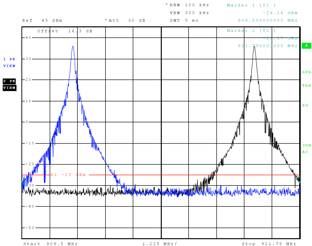
Figure 16 Emissions Mask eGo
