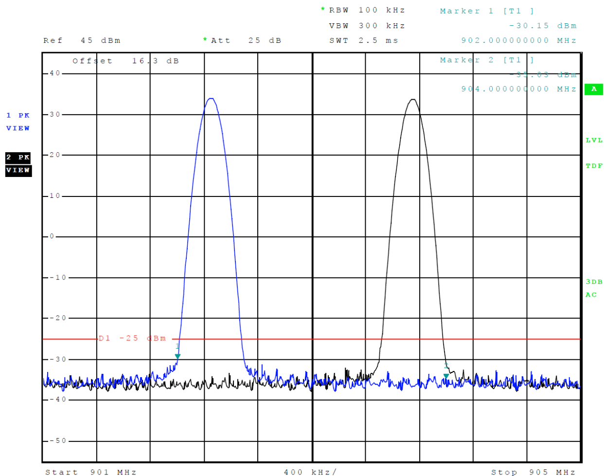
Figure 12 Emissions Mask ATA High Power (902-904 MHz Band)
