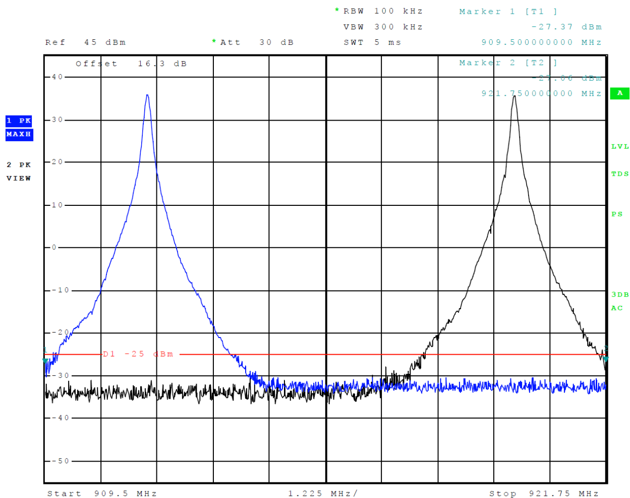
Figure 19 Emissions Mask EPC
