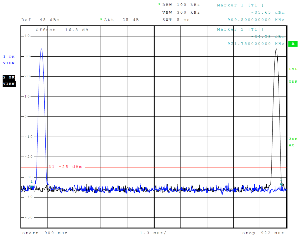
Figure 13 Emissions Mask ATA High Power (909.5-921.75 MHz Band)
