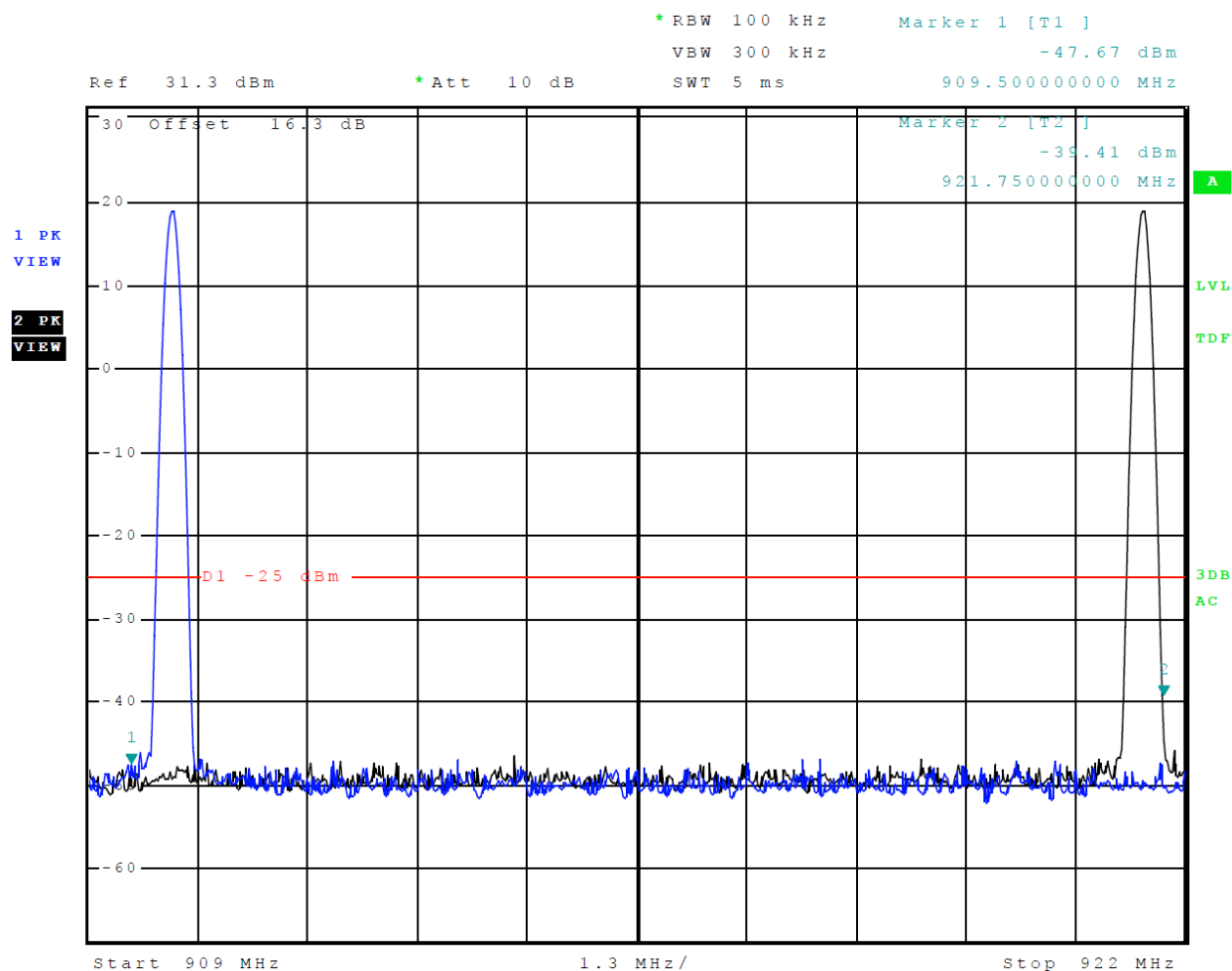
Figure 15 Emissions Mask ATA Low Power (909.5-921.75 MHz Band)
