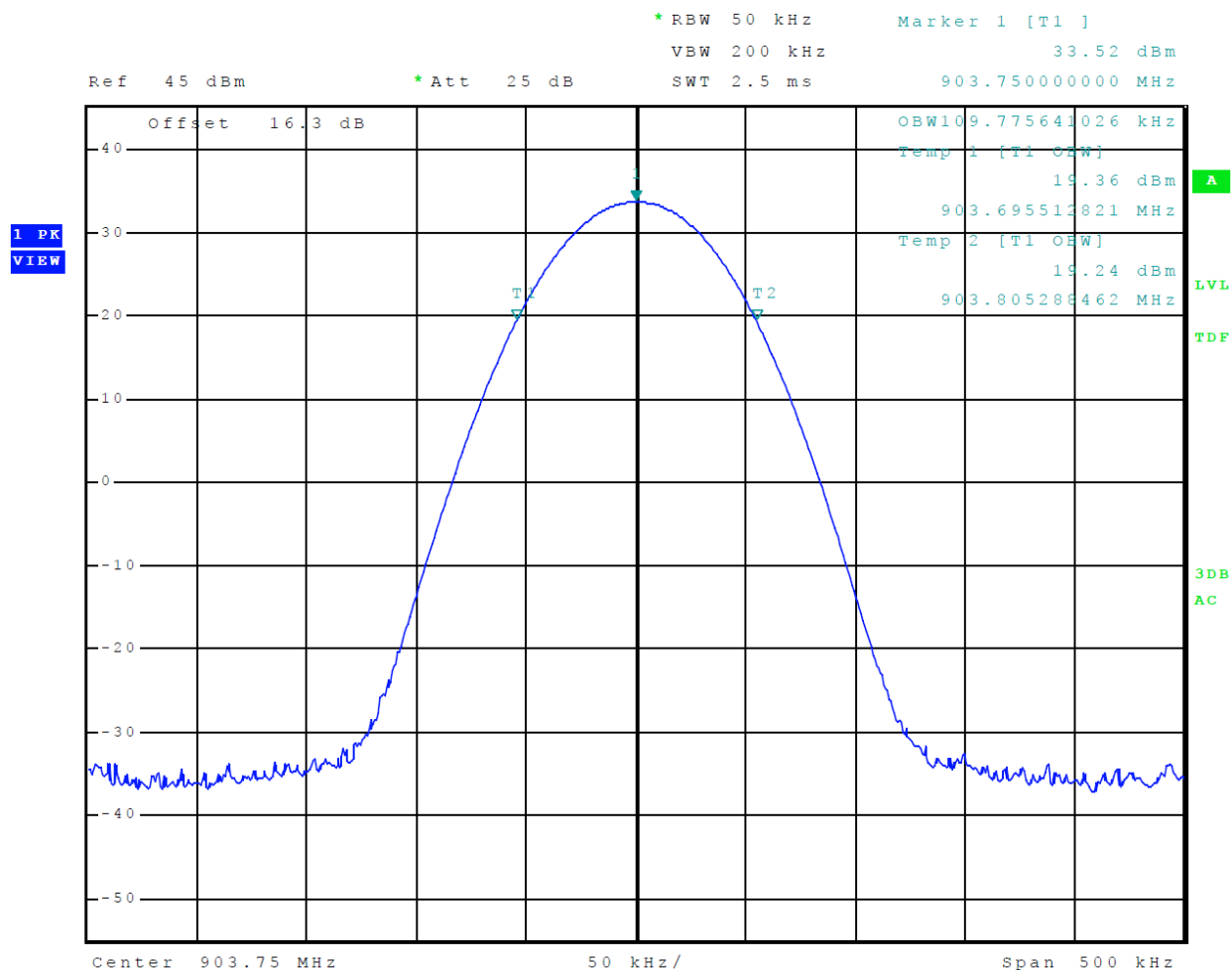
Figure 7 Occupied Bandwidth CW (ATA)
