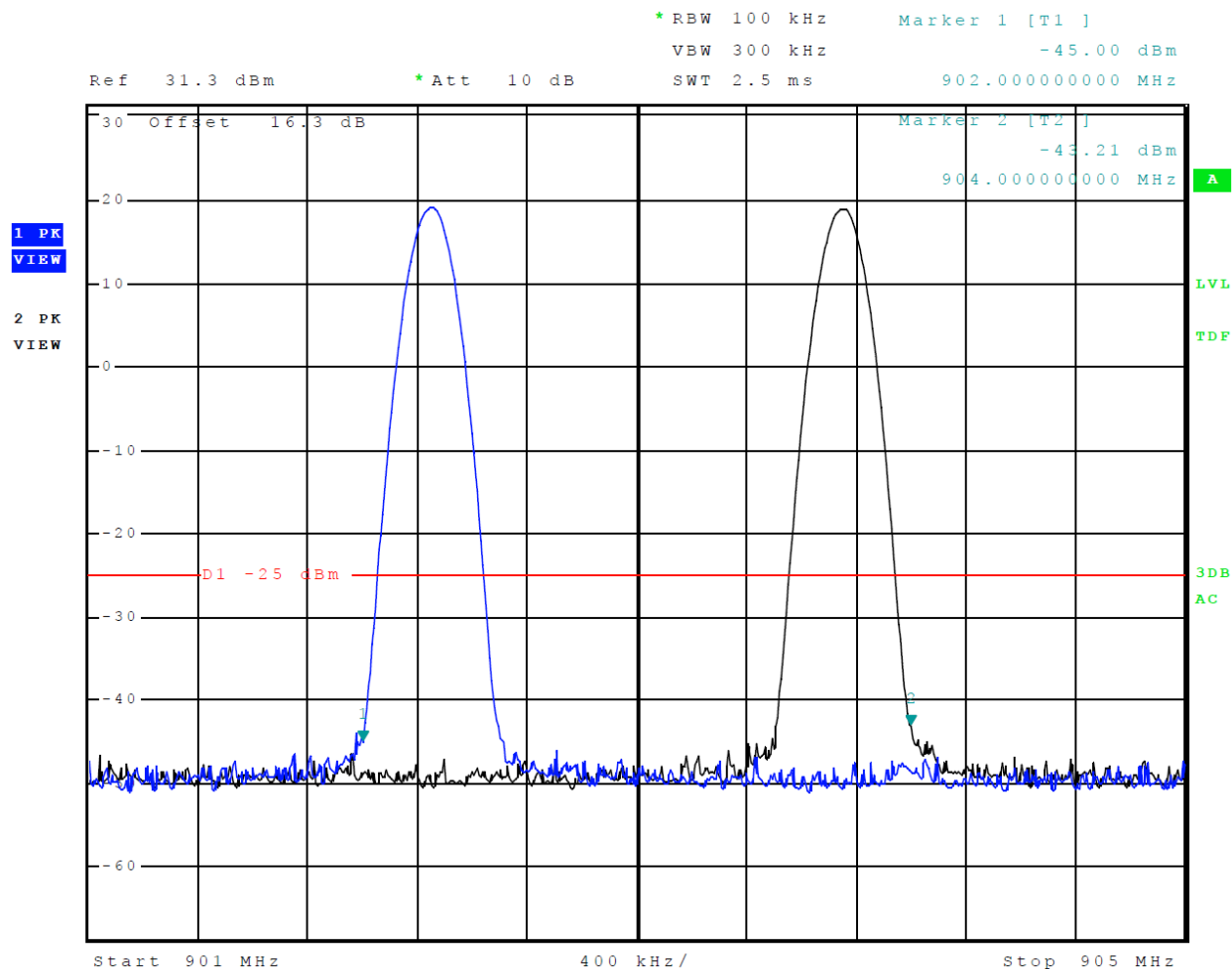
Figure 14 Emissions Mask ATA Low Power (902-904 MHz Band)
