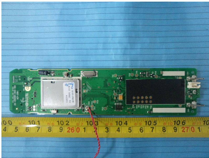
EUT – Main Board Top View (2# Handset)
