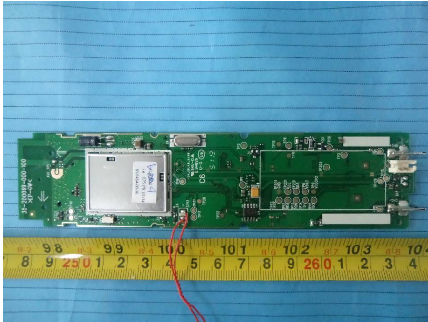
EUT – Main Board Top View (1# Handset)
