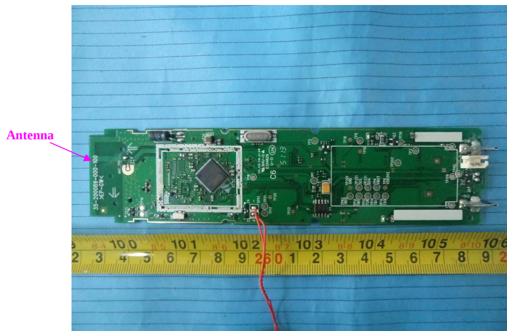
EUT – Main Board Top Shielding off View (1# Handset)
