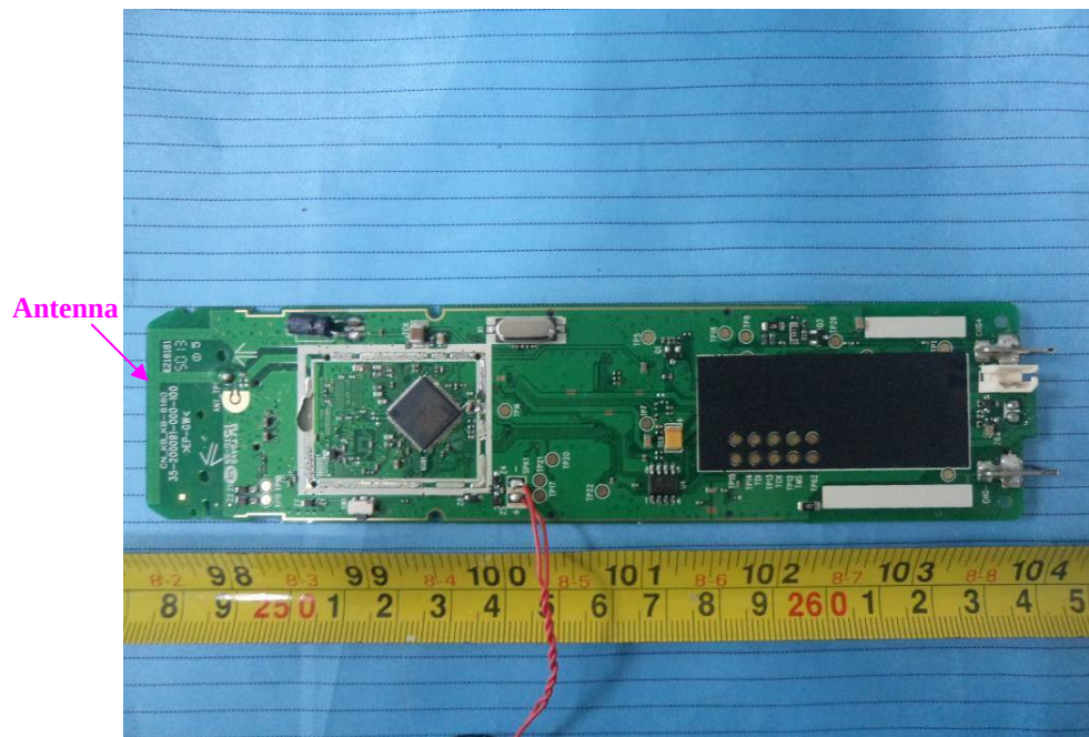
EUT – Main Board Top Shielding off View (2# Handset)
