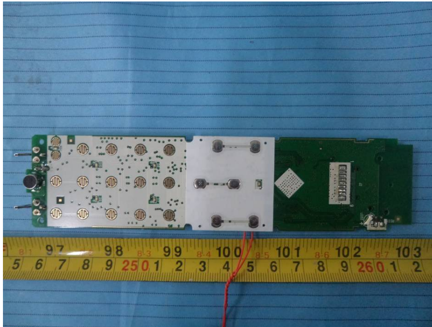
EUT – Main Board Bottom View (1# Handset)
